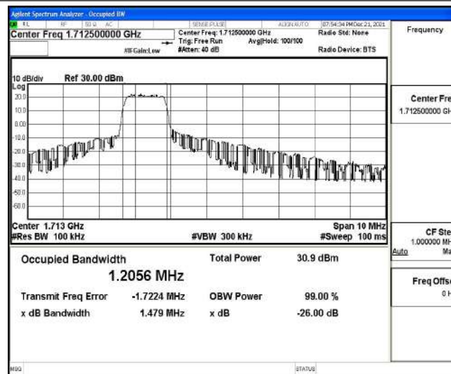
Band4-5MHz-QPSK-19975-6-0-Low-1.2056-1.479-PASS
