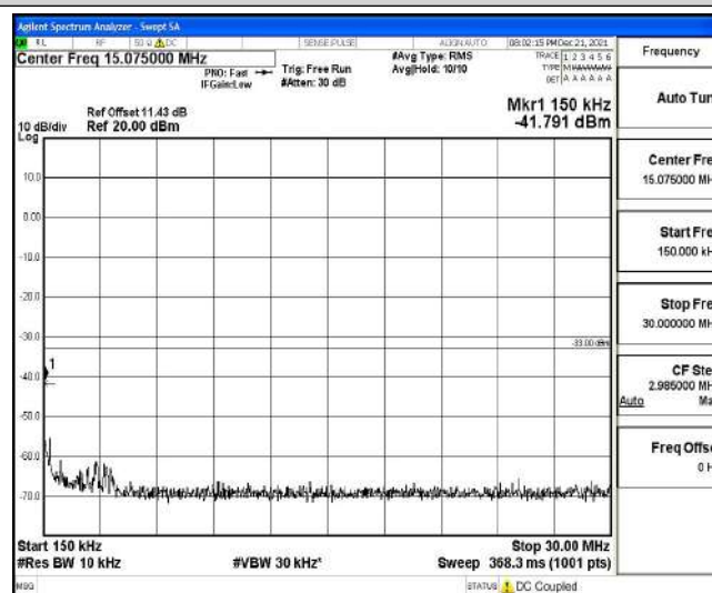
Band4-5MHz-16QAM-20175-1-0-Low-0.15-30--41.79-PASS
