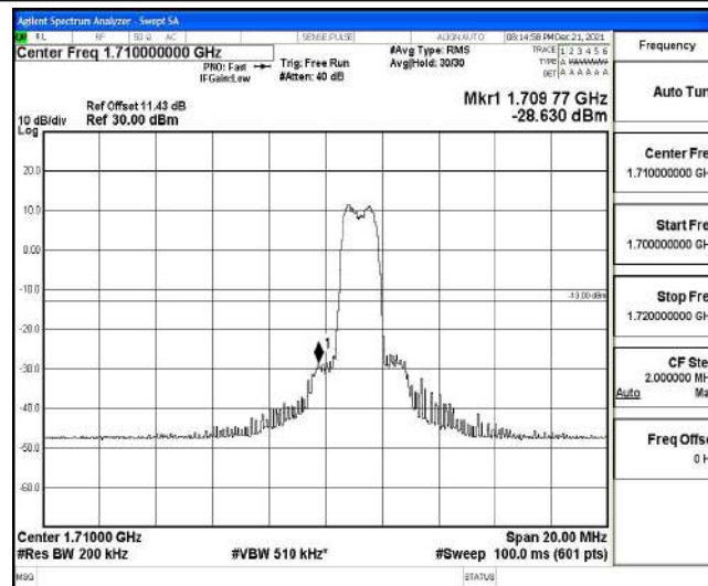
Band4-10MHz-16QAM-20000-6-0-Low--28.63-PASS
