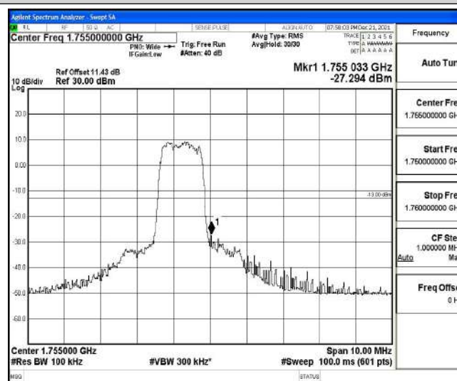
Band4-5MHz-QPSK-20375-6-0-High--27.29-PASS
