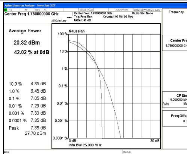
Band4-10MHz-QPSK-20350-6-0-High-7.05-&lt;=13-PASS
