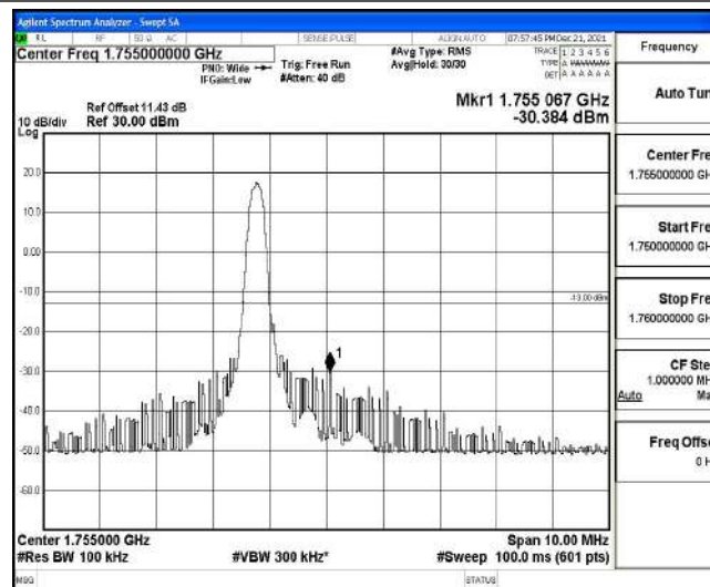
Band4-5MHz-QPSK-20375-1-0-High--30.38-PASS
