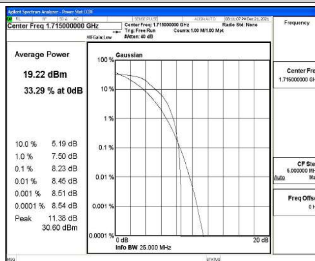
Band4-10MHz-16QAM-20000-6-0-Low-8.23-&lt;=13-PASS
