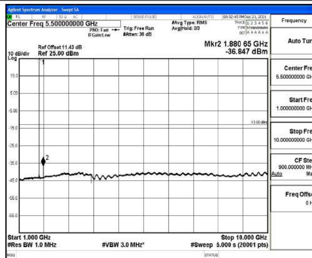
Band4-5MHz-16QAM-20175-1-0-Low-1000-10000--36.85-PASS
