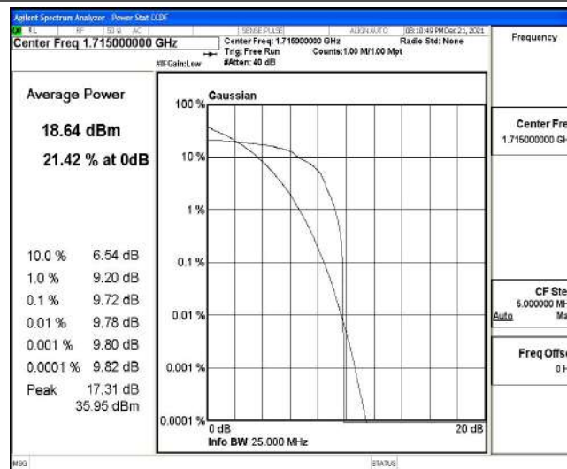
Band4-10MHz-16QAM-20000-1-0-Low-9.72-&lt;=13-PASS
