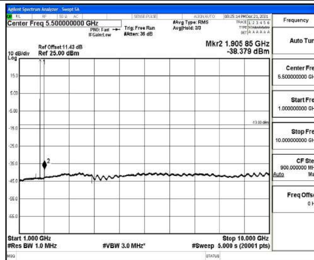
Band4-10MHz-16QAM-20350-1-0-High-1000-10000--38.38-PASS
