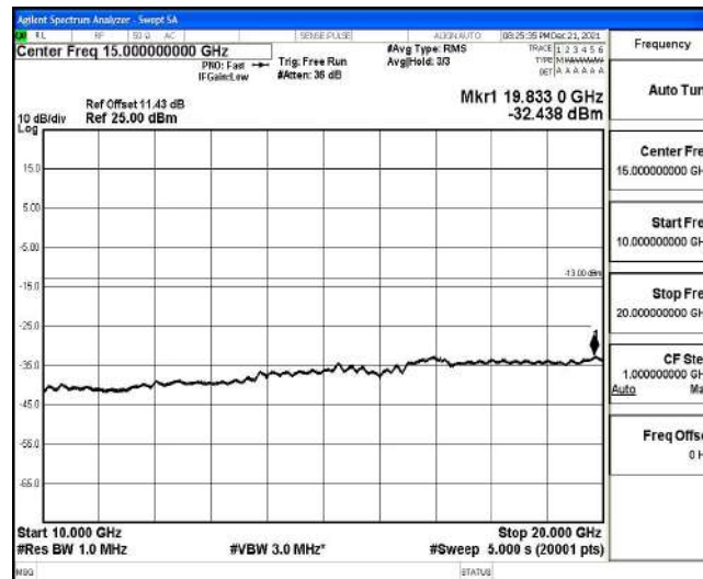
Band4-10MHz-16QAM-20350-1-0-High-10000-20000--32.44-PASS
