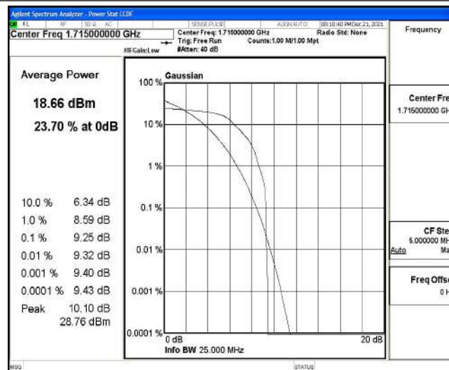
Band4-10MHz-QPSK-20000-1-0-Low-9.25-&lt;=13-PASS
