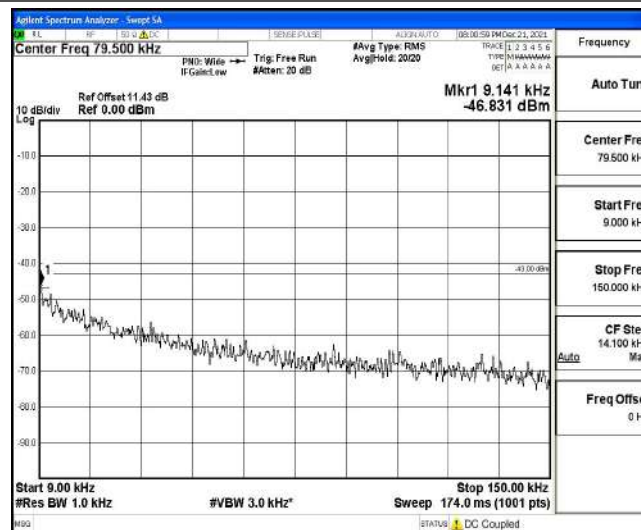
Band4-5MHz-QPSK-20175-1-0-Low-0.15--46.83-PASS
