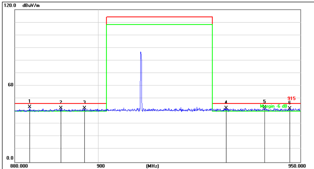
915 MHz Horizontal
