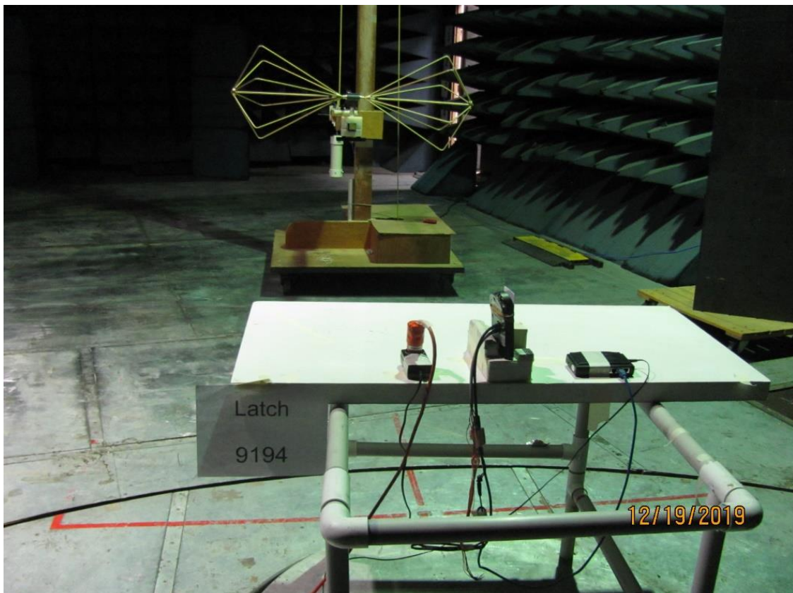
Biconical Antenna
