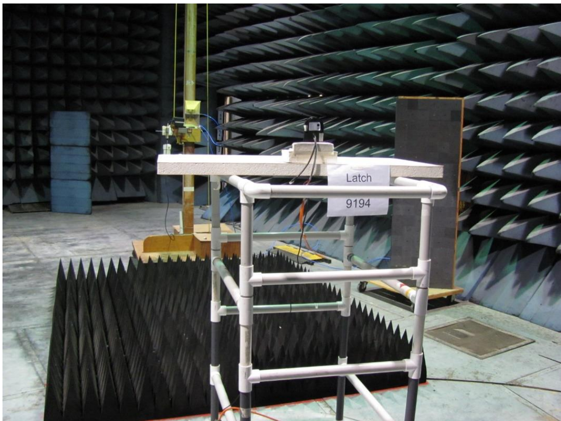
Horn Antenna above 1 GHz
