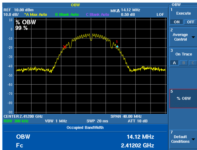
8011.b, Channel 1
