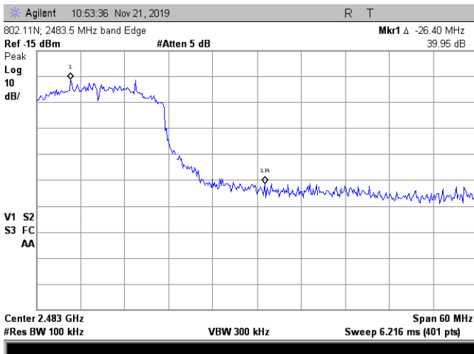
802.11N, Channel 11
