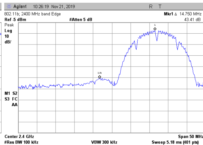
802.11b, Cannel 1
