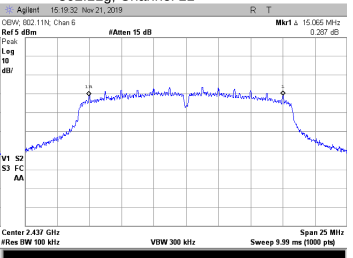
802.11n, Channel 6
