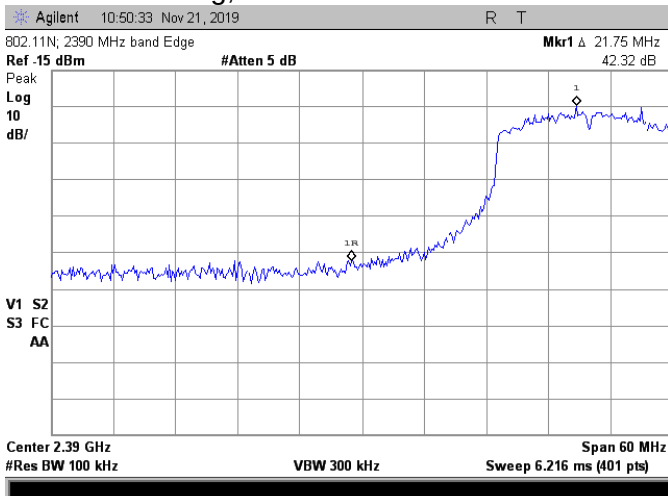
802.11N, Channel 1
