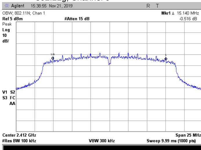
802.11n, Channel 1
