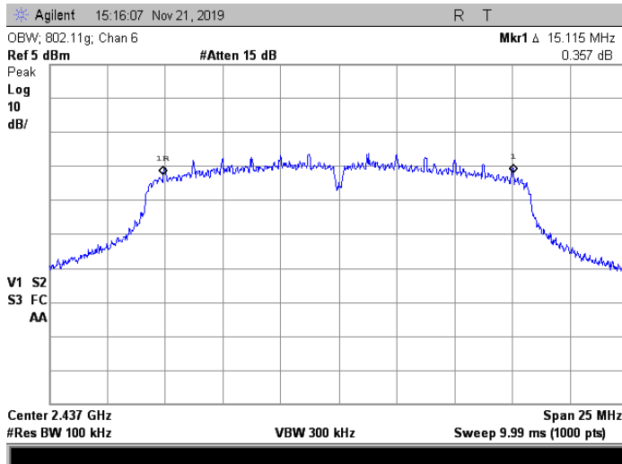
802.11g, Channel 6
