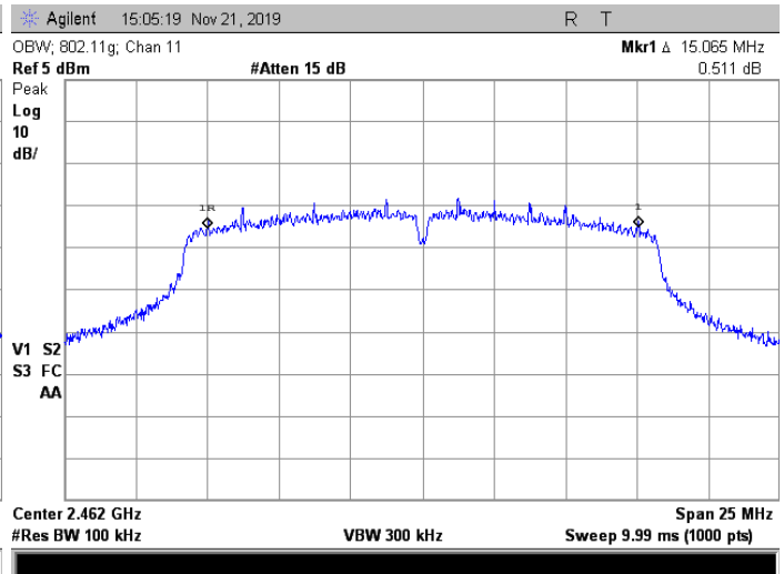
802.11g, Channel 11
