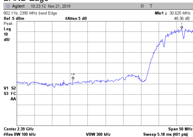
802.11b, Channel 1
