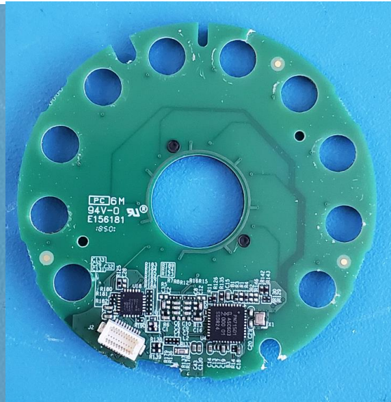
Lens front PCB bottom
