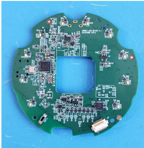
Lens rear PCB top
