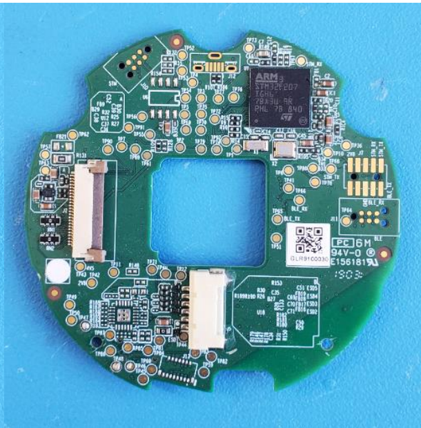
Lens rear PCB bottom
