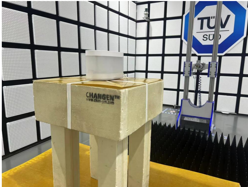
RSE 18-40GHz
