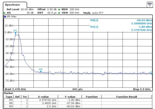
CH39-Bandedge
