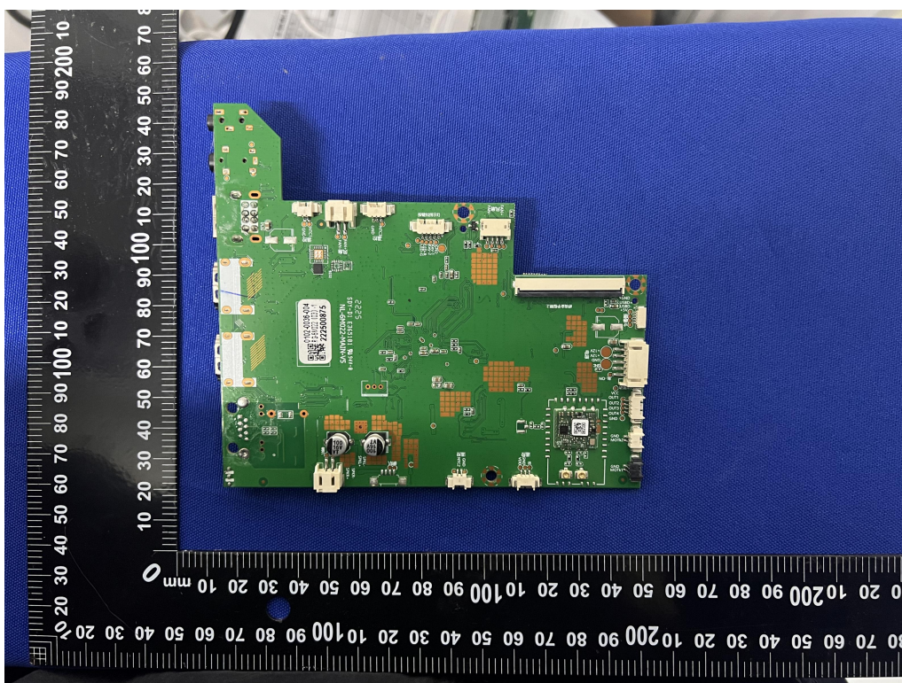
Photo 14 Main board
