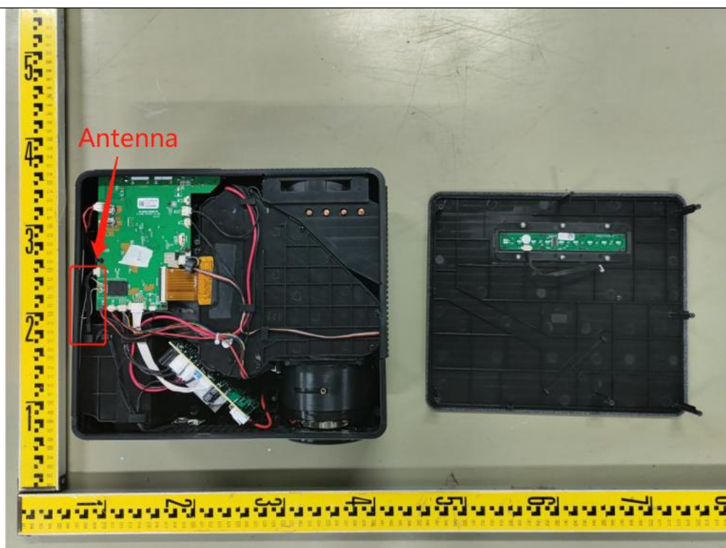
Photo 17 Antenna location
