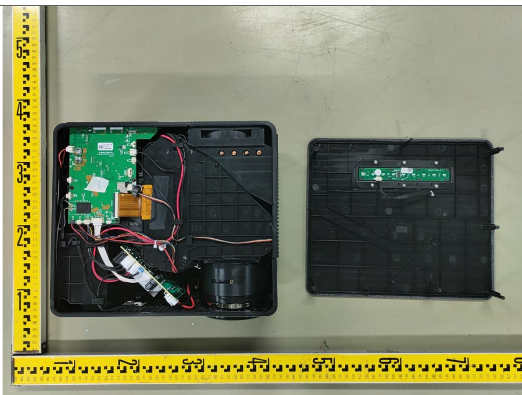
Photo 5 Internal view
