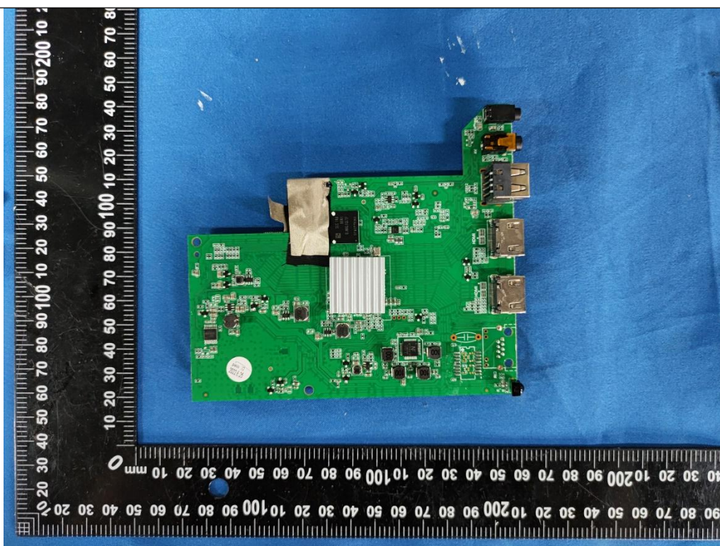
Photo 13 Main board
