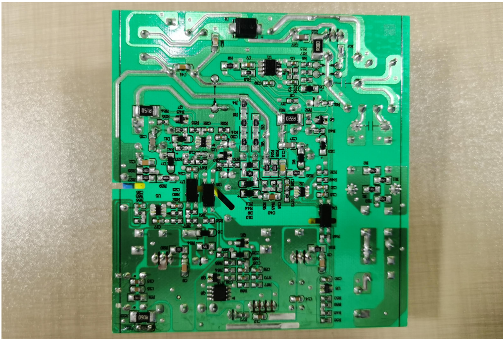
Photo 10 Power supply board
