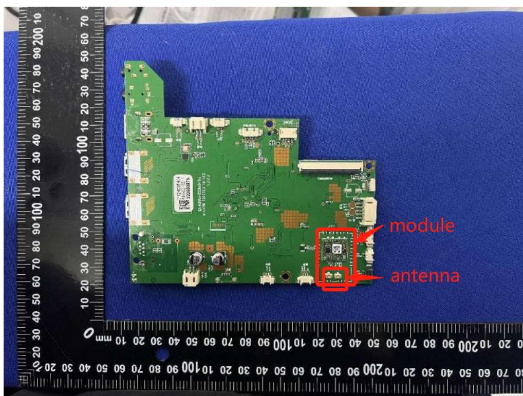
Photo 18 Antenna location
