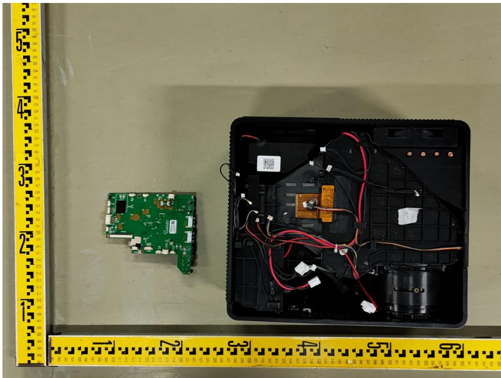
Photo 7 Internal view
