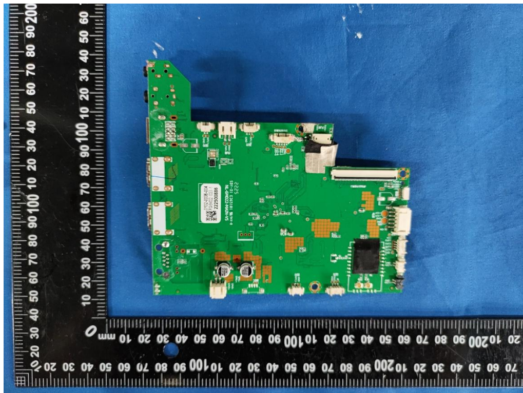
Photo 12 Main board
