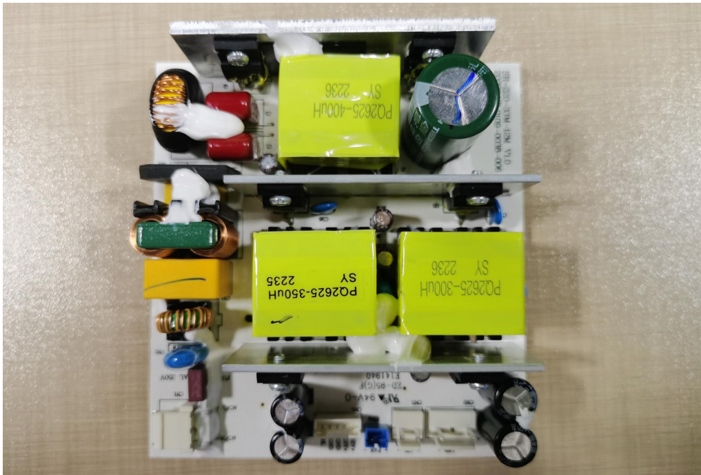
Photo 9 Power supply board
