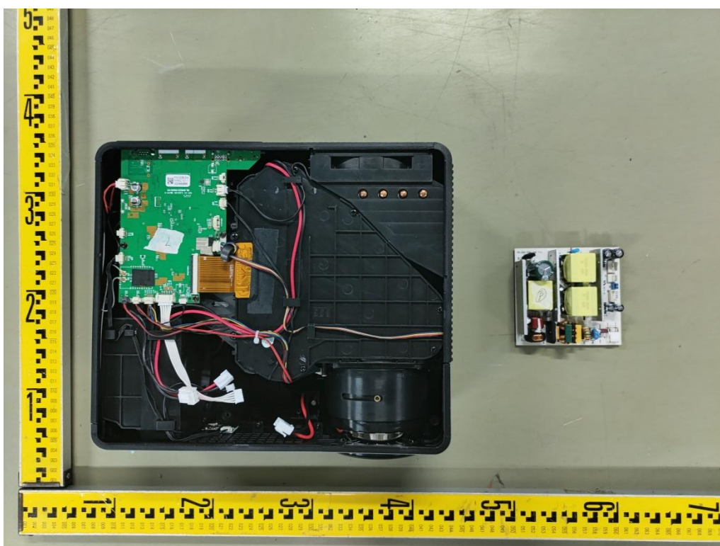
Photo 6 Internal view
