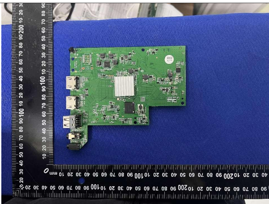
Photo 15 Main board
