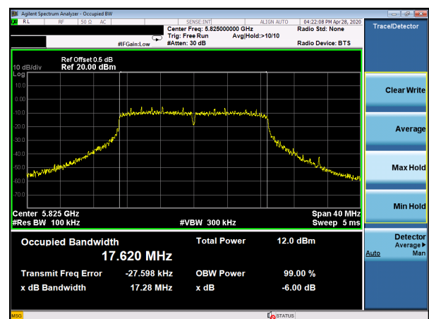
(802.11 n20) 6dB&99%Bandwidth plot on channel 165
