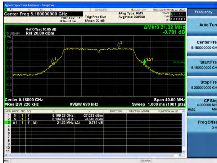
11A_Ant2_5180
