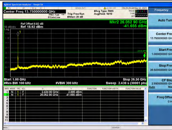
11G_Ant2_2437_0~Reference
