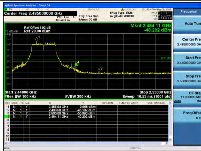
11G_Ant2_High_2462
