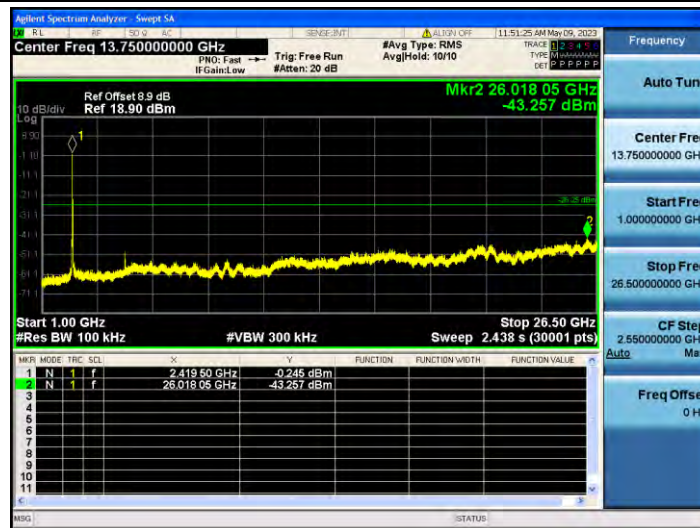
11G_Ant2_2412_0-Reference
