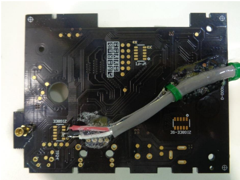
Photo 6: – Bottom View of the Antenna – Conducted Measurements
