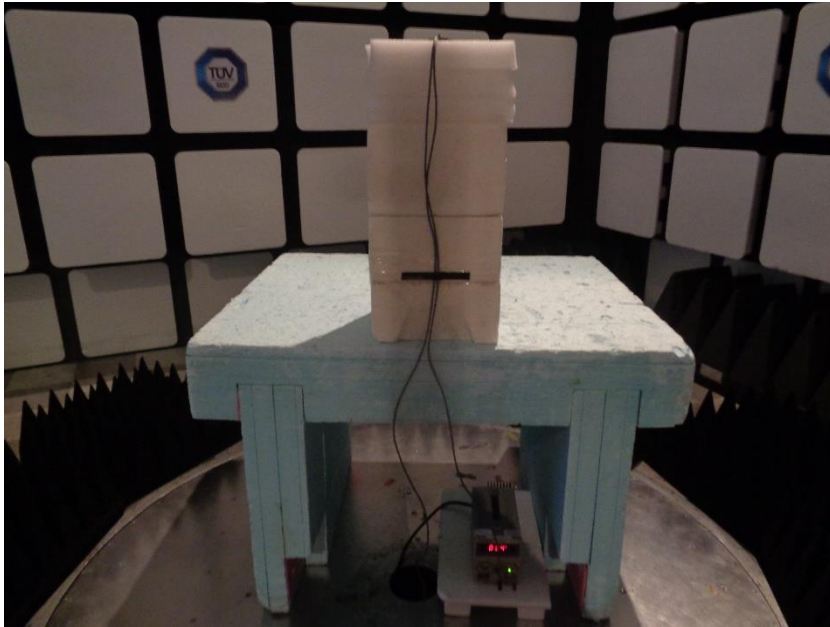
Photo 4: – Setup of Radiated Spurious Emissions > 1GHz
