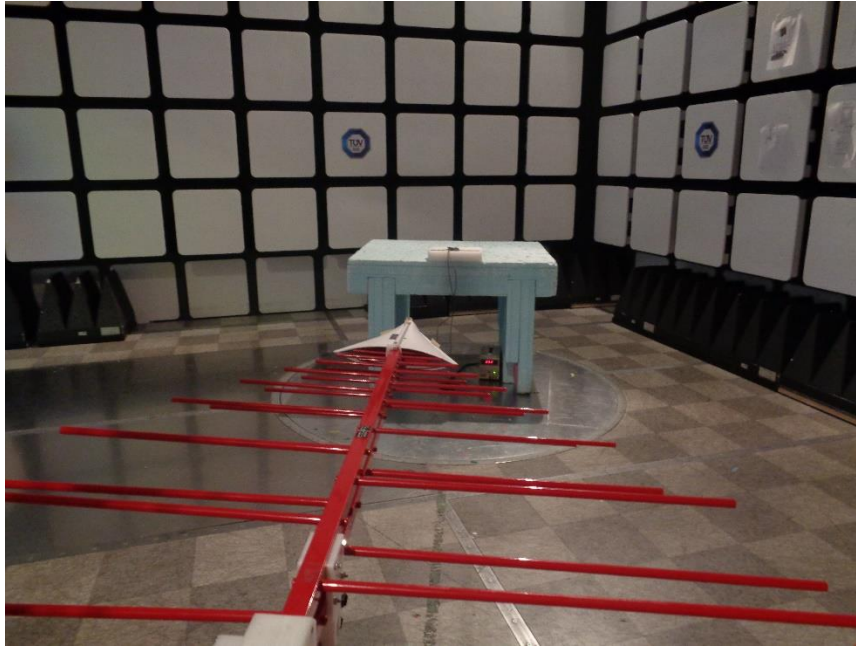
Photo 2: – Radiated Spurious Emissions – Horizontal Polarization <1GHz
