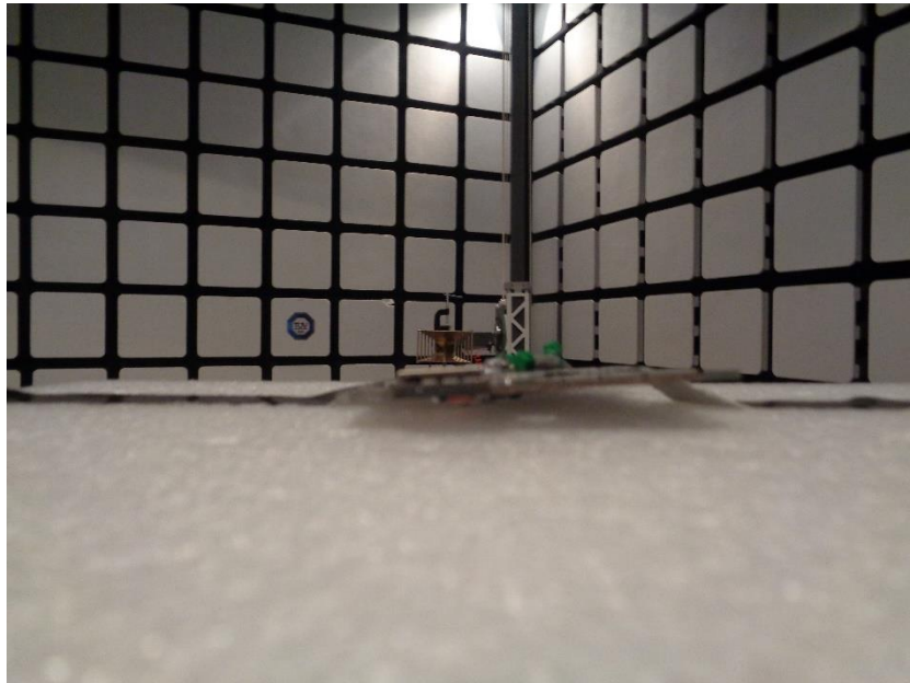
Photo 5: – Table Closeup of Radiated Spurious Emissions > 1GHz
