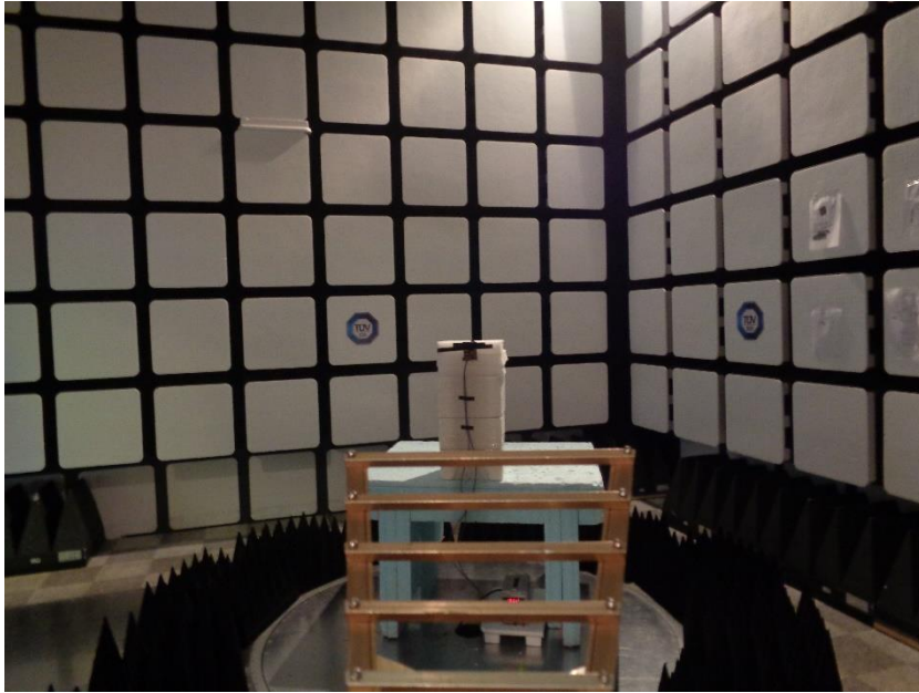
Photo 6: – Radiated Spurious Emissions – Horizontal Polarization >1GHz
