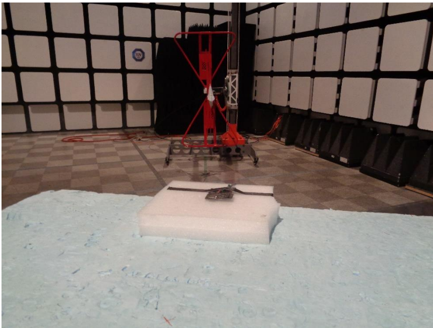
Photo 3: – Radiated Spurious Emissions – Vertical Polarization <1GHz
