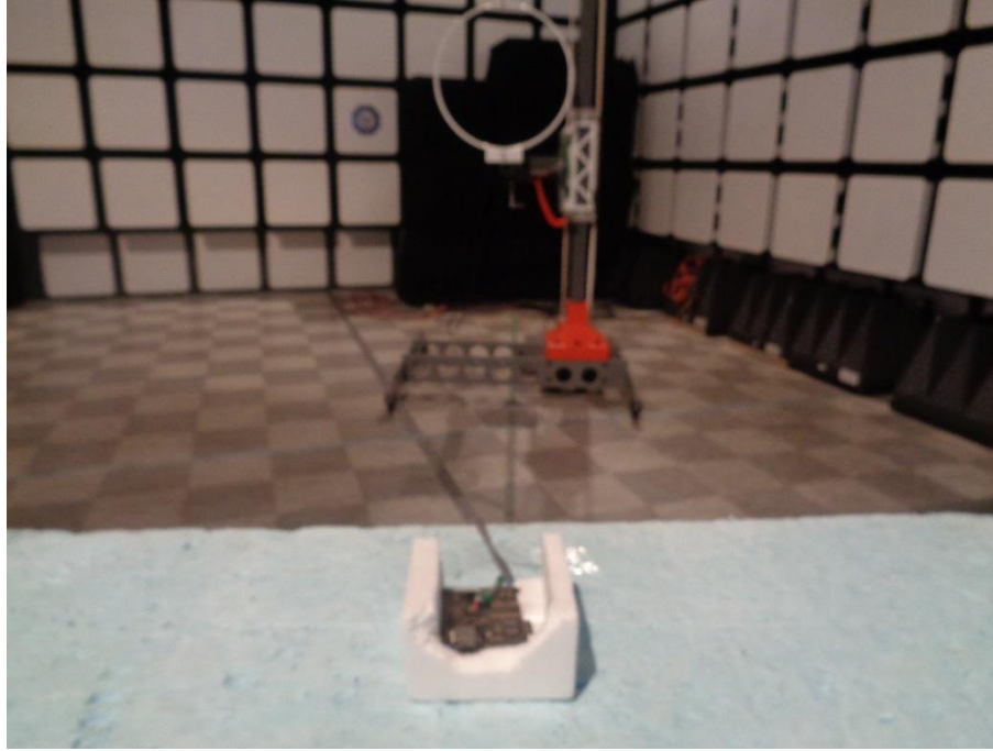
Photo 1: –Test Setup – 15kHz to 30MHz z
