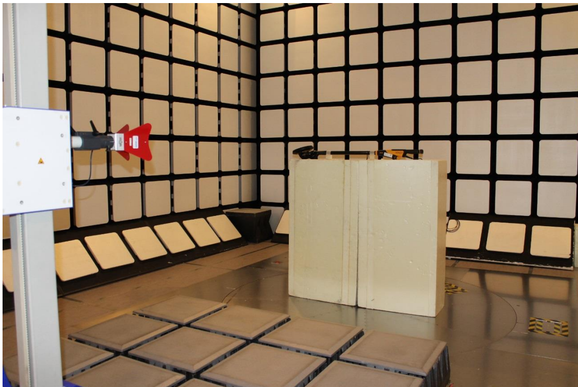
Photograph 5. Radiated emission test setup (1 to 18 GHz)
