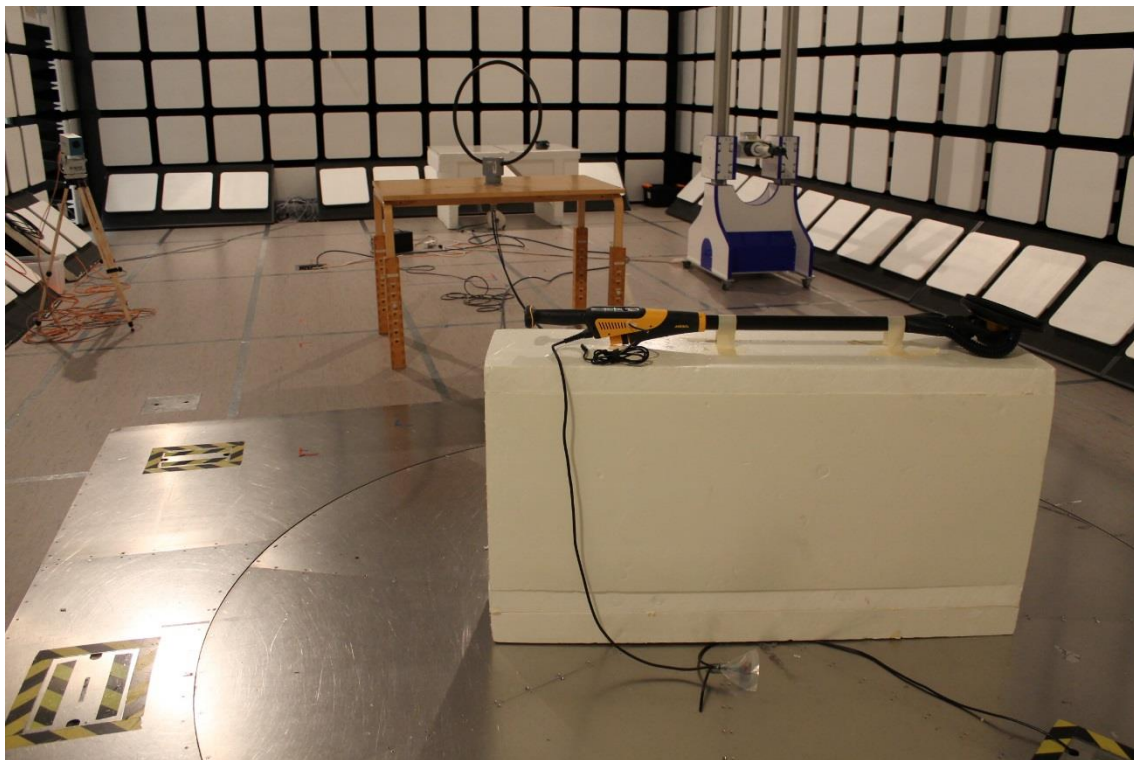
Photograph 3. Radiated emission test setup (9 kHz to 30 MHz)
