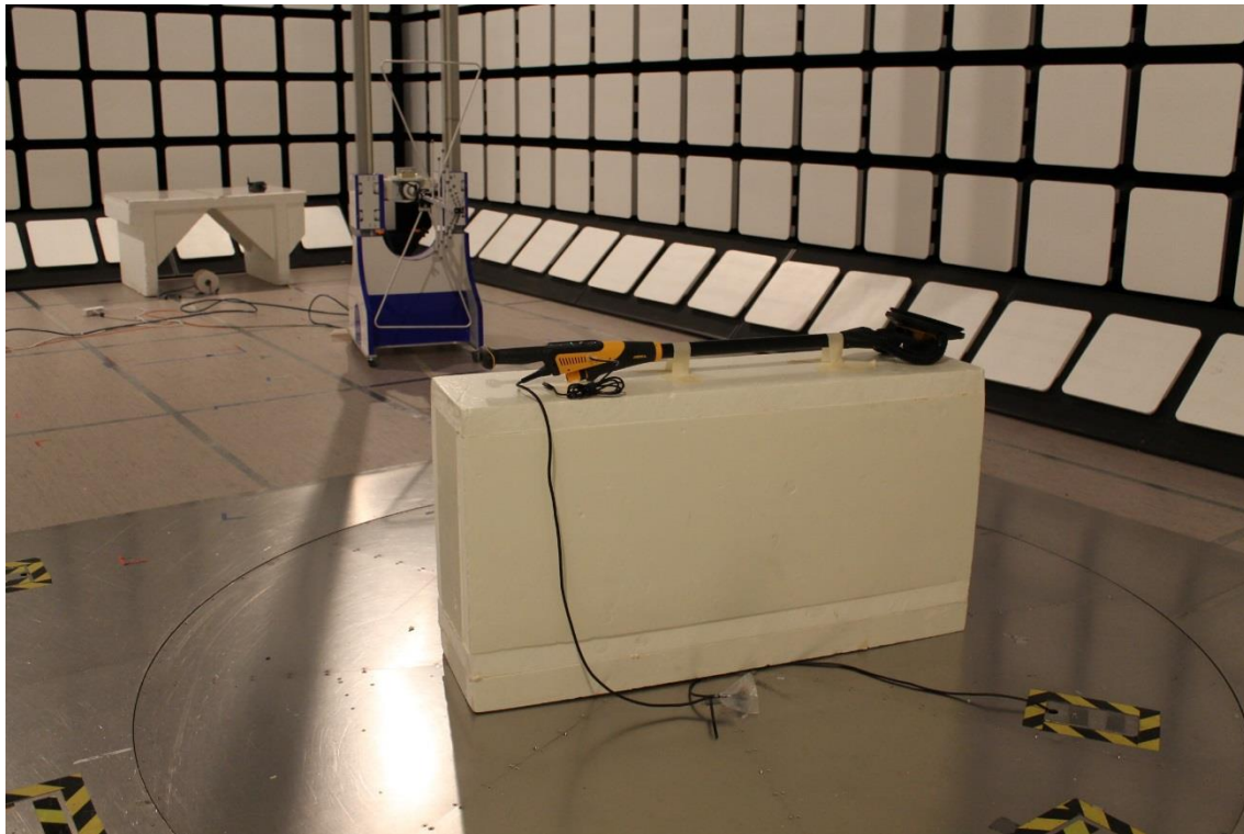
Photograph 4. Radiated emission test setup (30 MHz to 1000 MHz)
