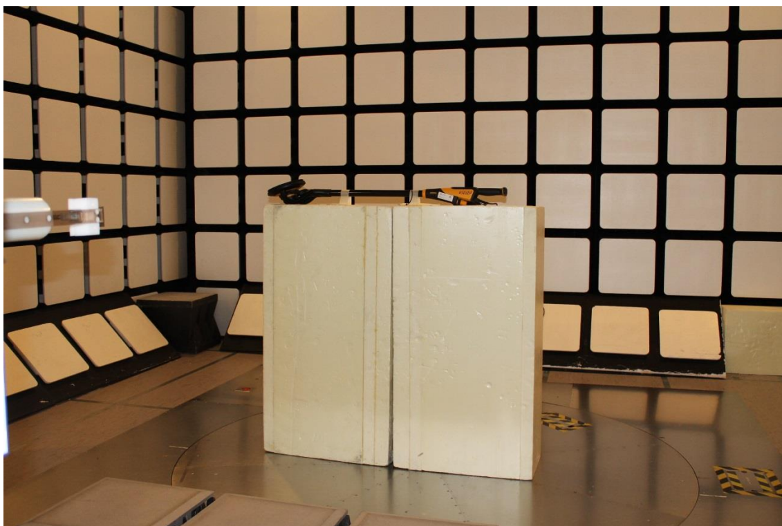
Photograph 6. Radiated emission test setup (18 to 26.5 GHz)
