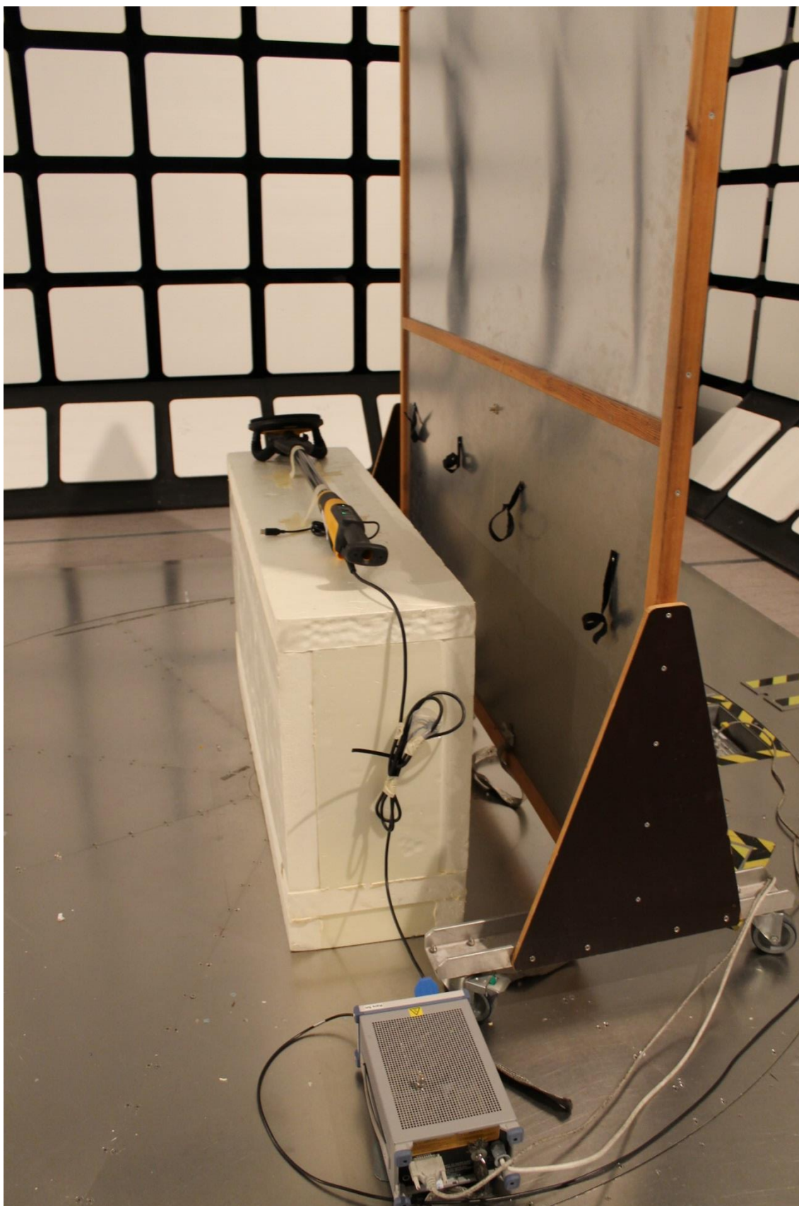
Photograph 7. Conducted emission test setup.
