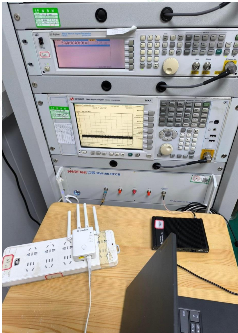
DFS
