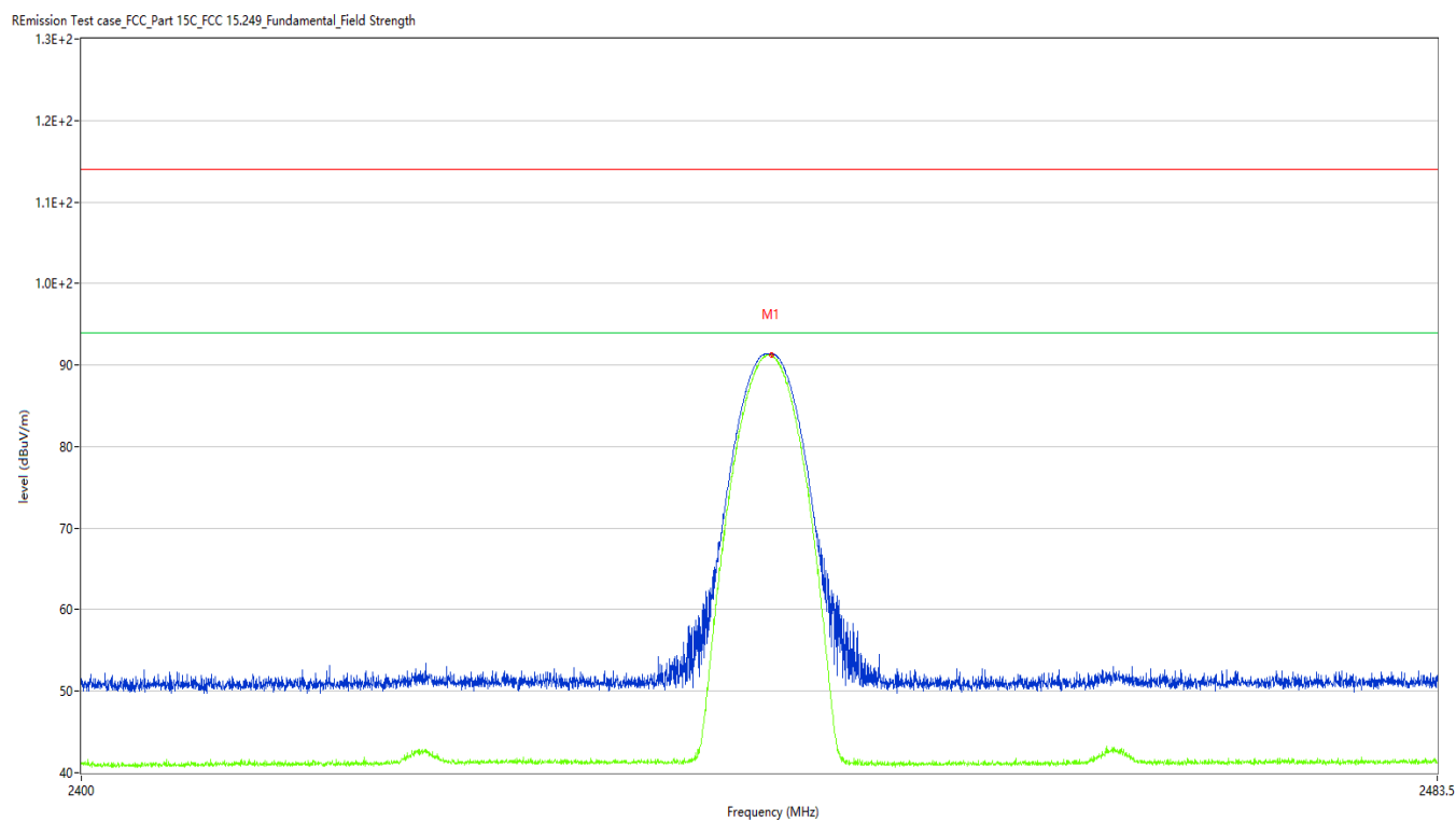
Figure 3: Test plots of Field strength of fundamental, 2442MHz, Horizontal polarization
