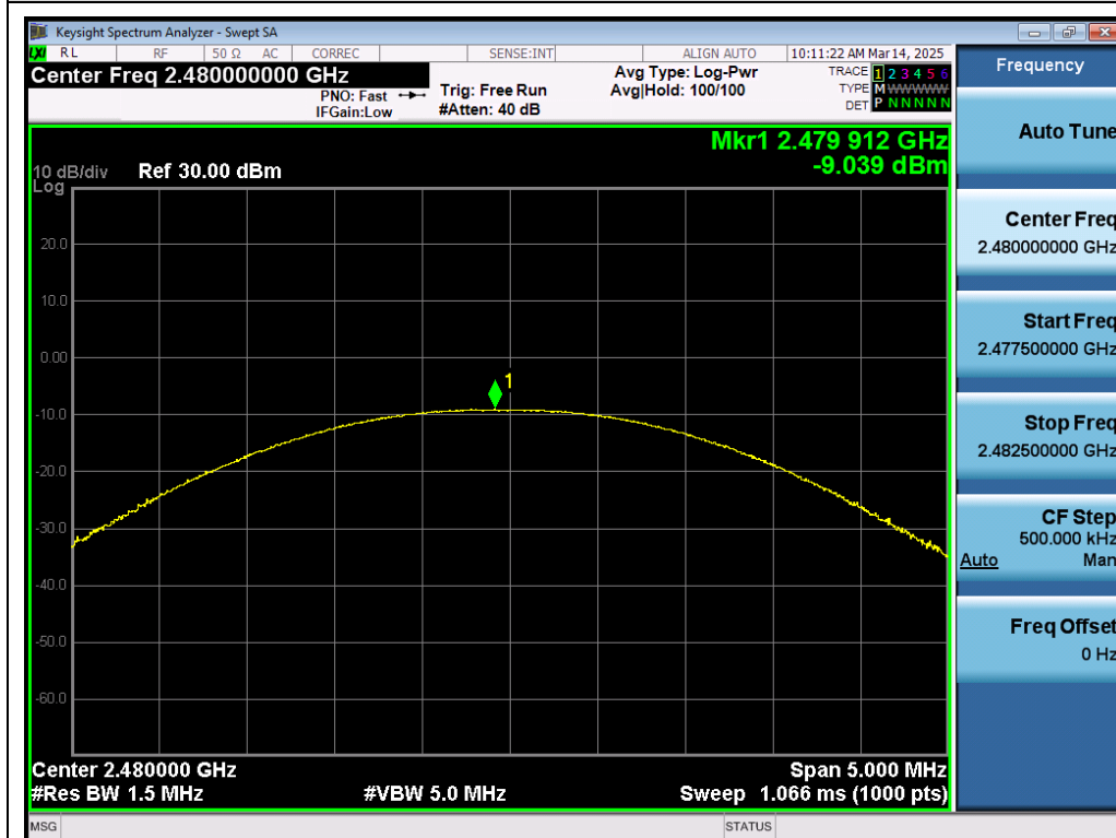
Test_Graph_EDR_ANT1_2480_2Mbps_Peak Power
