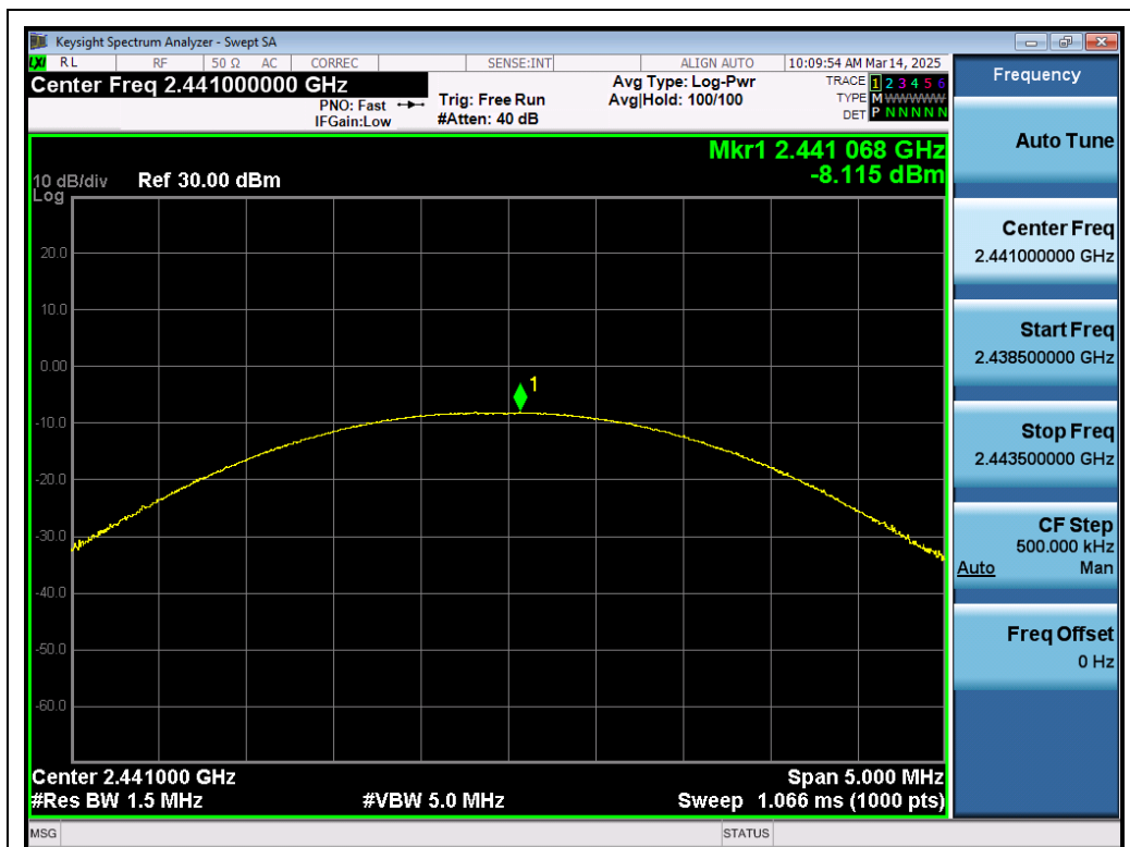
Test_Graph_EDR_ANT1_2441_2Mbps_Peak Power
