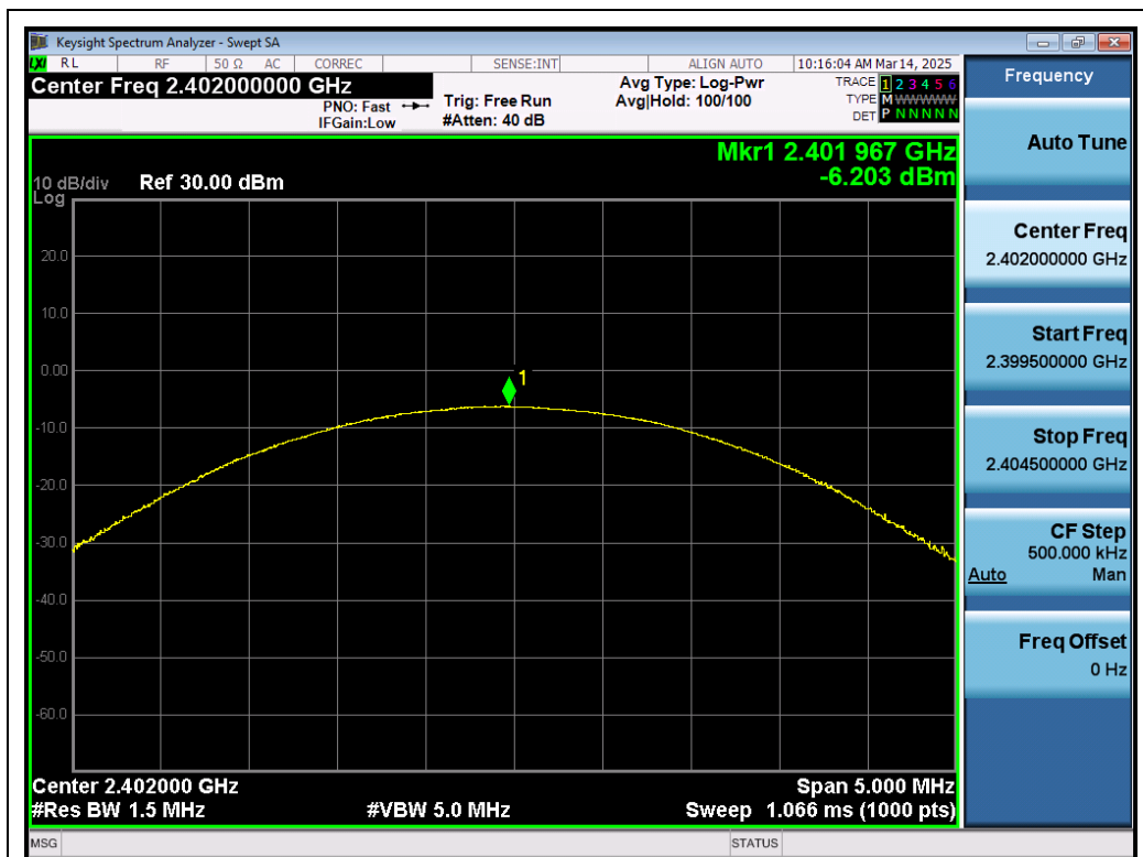
Test_Graph_EDR_ANT1_2402_3Mbps_Peak Power
