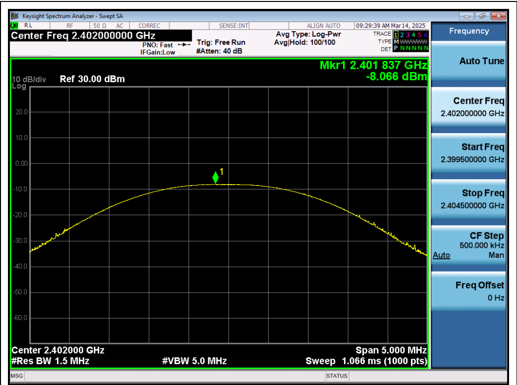
Test_Graph_BR_ANT1_2402_1Mbps_Peak Power
