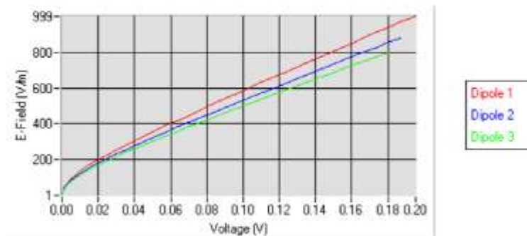
Calibration curves
