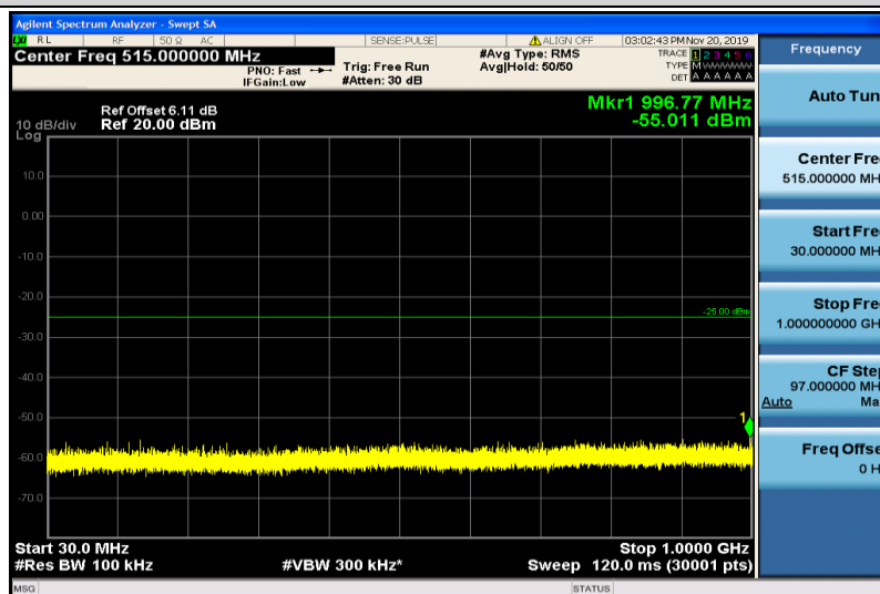
Band41-20MHz-QPSK-39750-1RB#0-30~1000MHz
