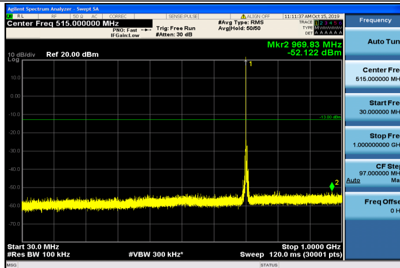
Band17-5MHz-16QAM-23790-1RB#0-30~1000MHz
