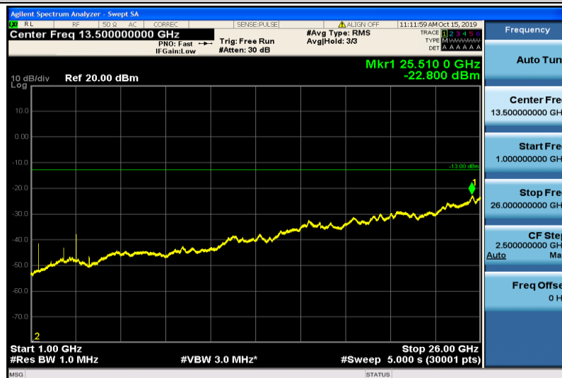
Band17-5MHz-16QAM-23790-1RB#0-1000~26000MHz
