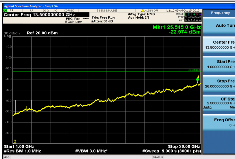
Band17-5MHz-16QAM-23755-1RB#0-1000~26000MHz
