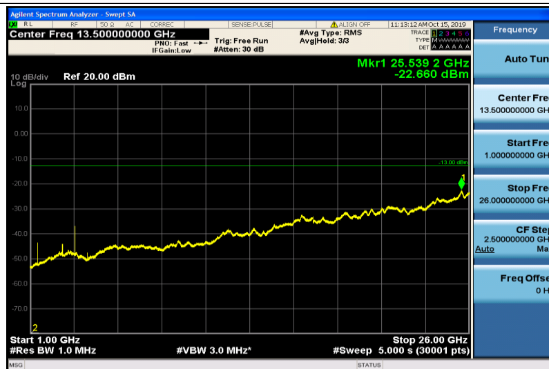
Band17-5MHz-16QAM-23825-1RB#0-1000~26000MHz
