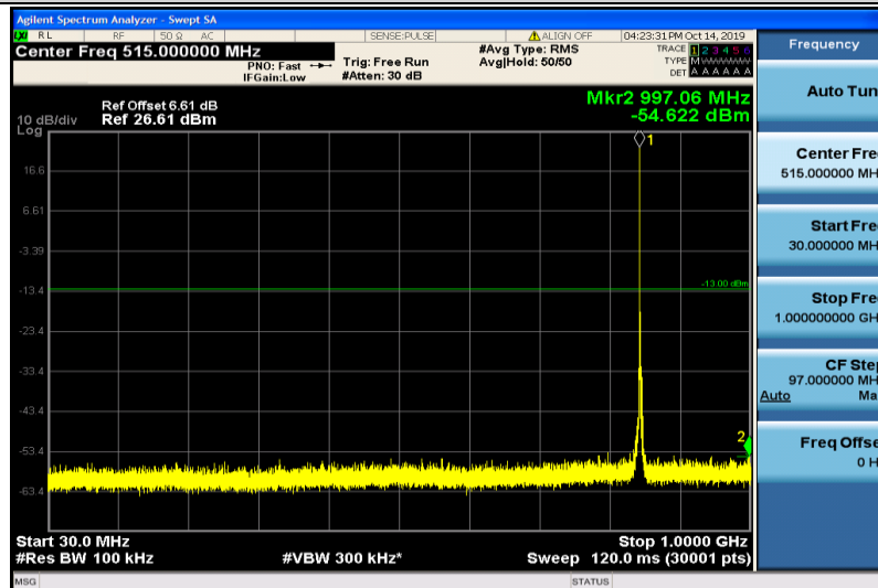
Band5-3MHz-16QAM-20635-1RB#0-30~1000MHz
