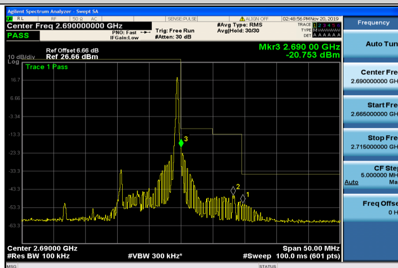
Band41-10MHz-16QAM-41540-1RB#49
