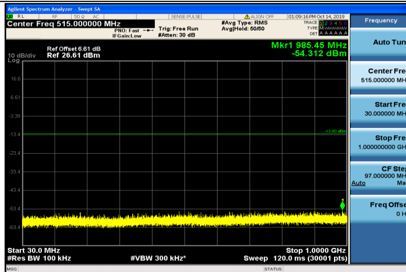
Band2-10MHz-16QAM-19150-1RB#0-30~1000MHz
