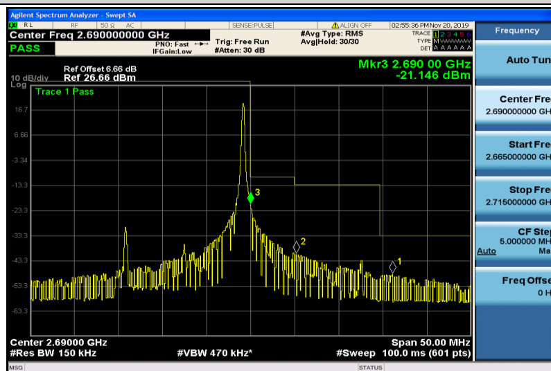
Band41-15MHz-16QAM-41515-1RB#74
