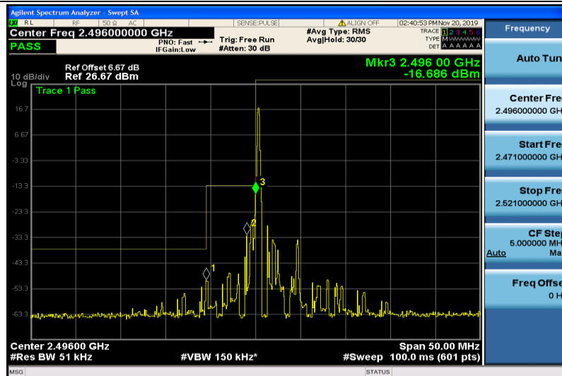
Band41-5MHz-QPSK-39675-1RB#0
