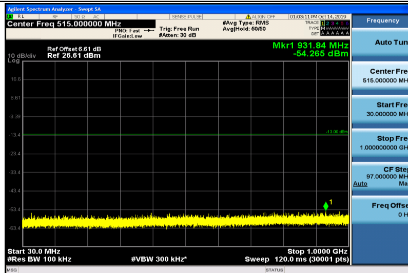
Band2-5MHz-16QAM-19175-1RB#0-30~1000MHz
