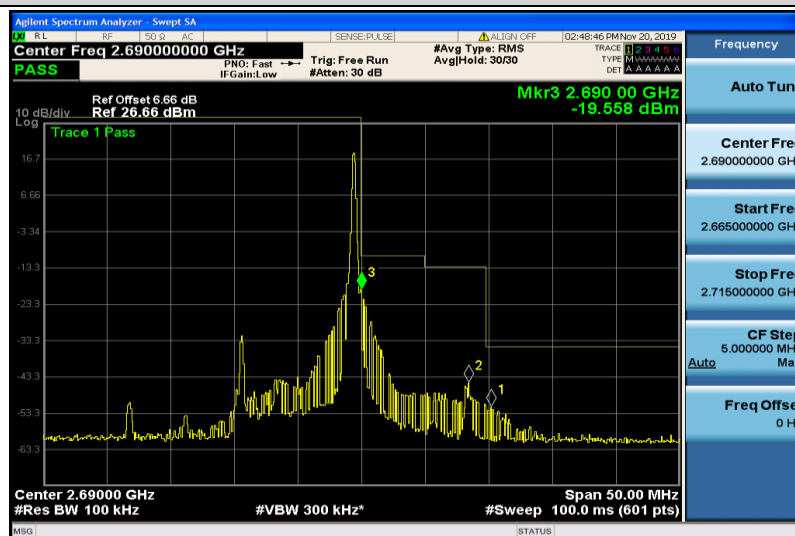
Band41-10MHz-QPSK-41540-1RB#49
