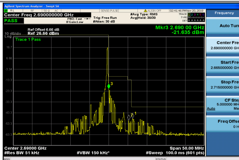
Band41-5MHz-QPSK-41565-1RB#24
