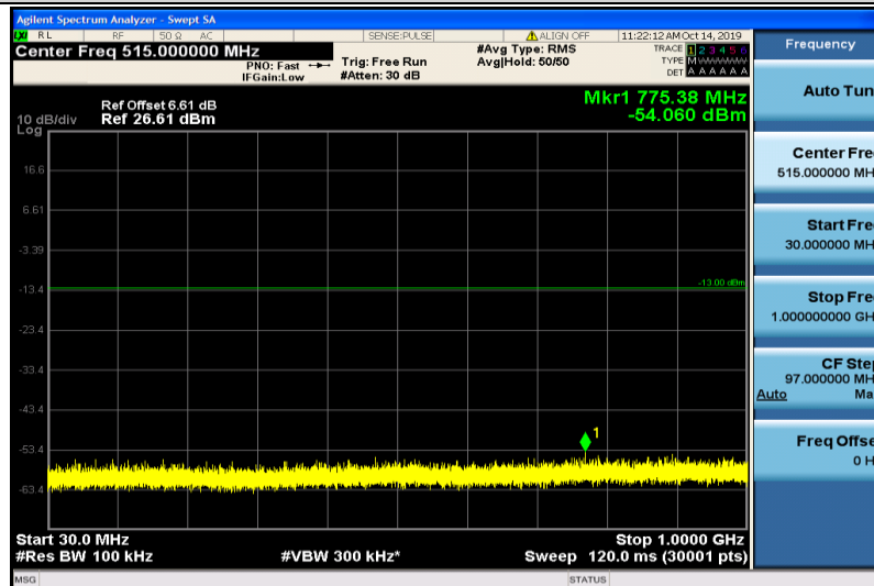
Band2-3MHz-16QAM-19185-1RB#0-30~1000MHz
