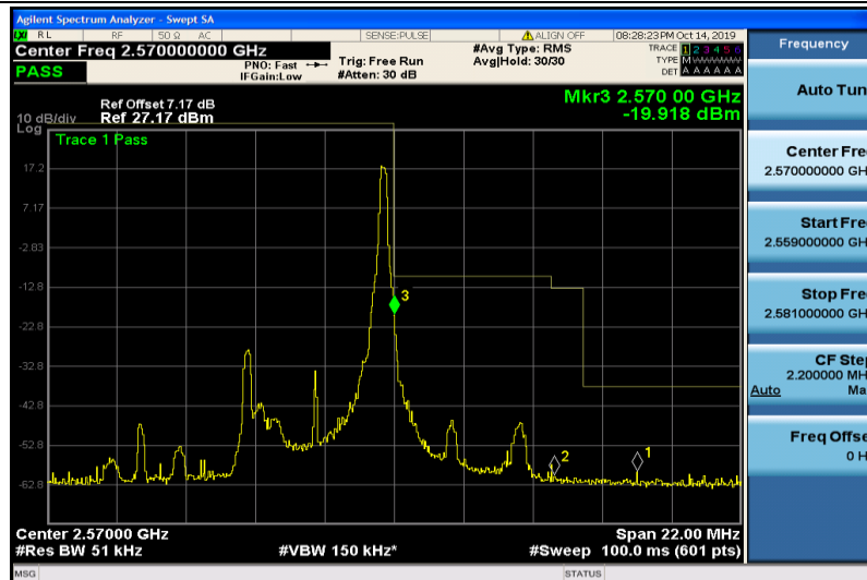
Band7-5MHz-QPSK-21425-1RB#24
