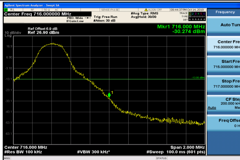
Band12-10MHz-16QAM-23130-1RB#49
