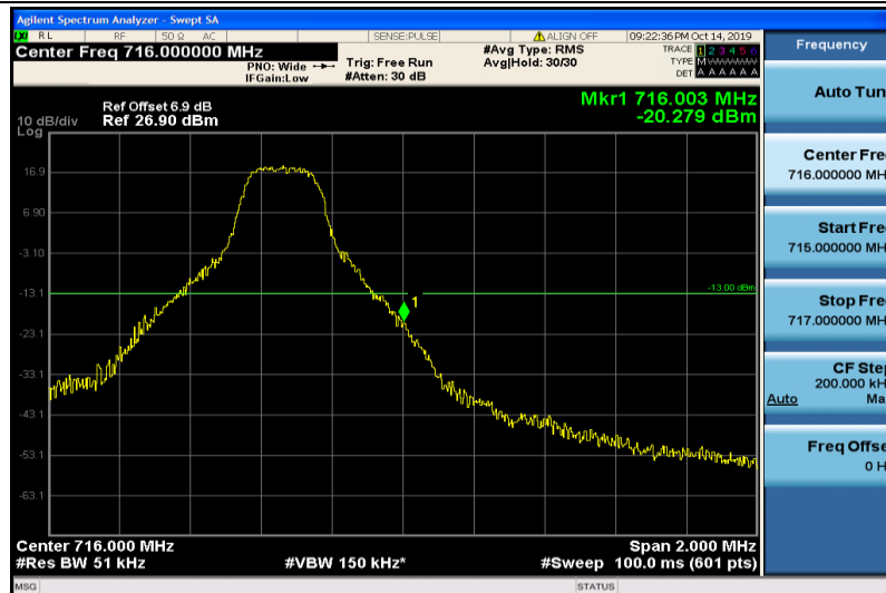
Band12-5MHz-QPSK-23155-1RB#24
