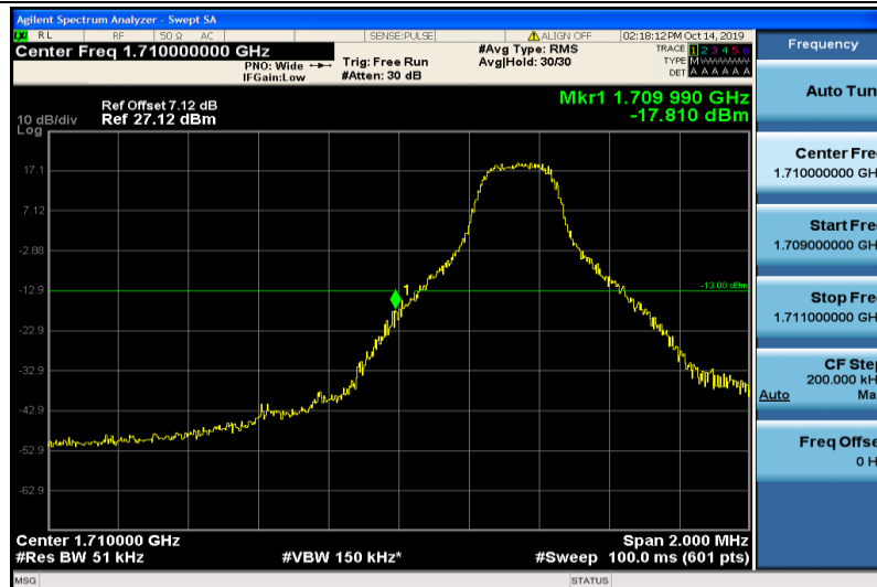
Band4-5MHz-QPSK-19975-1RB#0
