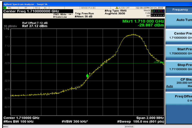
Band4-10MHz-16QAM-20000-1RB#0
