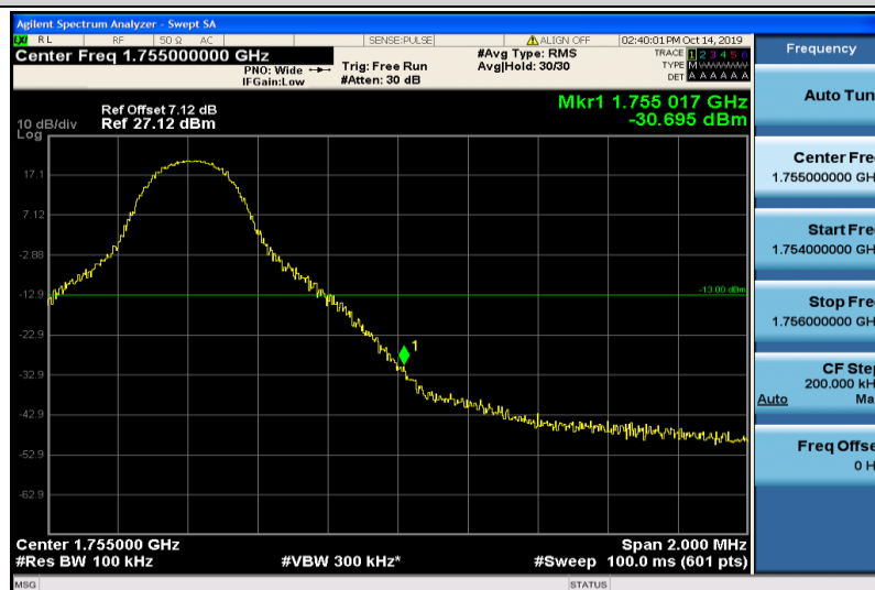
Band4-10MHz-QPSK-20350-1RB#49
