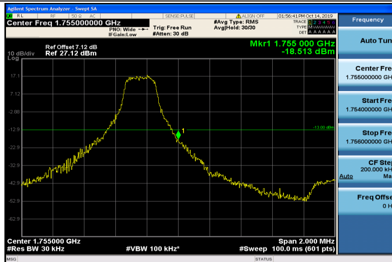
Band4-3MHz-QPSK-20385-1RB#14
