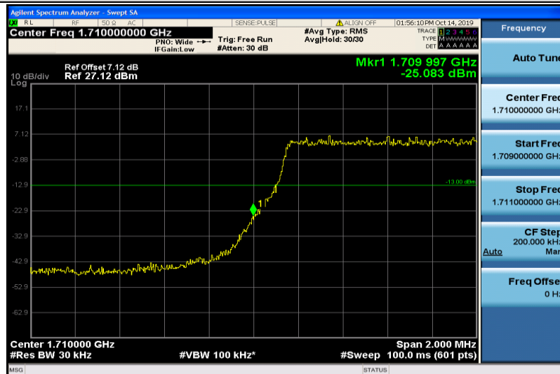
Band4-3MHz-QPSK-19965-15RB#0
