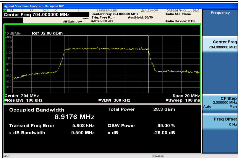
Band12-10MHz-16QAM-23060-50RB#0-8.9176
