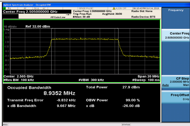
Band7-10MHz-16QAM-20800-50RB#0-8.9352
