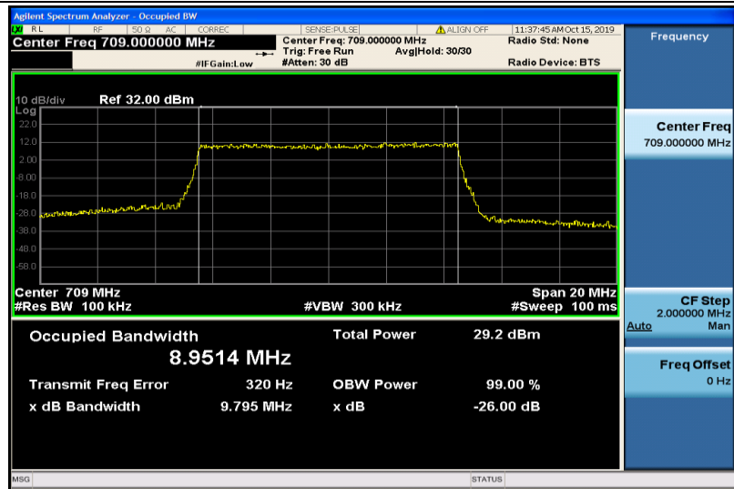
Band17-10MHz-QPSK-23780-50RB#0-8.9514
