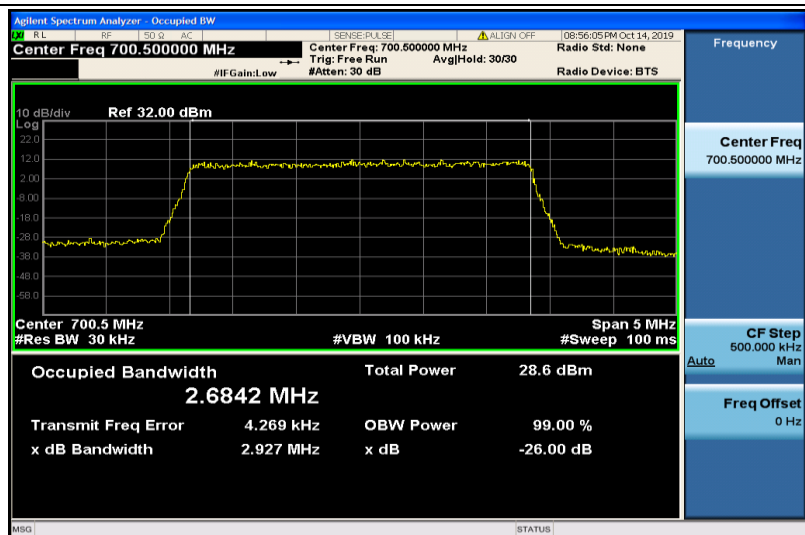
Band12-3MHz-QPSK-23025-15RB#0-2.6842
