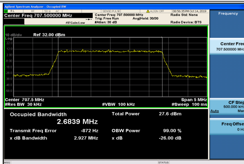
Band12-3MHz-16QAM-23095-15RB#0-2.6839
