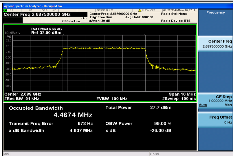
Band41-5MHz-16QAM-41565-25RB#0-4.4674
