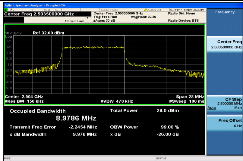
Band41-15MHz-QPSK-39725-75RB#0-8.9786
