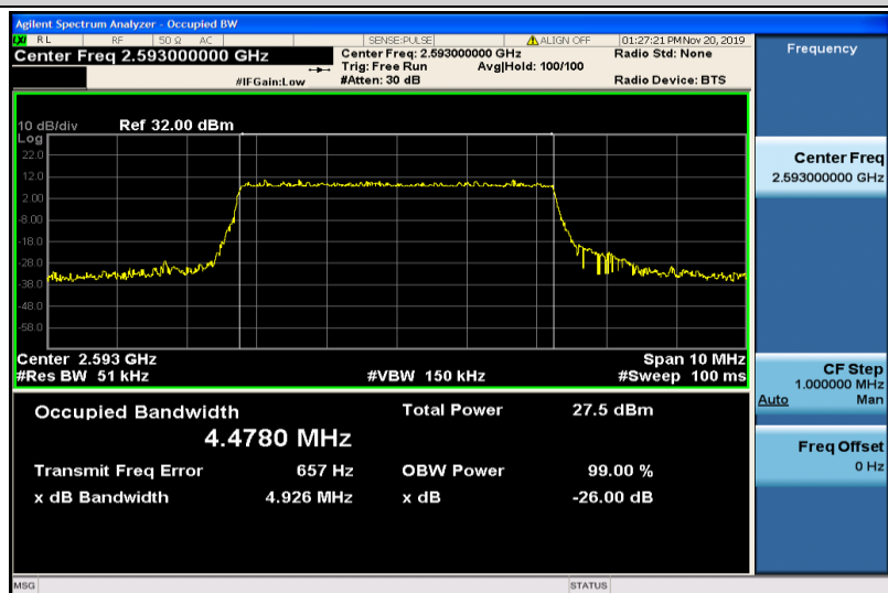
Band41-5MHz-16QAM-40620-25RB#0-4.4780
