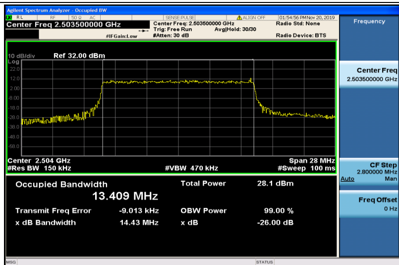
Band41-15MHz-16QAM-39725-75RB#0-13.409
