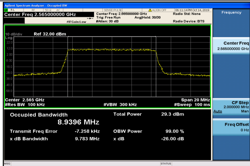
Band7-10MHz-QPSK-21400-50RB#0-8.9396
