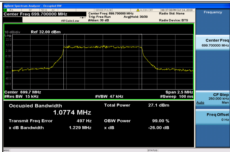
Band12-1.4MHz-16QAM-23017-6RB#0-1.0774
