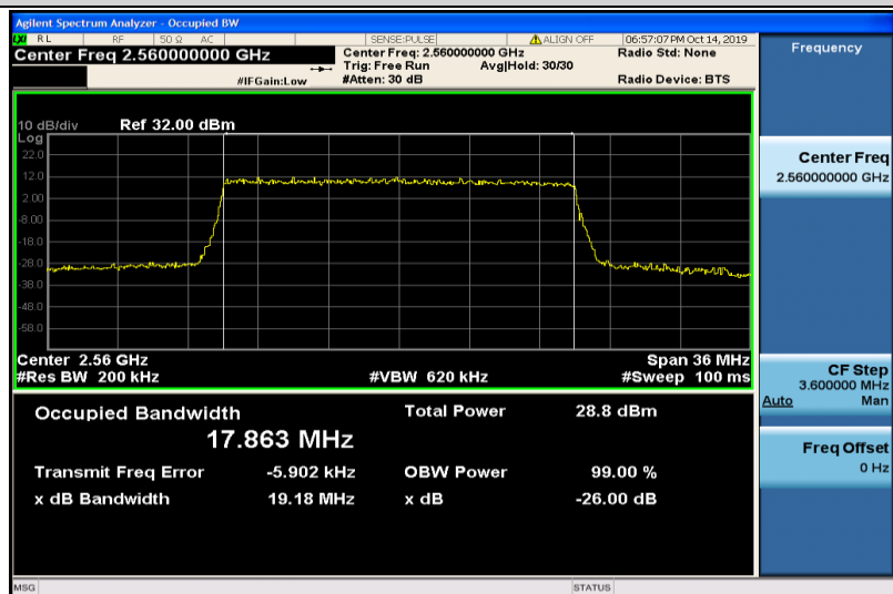
Band7-20MHz-16QAM-21350-100RB#0-17.863
