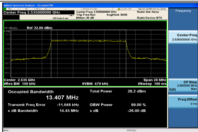
Band7-15MHz-16QAM-21100-75RB#0-13.407
