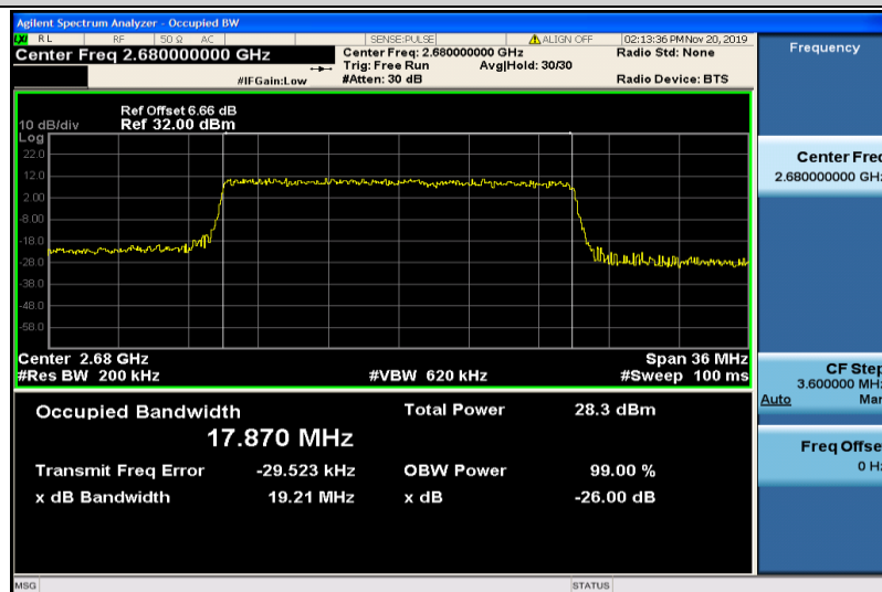
Band41-20MHz-QPSK-41490-100RB#0-17.870
