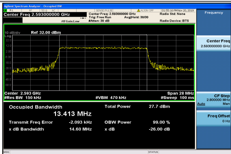
Band41-15MHz-16QAM-40620-75RB#0-13.413
