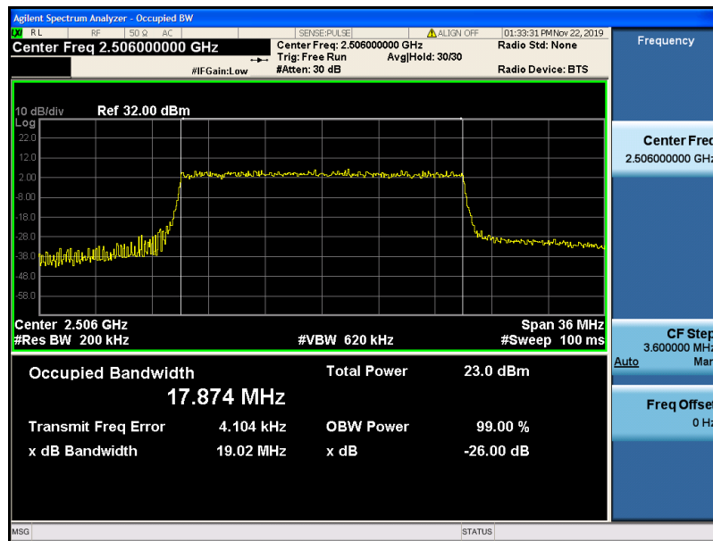
Band41-20MHz-QPSK-39750-100RB#0-17.874
