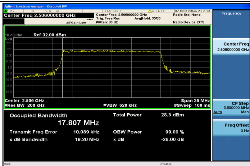
Band41-20MHz-16QAM-39750-100RB#0-17.807
