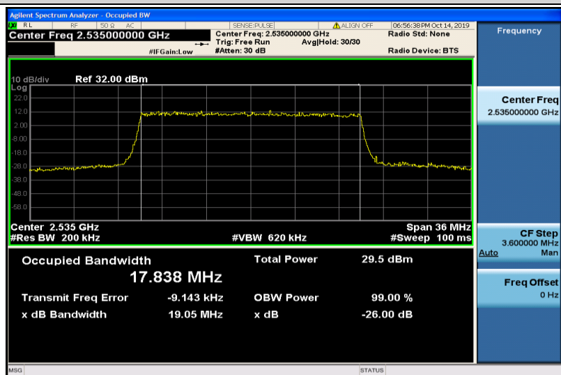
Band7-20MHz-QPSK-21100-100RB#0-17.838
