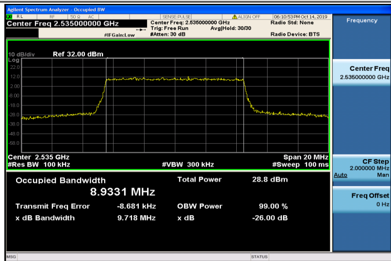
Band7-10MHz-QPSK-21100-50RB#0-8.9331
