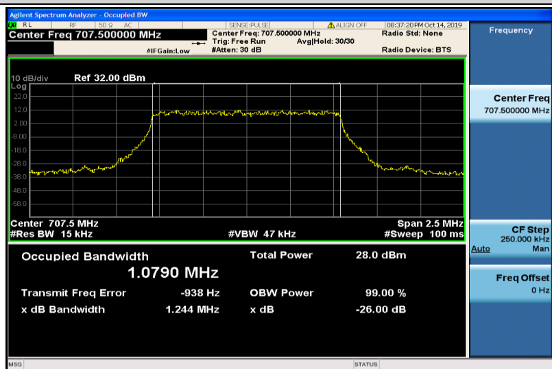
Band12-1.4MHz-QPSK-23095-6RB#0-1.0790
