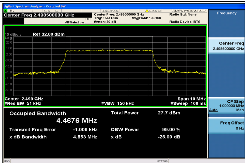
Band41-5MHz-16QAM-39675-25RB#0-4.4676
