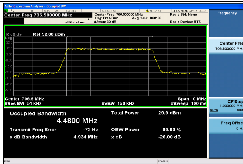
Band17-5MHz-16QAM-23755-25RB#0-4.4800
