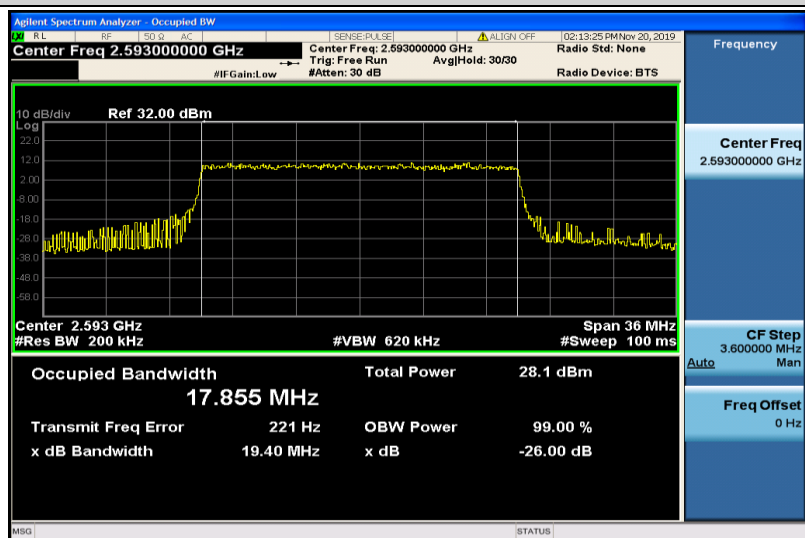
Band41-20MHz-16QAM-40620-100RB#0-17.855
