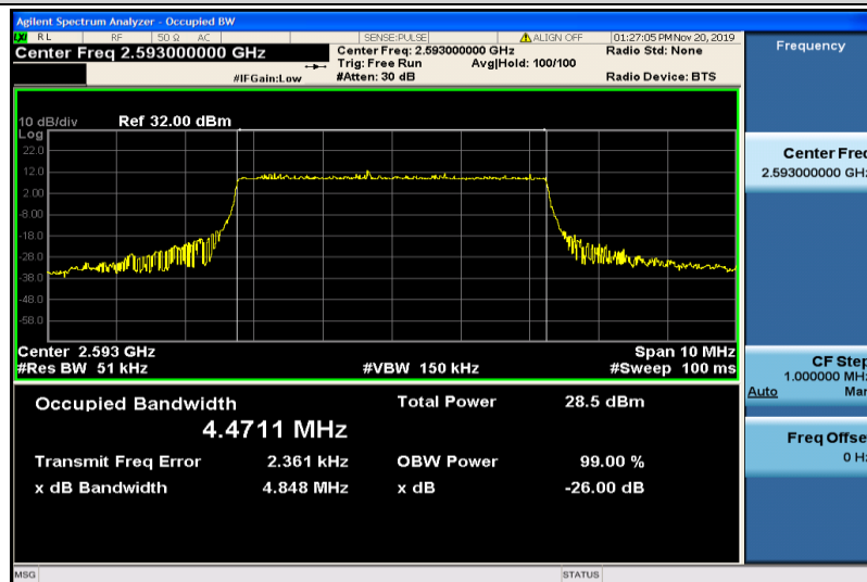
Band41-5MHz-QPSK-40620-25RB#0-4.4711
