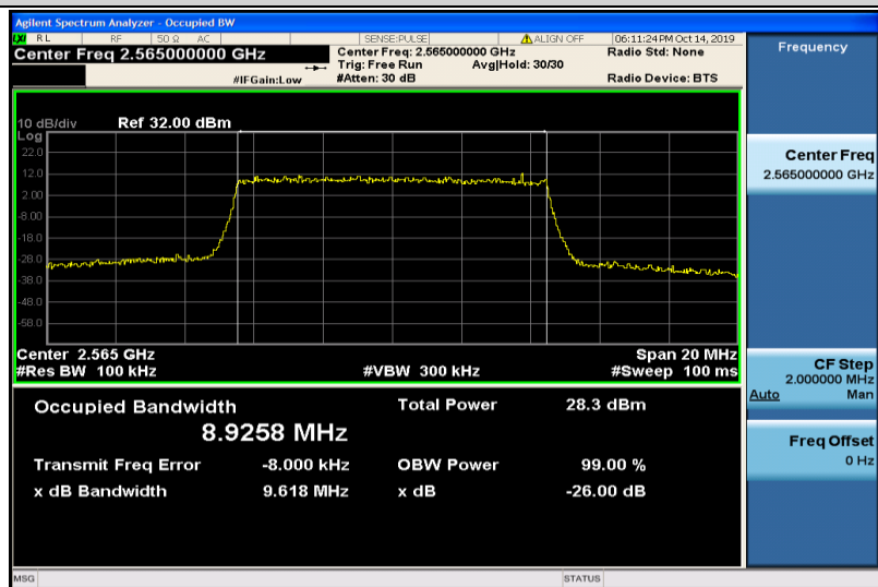
Band7-10MHz-16QAM-21400-50RB#0-8.9258
