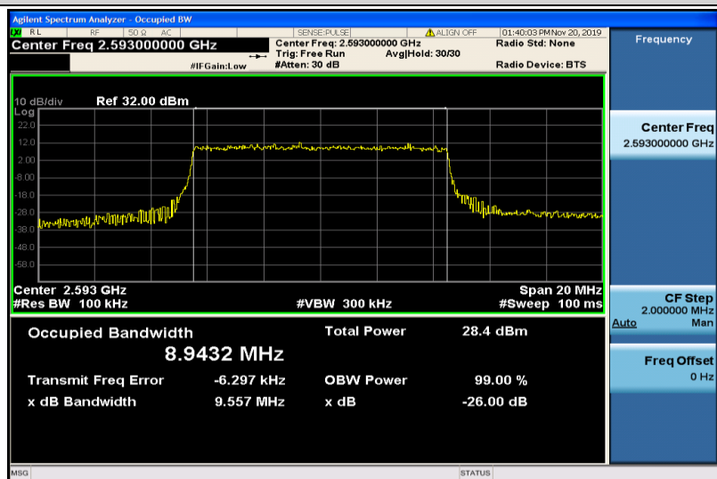
Band41-10MHz-QPSK-40620-50RB#0-8.9432
