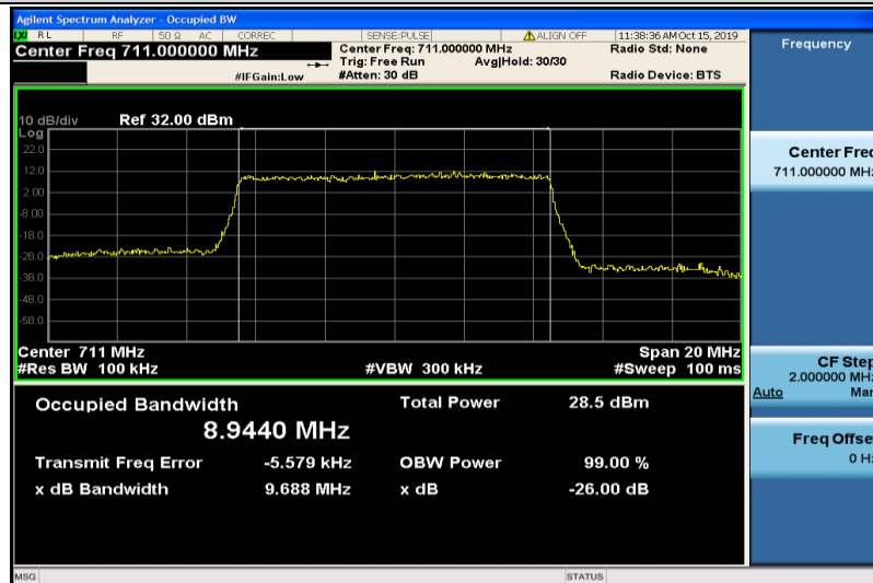
Band17-10MHz-16QAM-23800-50RB#0-8.9440
