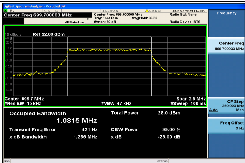
Band12-1.4MHz-QPSK-23017-6RB#0-1.0815
