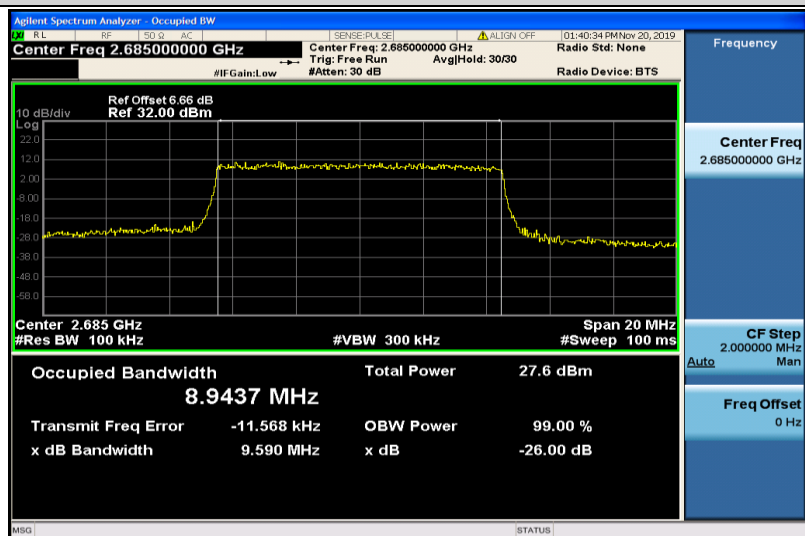
Band41-10MHz-16QAM-41540-50RB#0-8.9437
