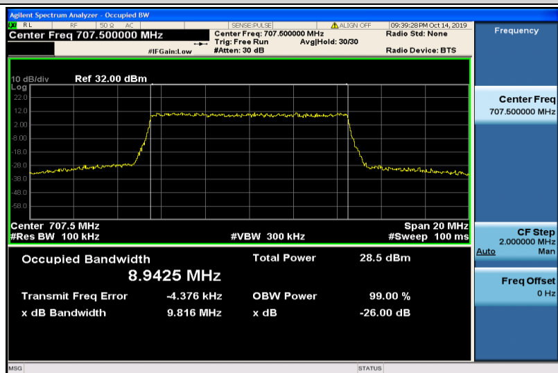
Band12-10MHz-16QAM-23095-50RB#0-8.9425
