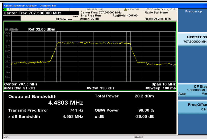
Band12-5MHz-16QAM-23095-25RB#0-4.4803
