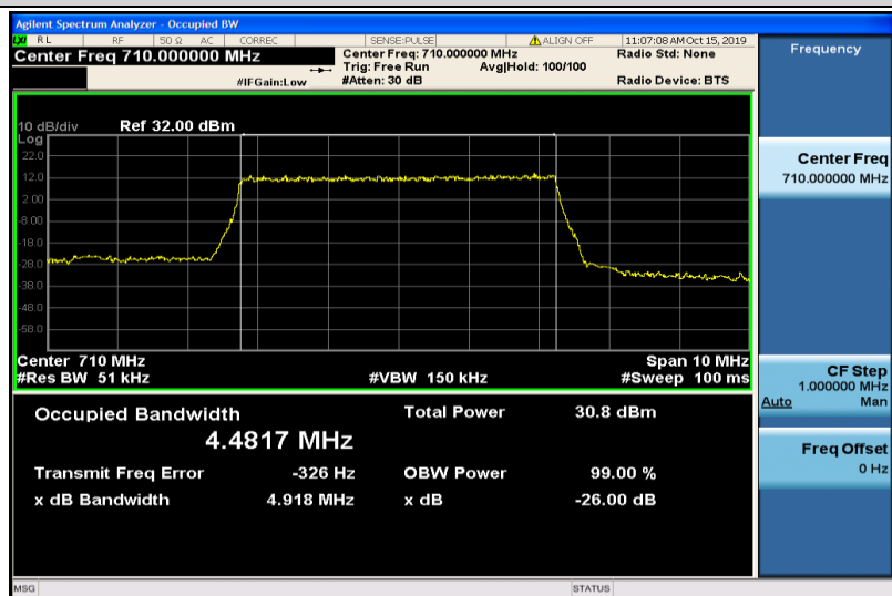
Band17-5MHz-QPSK-23790-25RB#0-4.4817
