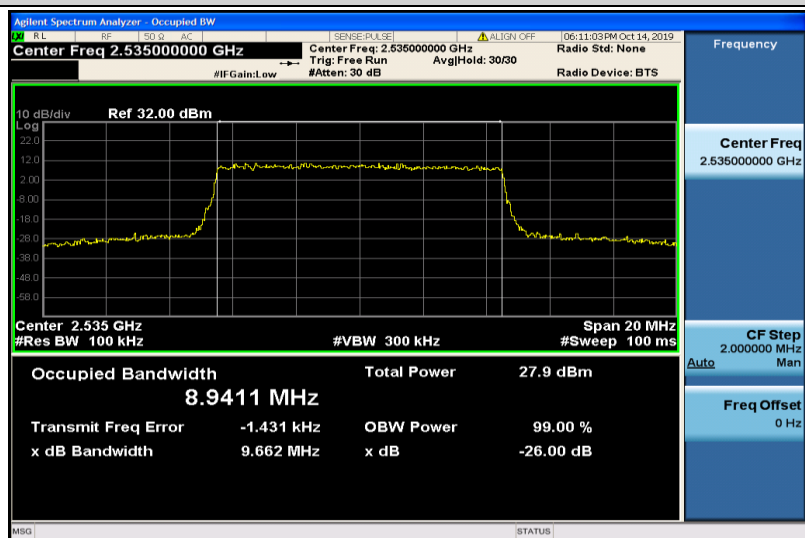
Band7-10MHz-16QAM-21100-50RB#0-8.9411
