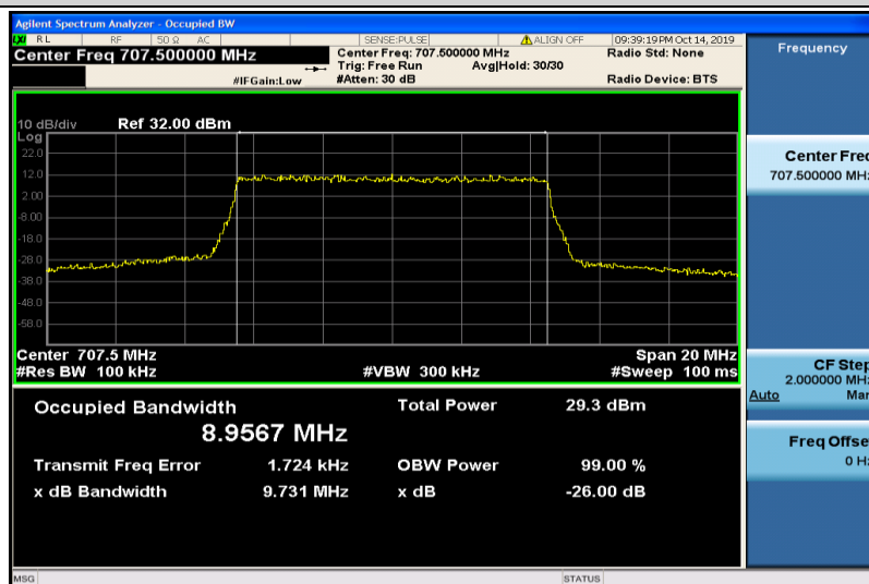
Band12-10MHz-QPSK-23095-50RB#0-8.9567
