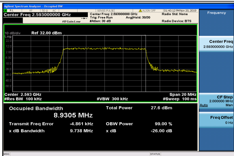
Band41-10MHz-16QAM-40620-50RB#0-8.9305
