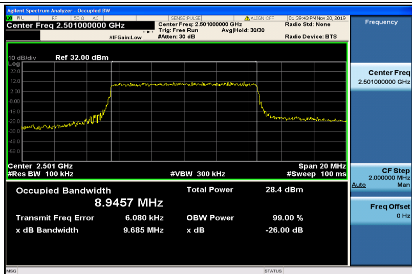
Band41-10MHz-QPSK-39700-50RB#0-8.9457
