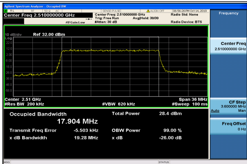
Band7-20MHz-16QAM-20850-100RB#0-17.904
