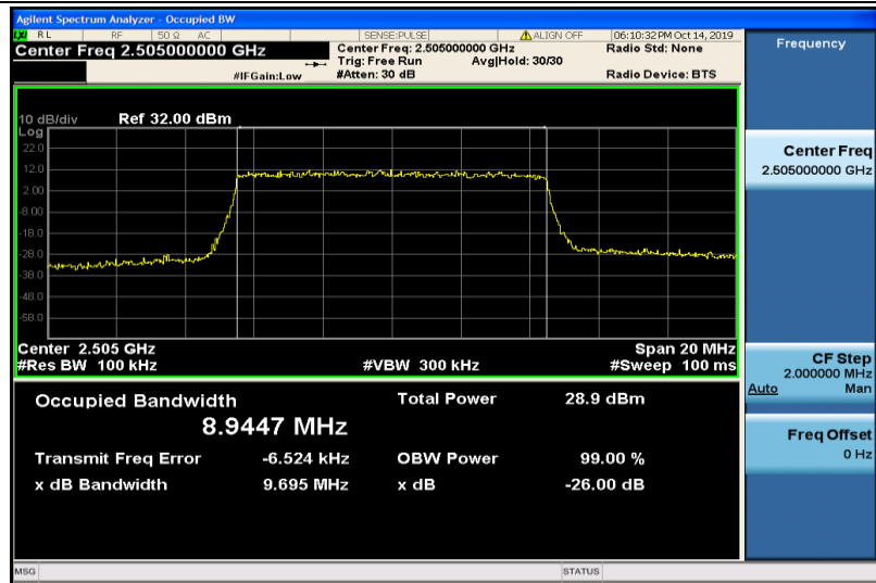
Band7-10MHz-QPSK-20800-50RB#0-8.9447
