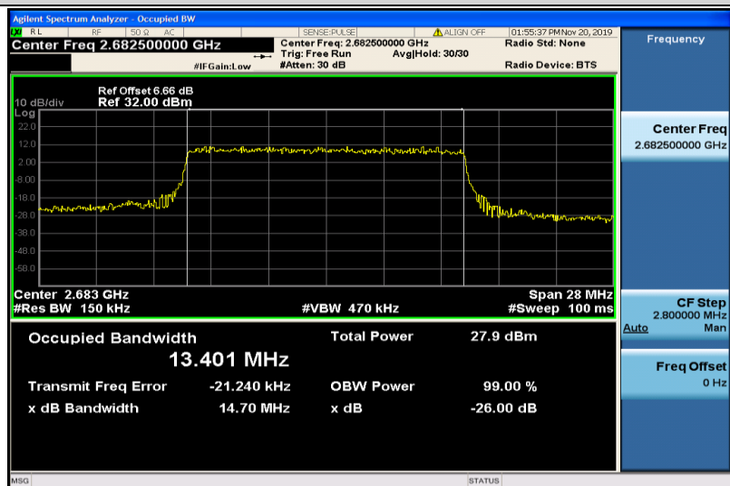
Band41-15MHz-16QAM-41515-75RB#0-13.401
