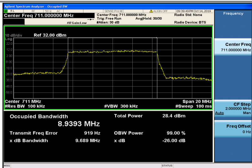
Band12-10MHz-16QAM-23130-50RB#0-8.9393
