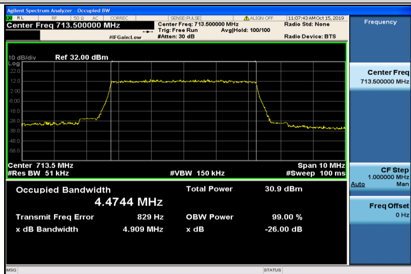
Band17-5MHz-QPSK-23825-25RB#0-4.4744
