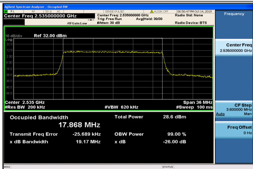
Band7-20MHz-16QAM-21100-100RB#0-17.868
