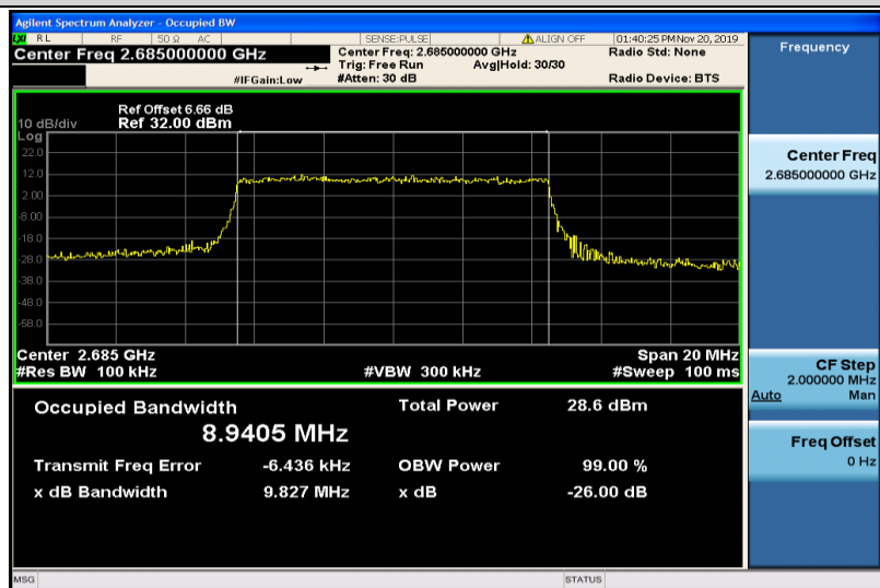
Band41-10MHz-QPSK-41540-50RB#0-8.9405
