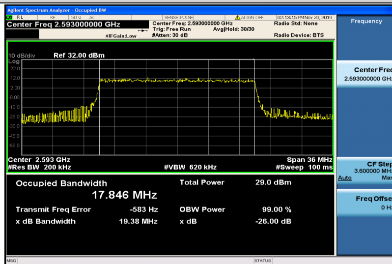
Band41-20MHz-QPSK-40620-100RB#0-17.846
