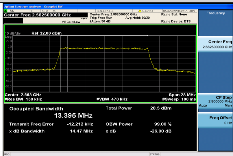
Band7-15MHz-16QAM-21375-75RB#0-13.395
