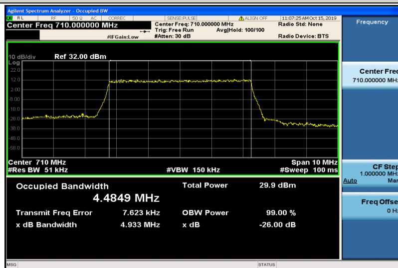
Band17-5MHz-16QAM-23790-25RB#0-4.4849
