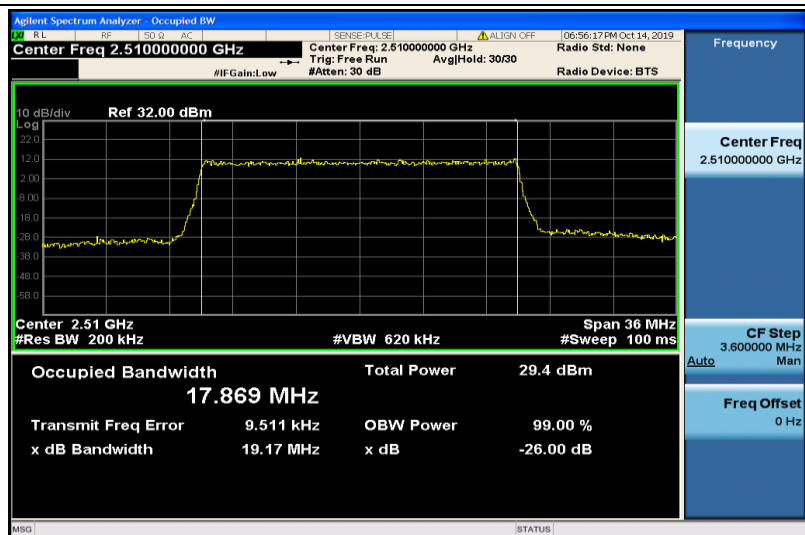
Band7-20MHz-QPSK-20850-100RB#0-17.869
