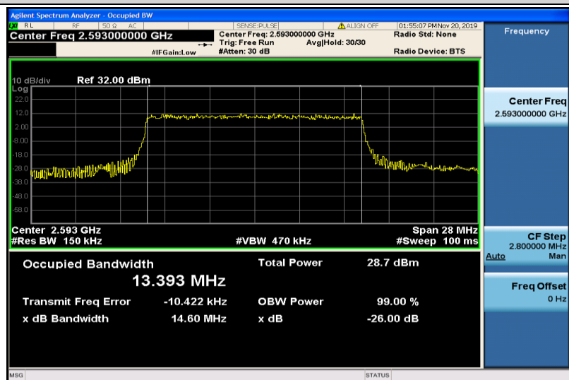
Band41-15MHz-QPSK-40620-75RB#0-13.393
