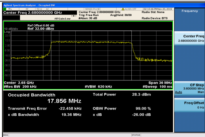
Band41-20MHz-16QAM-41490-100RB#0-17.856
