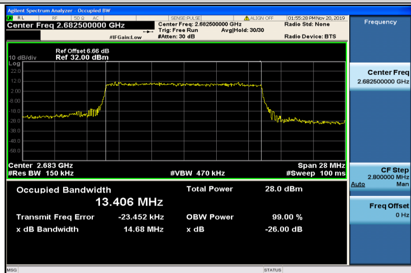
Band41-15MHz-QPSK-41515-75RB#0-13.406
