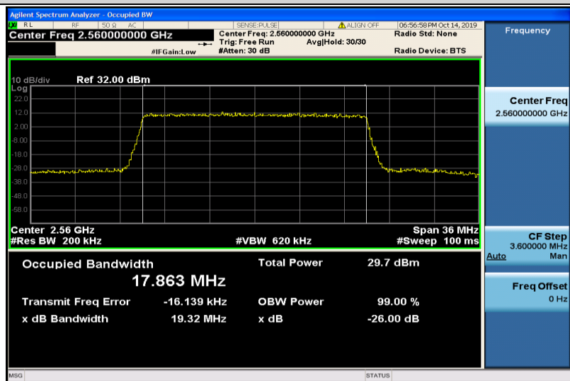
Band7-20MHz-QPSK-21350-100RB#0-17.863
