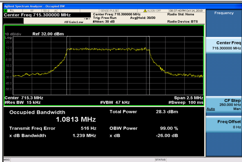
Band12-1.4MHz-QPSK-23173-6RB#0-1.0813
