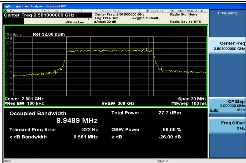
Band41-10MHz-16QAM-39700-50RB#0-8.9489
