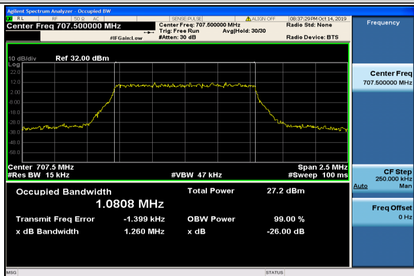
Band12-1.4MHz-16QAM-23095-6RB#0-1.0808
