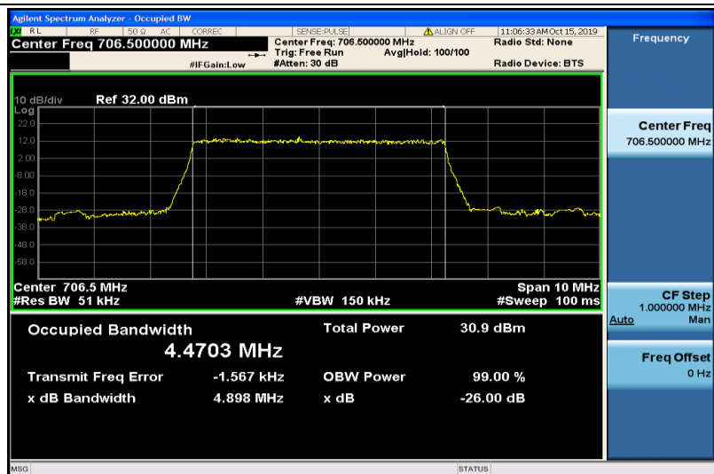
Band17-5MHz-QPSK-23755-25RB#0-4.4703
