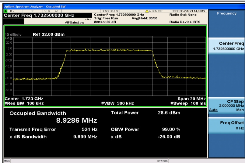
Band4-10MHz-16QAM-20175-50RB#0-8.9286
