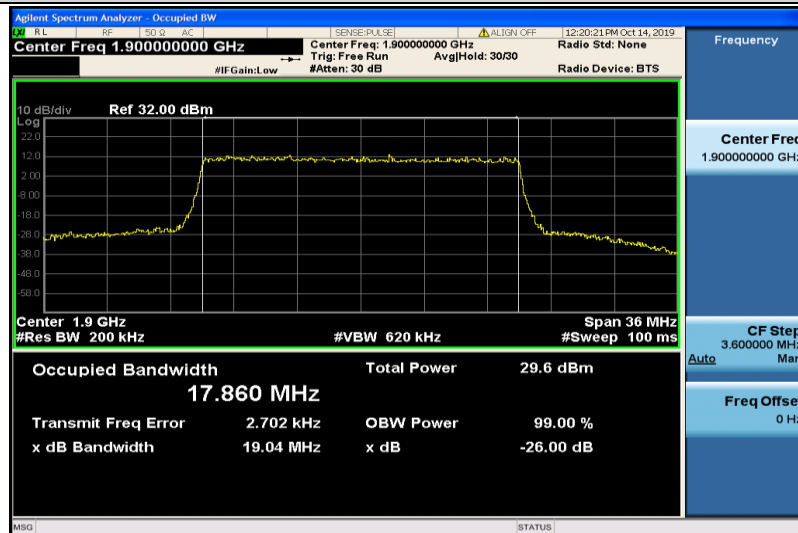
Band2-20MHz-QPSK-19100-100RB#0-17.860
