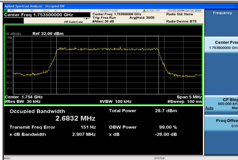
Band4-3MHz-QPSK-20385-15RB#0-2.6832
