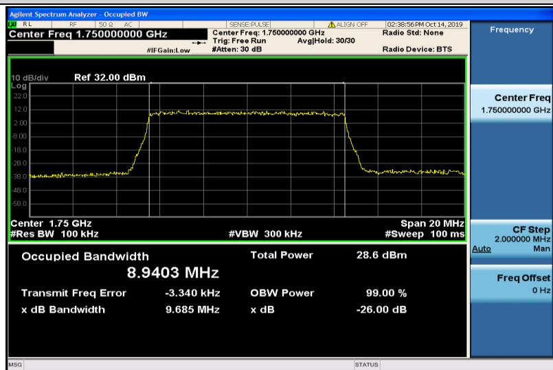
Band4-10MHz-16QAM-20350-50RB#0-8.9403
