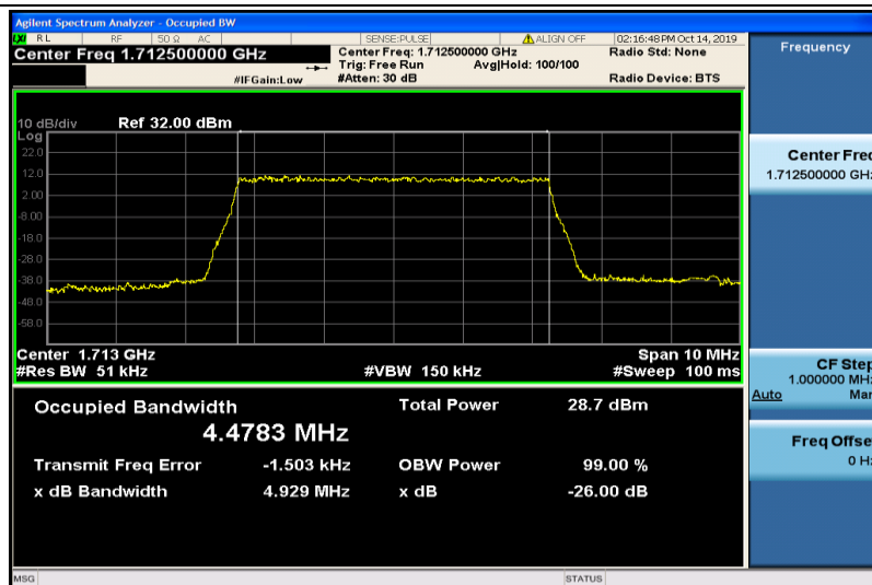
Band4-5MHz-16QAM-19975-25RB#0-4.4783
