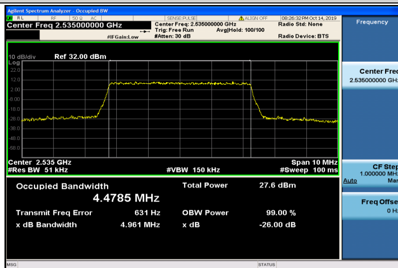
Band7-5MHz-16QAM-21100-25RB#0-4.4785
