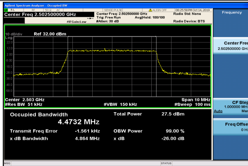
Band7-5MHz-16QAM-20775-25RB#0-4.4732
