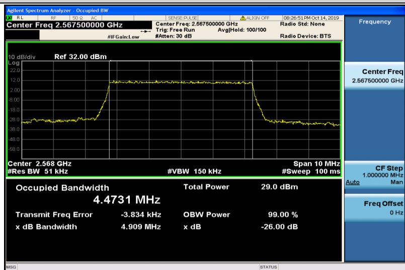
Band7-5MHz-QPSK-21425-25RB#0-4.4731
