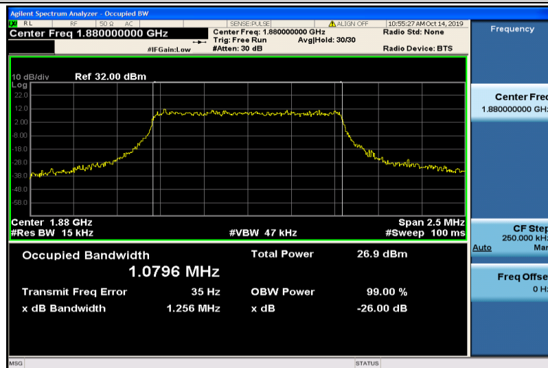
Band2-1.4MHz-16QAM-18900-6RB#0-1.0796
