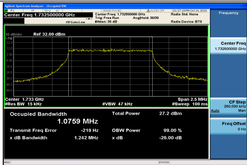
Band4-1.4MHz-16QAM-20175-6RB#0-1.0759
