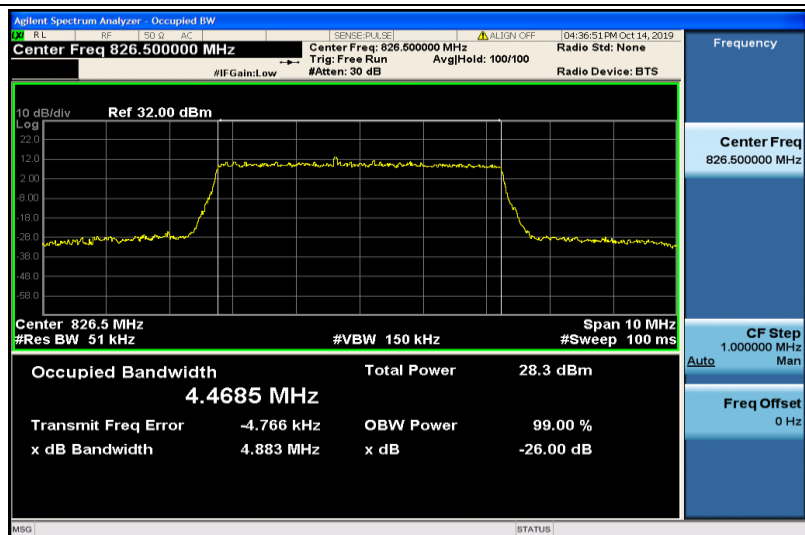
Band5-5MHz-16QAM-20425-25RB#0-4.4685
