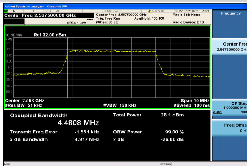
Band7-5MHz-16QAM-21425-25RB#0-4.4808
