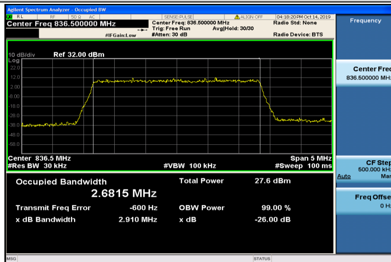
Band5-3MHz-16QAM-20525-15RB#0-2.6815
