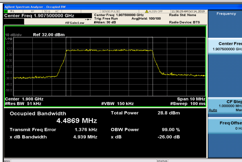
Band2-5MHz-QPSK-19175-25RB#0-4.4869
