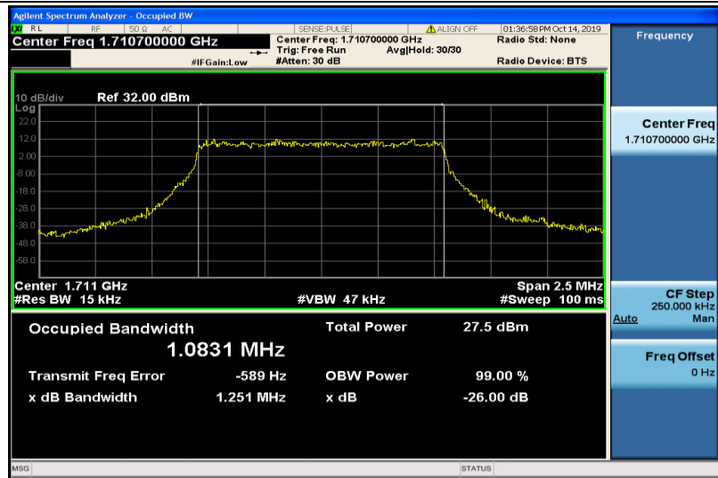
Band4-1.4MHz-16QAM-19957-6RB#0-1.0831
