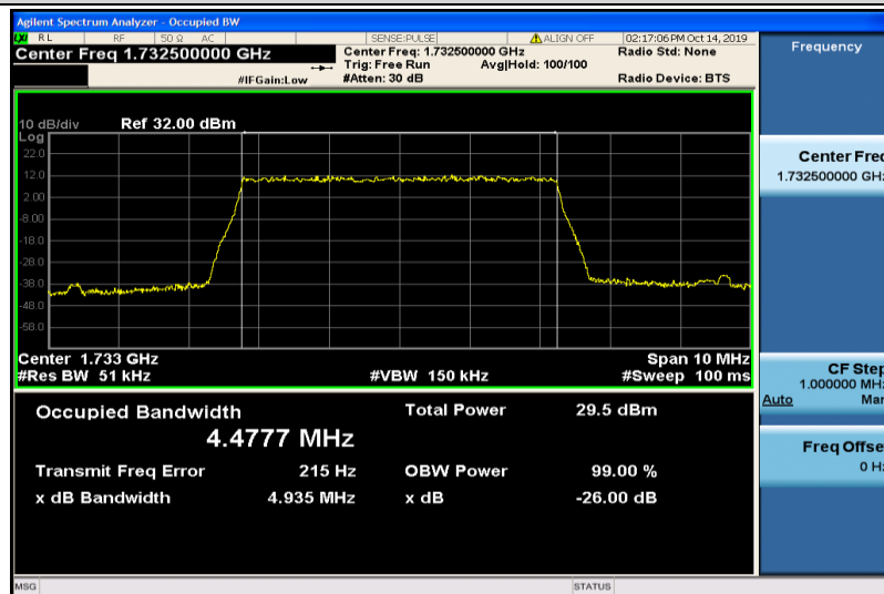
Band4-5MHz-QPSK-20175-25RB#0-4.4777
