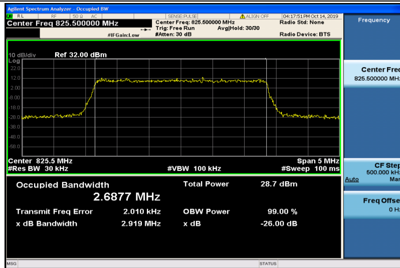
Band5-3MHz-QPSK-20415-15RB#0-2.6877
