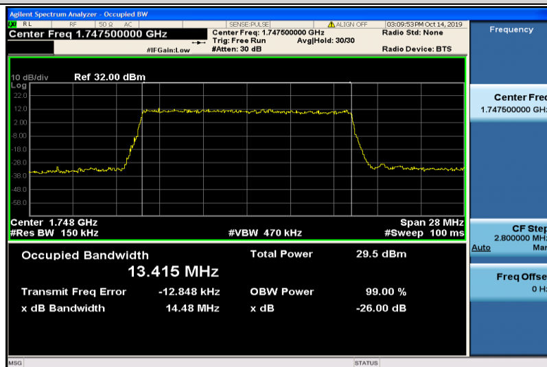
Band4-15MHz-QPSK-20325-75RB#0-13.415
