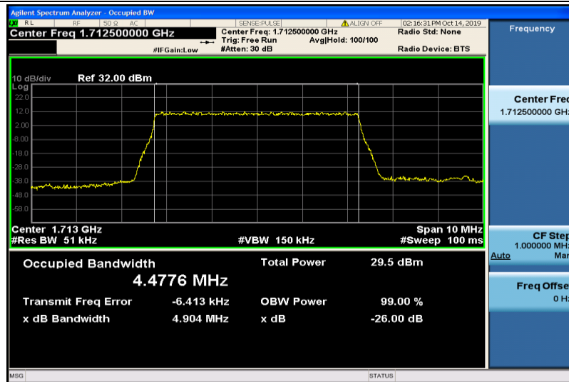
Band4-5MHz-QPSK-19975-25RB#0-4.4776
