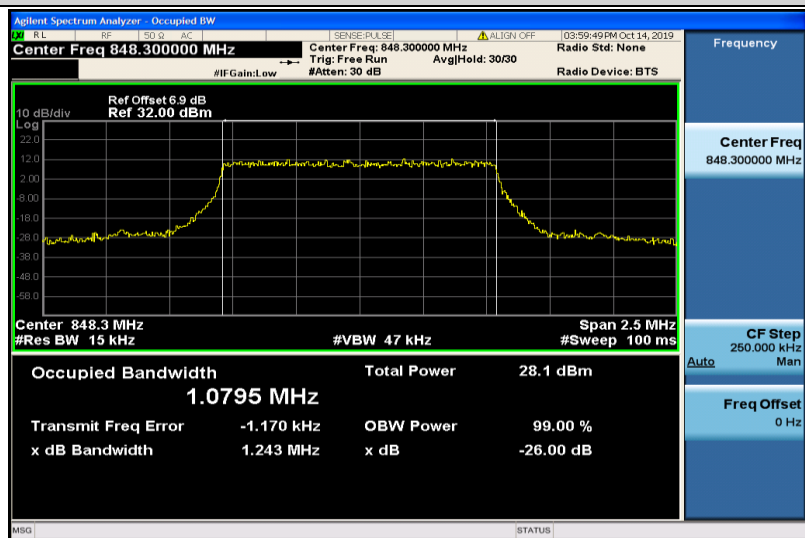
Band5-1.4MHz-QPSK-20643-6RB#0-1.0795
