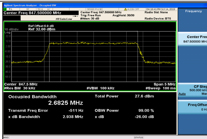
Band5-3MHz-16QAM-20635-15RB#0-2.6825
