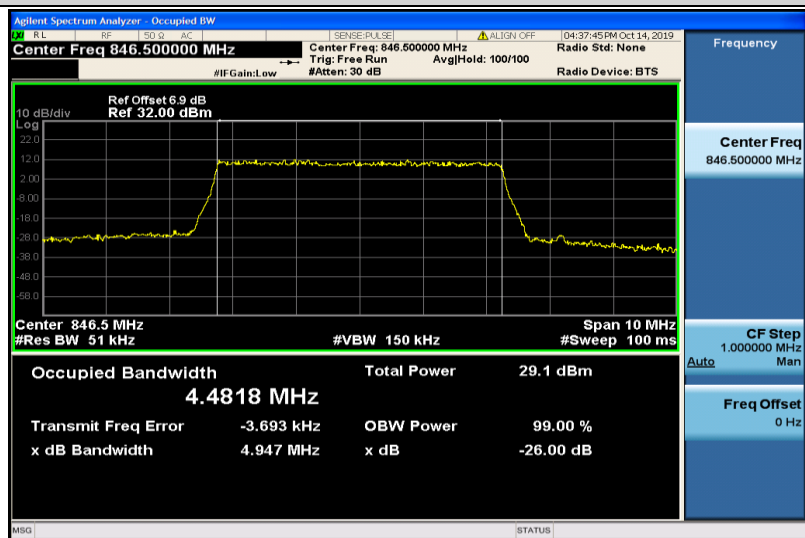
Band5-5MHz-QPSK-20625-25RB#0-4.4818
