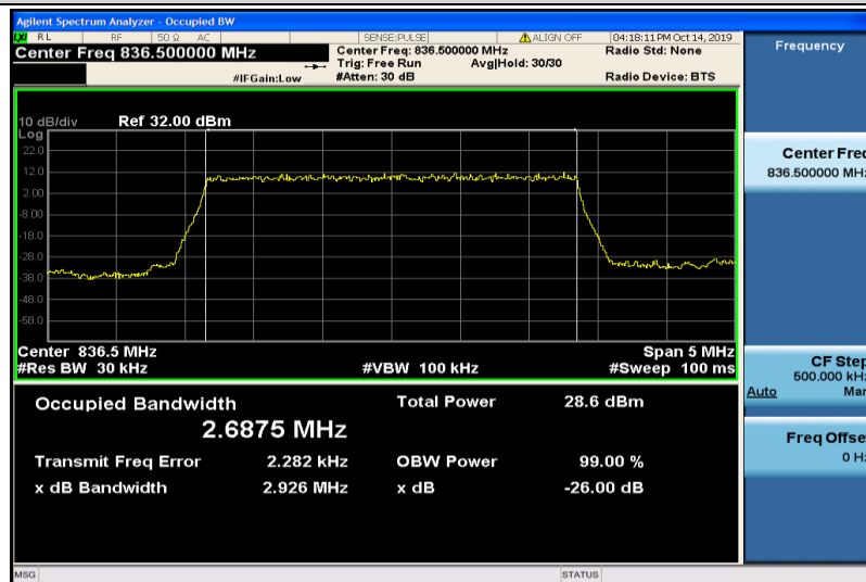
Band5-3MHz-QPSK-20525-15RB#0-2.6875
