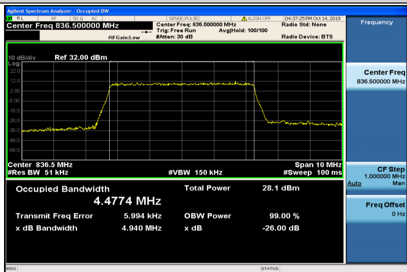
Band5-5MHz-16QAM-20525-25RB#0-4.4774
