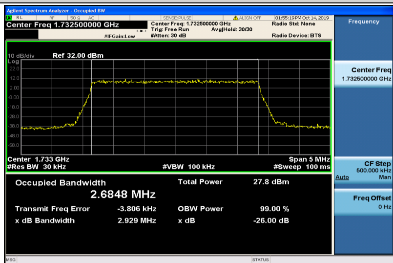
Band4-3MHz-16QAM-20175-15RB#0-2.6848
