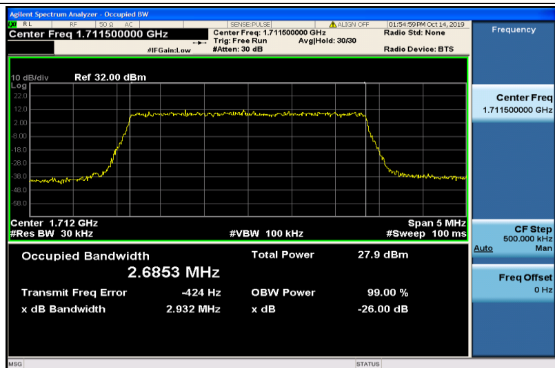
Band4-3MHz-16QAM-19965-15RB#0-2.6853
