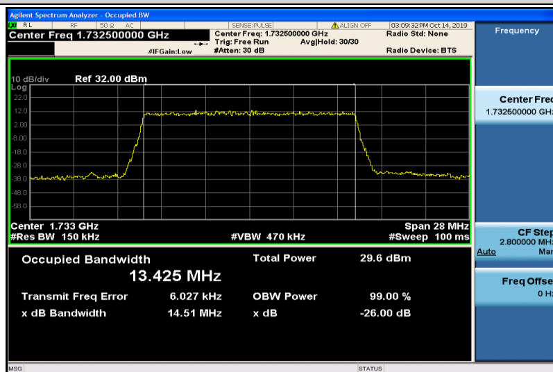
Band4-15MHz-QPSK-20175-75RB#0-13.425
