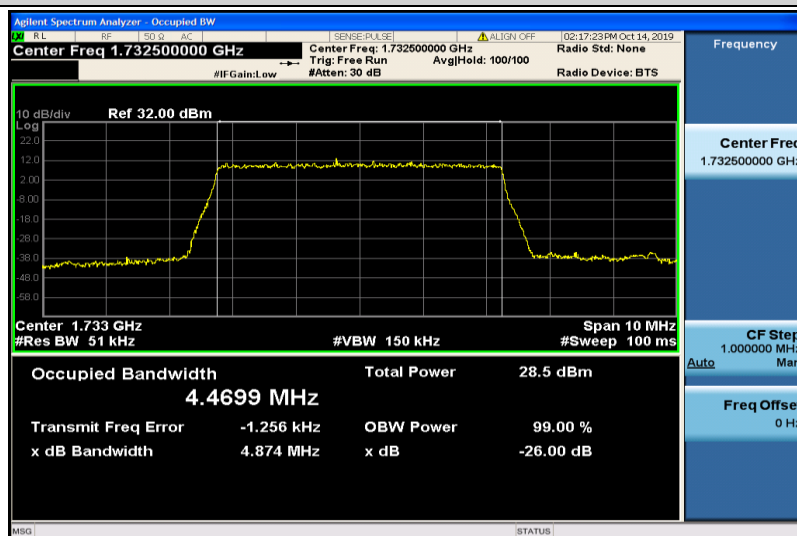
Band4-5MHz-16QAM-20175-25RB#0-4.4699
