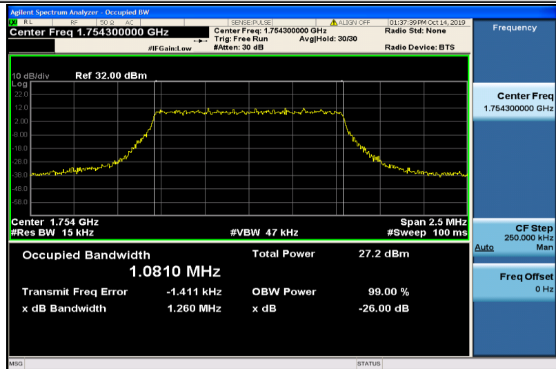
Band4-1.4MHz-16QAM-20393-6RB#0-1.0810
