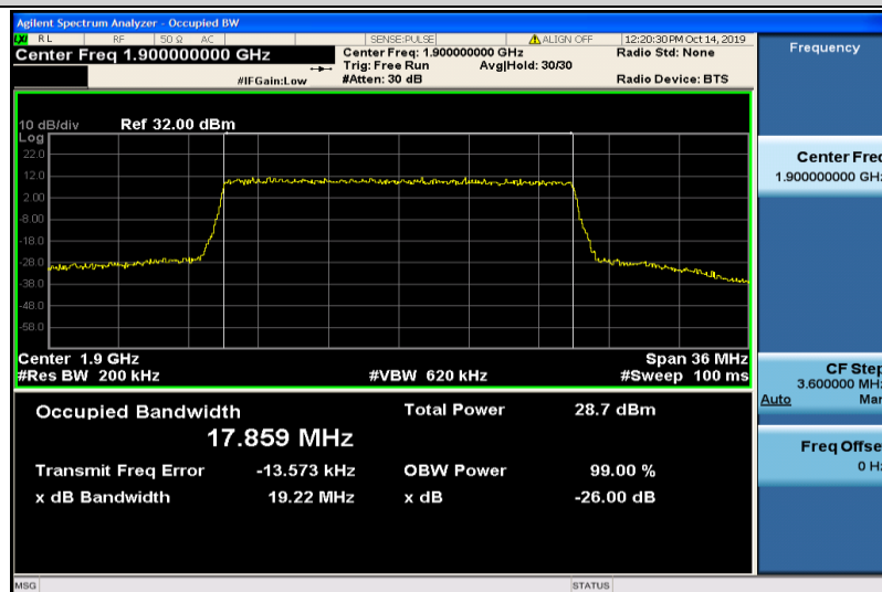
Band2-20MHz-16QAM-19100-100RB#0-17.859
