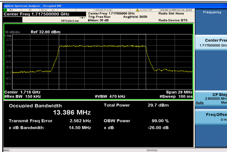
Band4-15MHz-QPSK-20025-75RB#0-13.386
