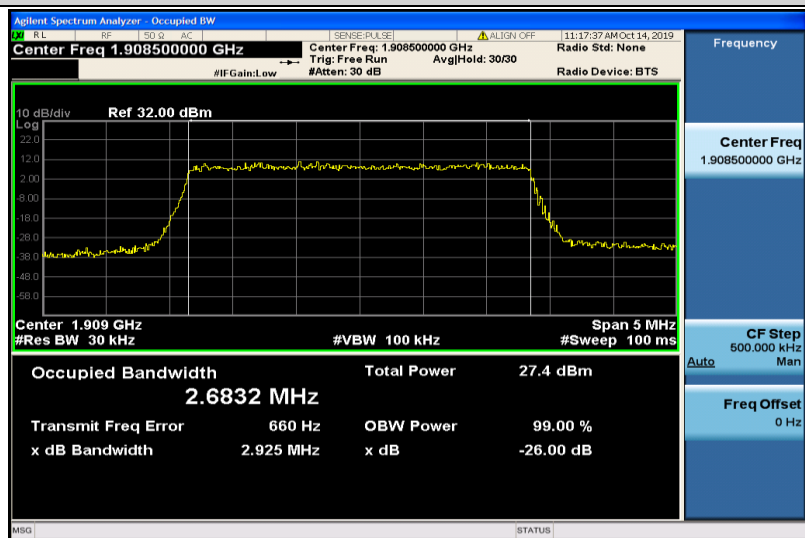
Band2-3MHz-16QAM-19185-15RB#0-2.6832
