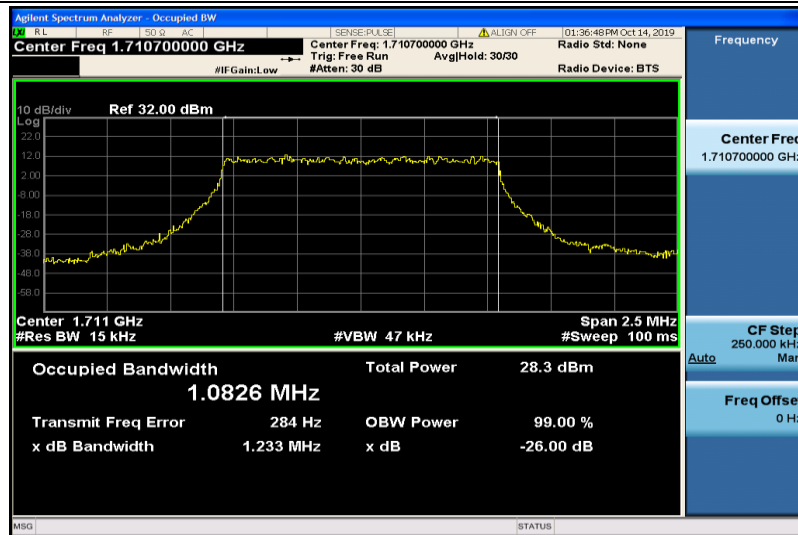
Band4-1.4MHz-QPSK-19957-6RB#0-1.0826
