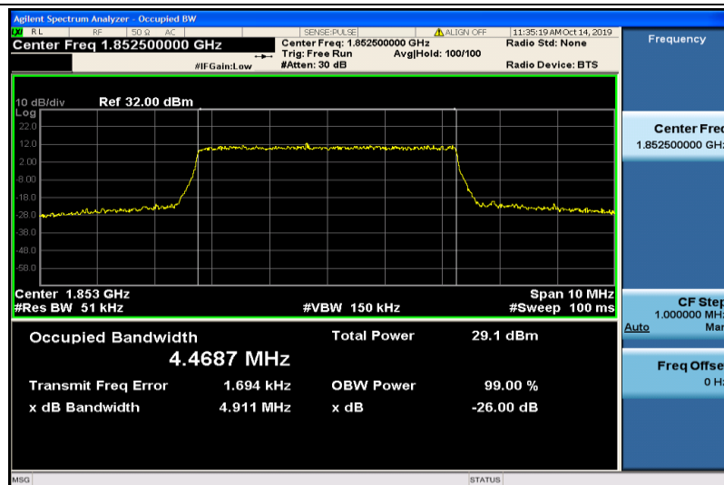
Band2-5MHz-QPSK-18625-25RB#0-4.4687
