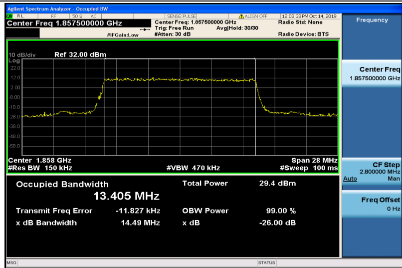
Band2-15MHz-QPSK-18675-75RB#0-13.405
