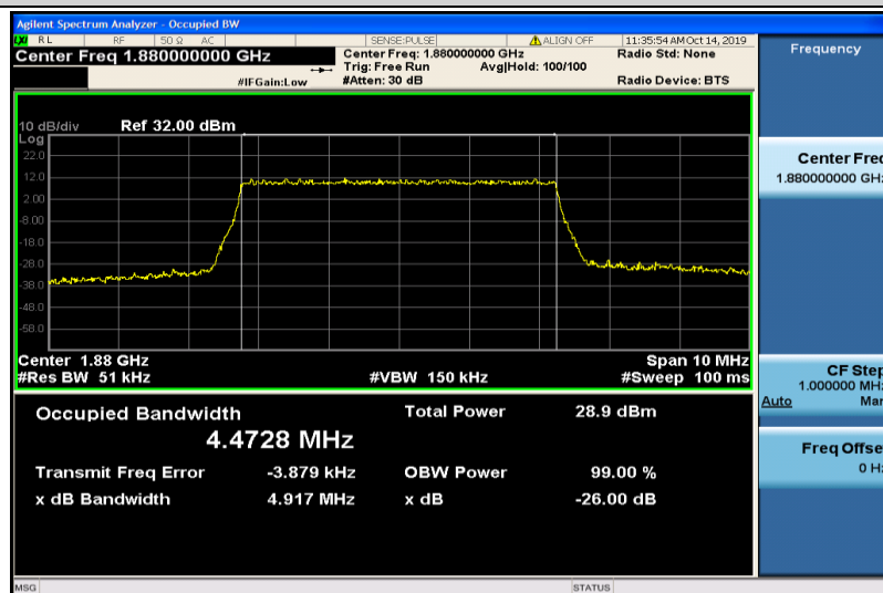
Band2-5MHz-QPSK-18900-25RB#0-4.4728
