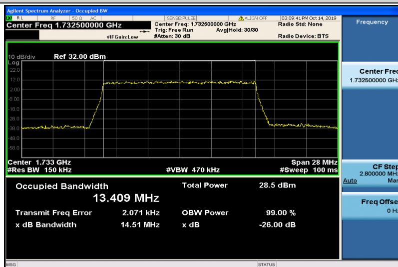
Band4-15MHz-16QAM-20175-75RB#0-13.409
