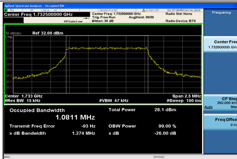
Band4-1.4MHz-QPSK-20175-6RB#0-1.0811
