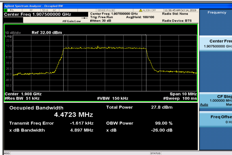
Band2-5MHz-16QAM-19175-25RB#0-4.4723
