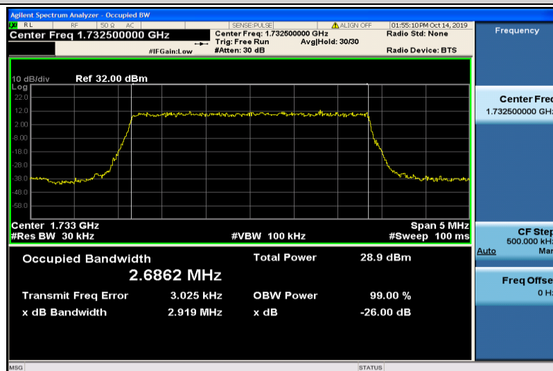
Band4-3MHz-QPSK-20175-15RB#0-2.6862
