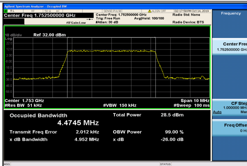
Band4-5MHz-16QAM-20375-25RB#0-4.4745
