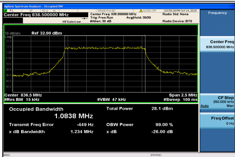
Band5-1.4MHz-QPSK-20525-6RB#0-1.0838
