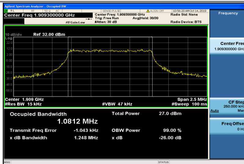
Band2-1.4MHz-16QAM-19193-6RB#0-1.0812
