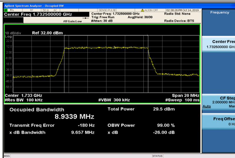
Band4-10MHz-QPSK-20175-50RB#0-8.9339
