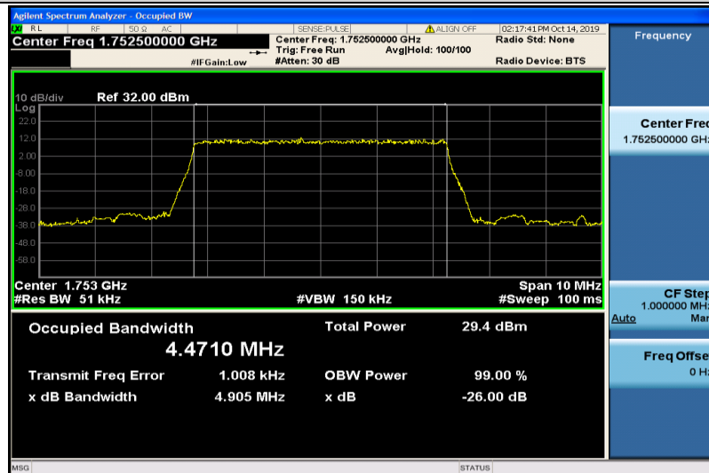
Band4-5MHz-QPSK-20375-25RB#0-4.4710
