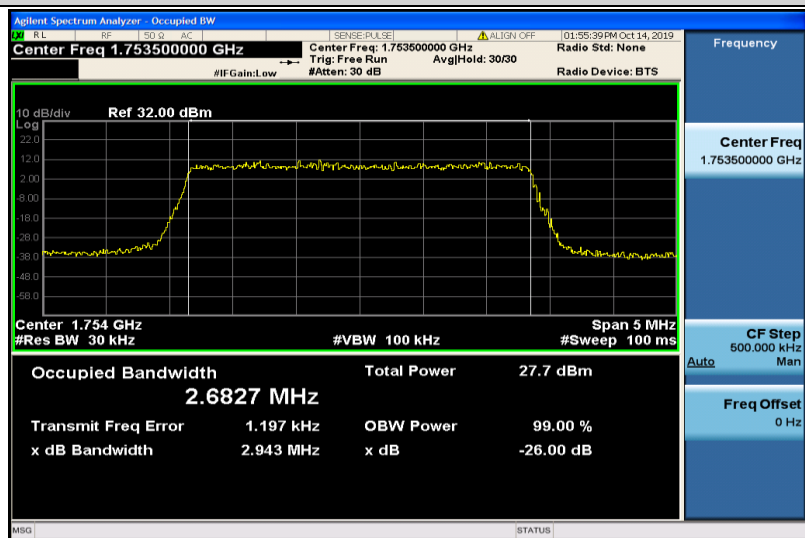
Band4-3MHz-16QAM-20385-15RB#0-2.6827
