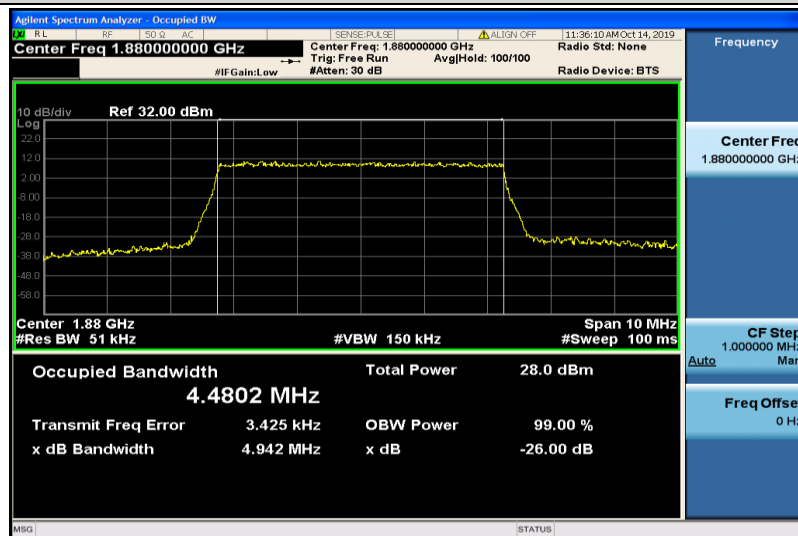
Band2-5MHz-16QAM-18900-25RB#0-4.4802
