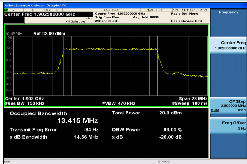
Band2-15MHz-QPSK-19125-75RB#0-13.415
