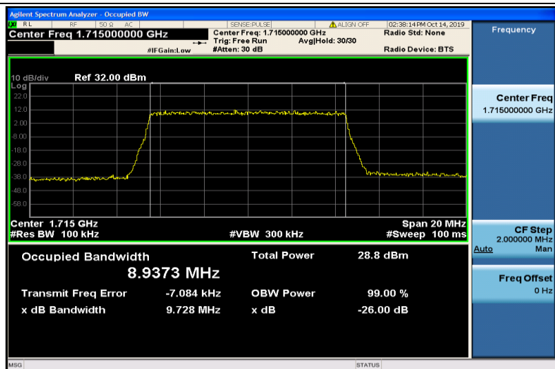
Band4-10MHz-16QAM-20000-50RB#0-8.9373
