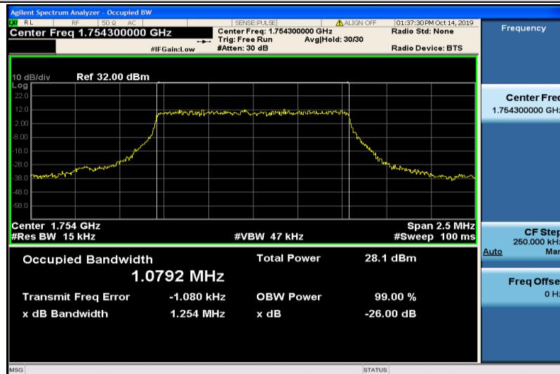
Band4-1.4MHz-QPSK-20393-6RB#0-1.0792
