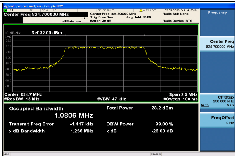
Band5-1.4MHz-QPSK-20407-6RB#0-1.0806
