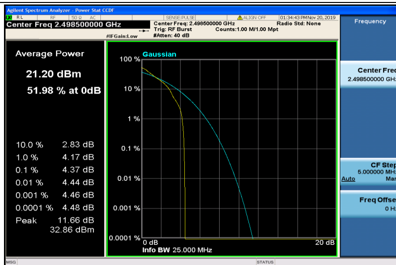
Band41-5MHz-QPSK-39675-1RB#0
