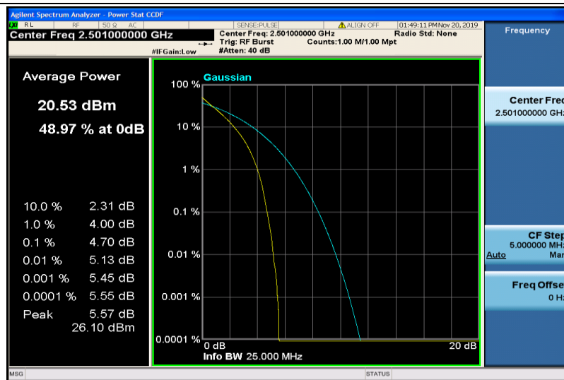
Band41-10MHz-QPSK-39700-1RB#0
