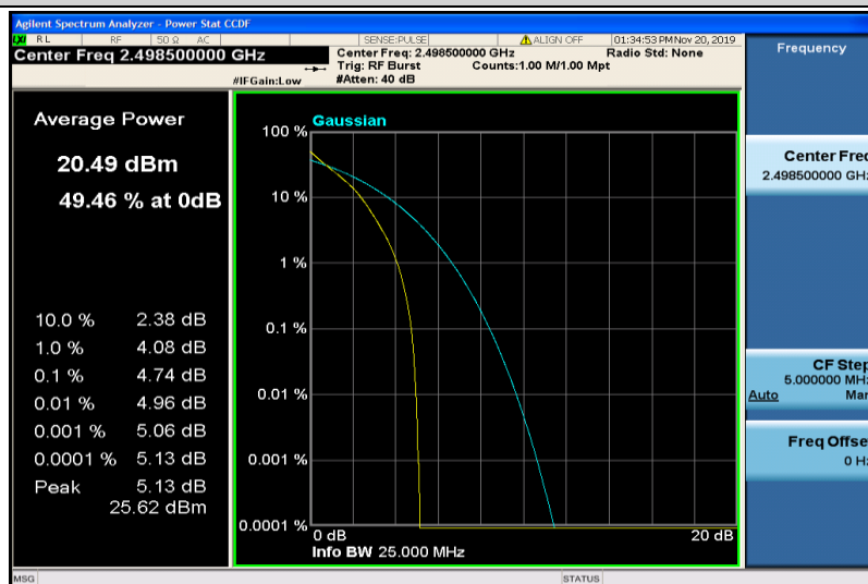
Band41-5MHz-QPSK-39675-25RB#0
