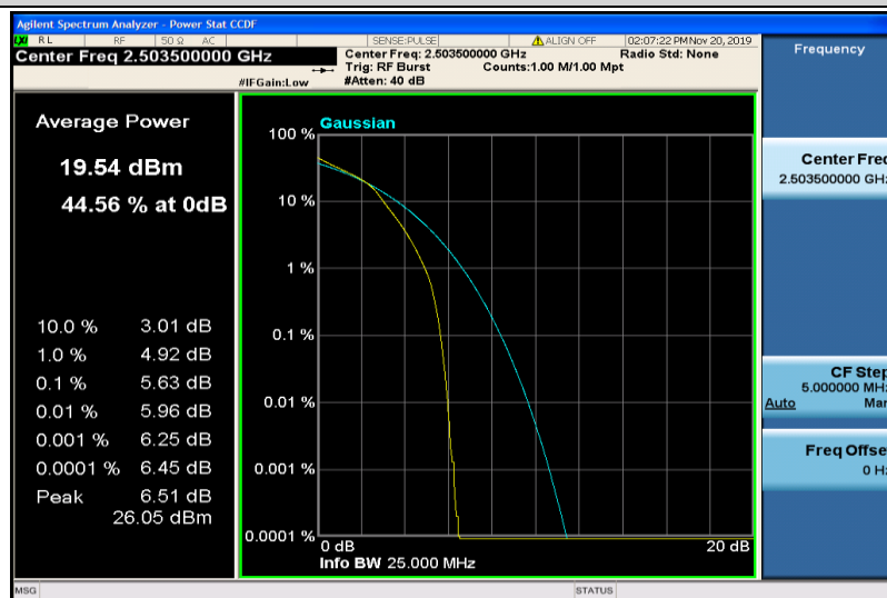
Band41-15MHz-16QAM-39725-75RB#0
