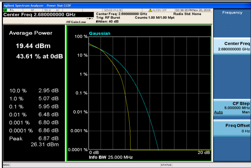
Band41-20MHz-16QAM-41490-100RB#0
