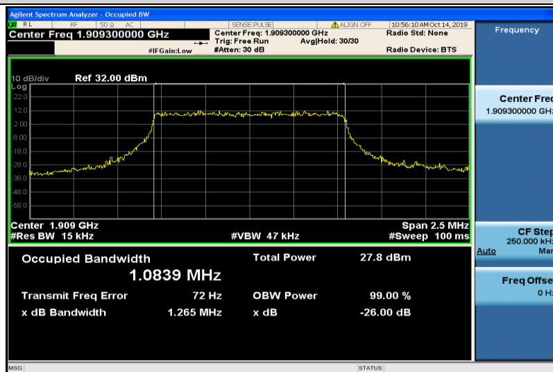
Band2-1.4MHz-QPSK-19193-6RB#0-1.0839
