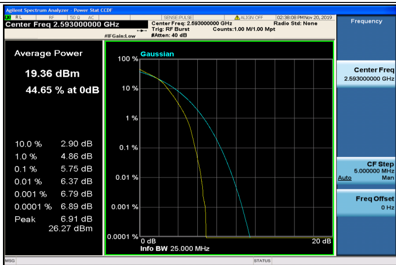
Band41-20MHz-16QAM-40620-100RB#0
