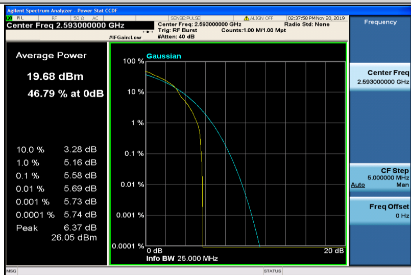
Band41-20MHz-16QAM-40620-1RB#0
