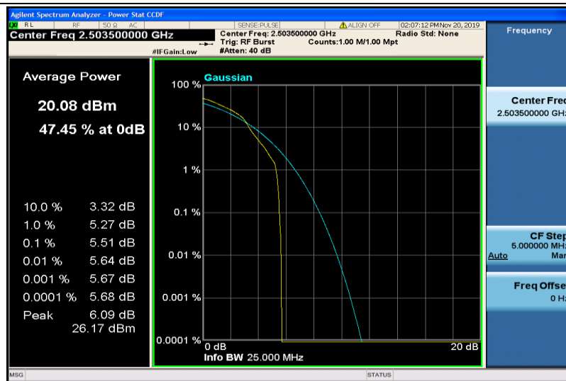
Band41-15MHz-16QAM-39725-1RB#0
