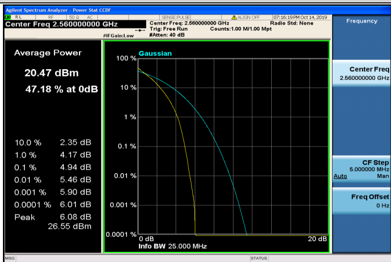
Band7-20MHz-QPSK-21350-100RB#0
