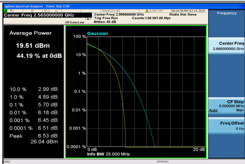
Band7-10MHz-16QAM-21400-50RB#0
