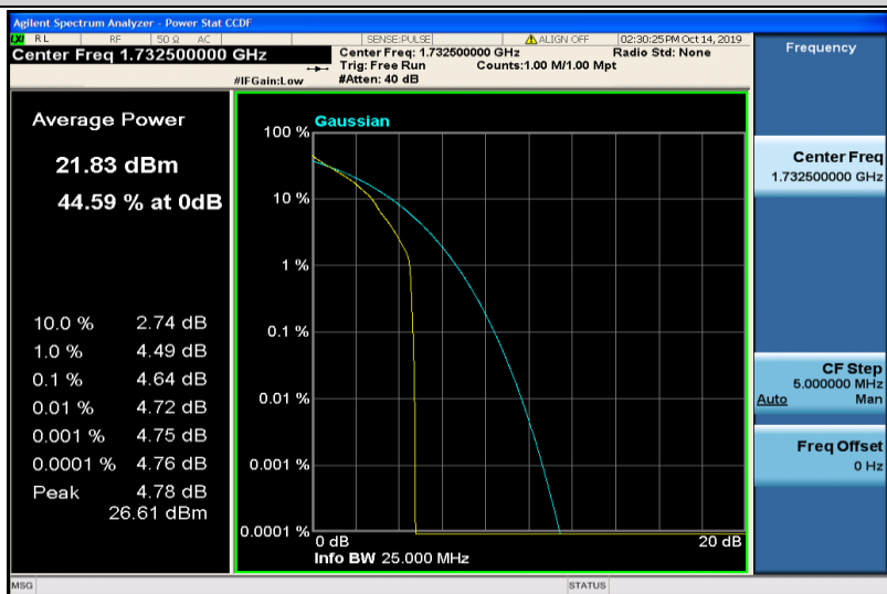
Band4-5MHz-QPSK-20175-1RB#0
