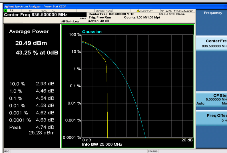
Band5-1.4MHz-16QAM-20525-1RB#0
