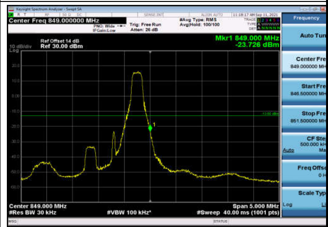
HighRange_FDD05_1.4MHz_848.3_OneRB _high_Q16
