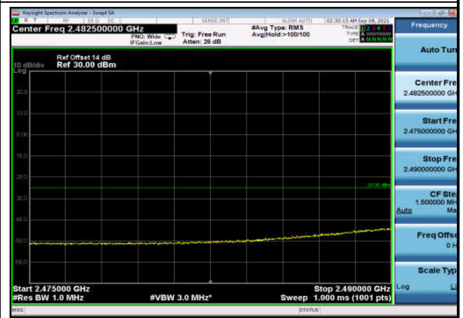
FDD07_5MHz_2502.5_Q16_fullRB_ExtraBands_Range_2475~2490
