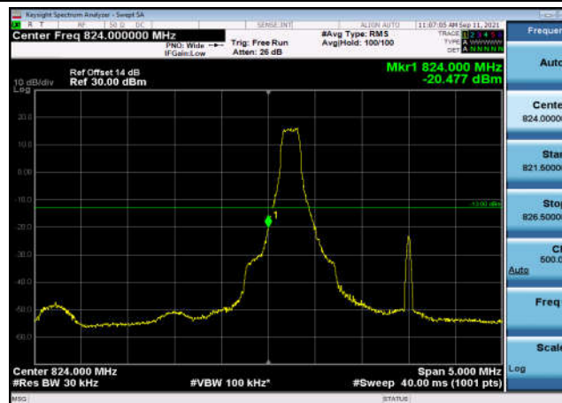
LowRange_FDD05_3MHz_825.5_OneRB _low_Q16
