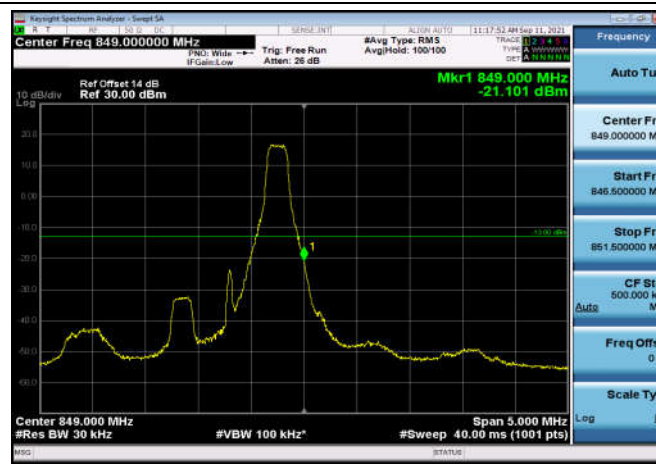
HighRange_FDD05_1.4MHz_848.3_OneRB _high_QPSK
