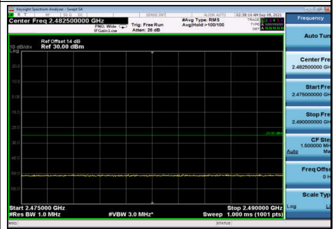
FDD07_10MHz_2505_Q16_fullRB_ExtraBand s_Range_2475~2490
