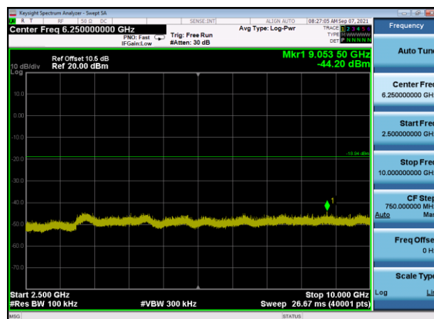
,Plot ,4Transmitter Spurious Emission : 2480,2500MHz~10000MHz
