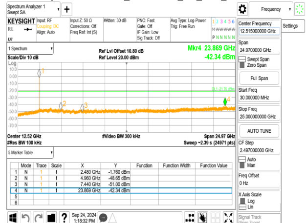
Spurious Emission_π/4QPSK_2M_DH5_2480MHz
