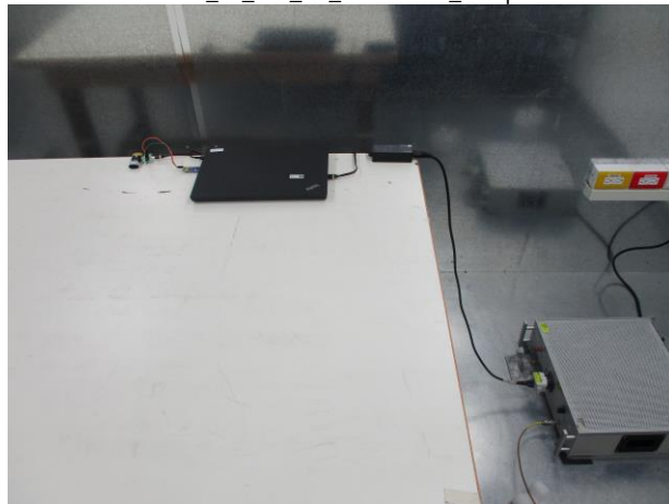
Part_15_247_BT_Conduction_Setup
