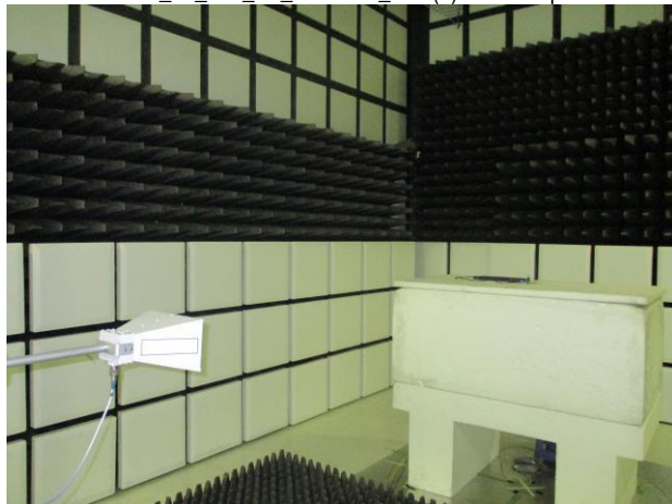
Part_15_247_LE_Radiated_966 (3).JPGSetup
