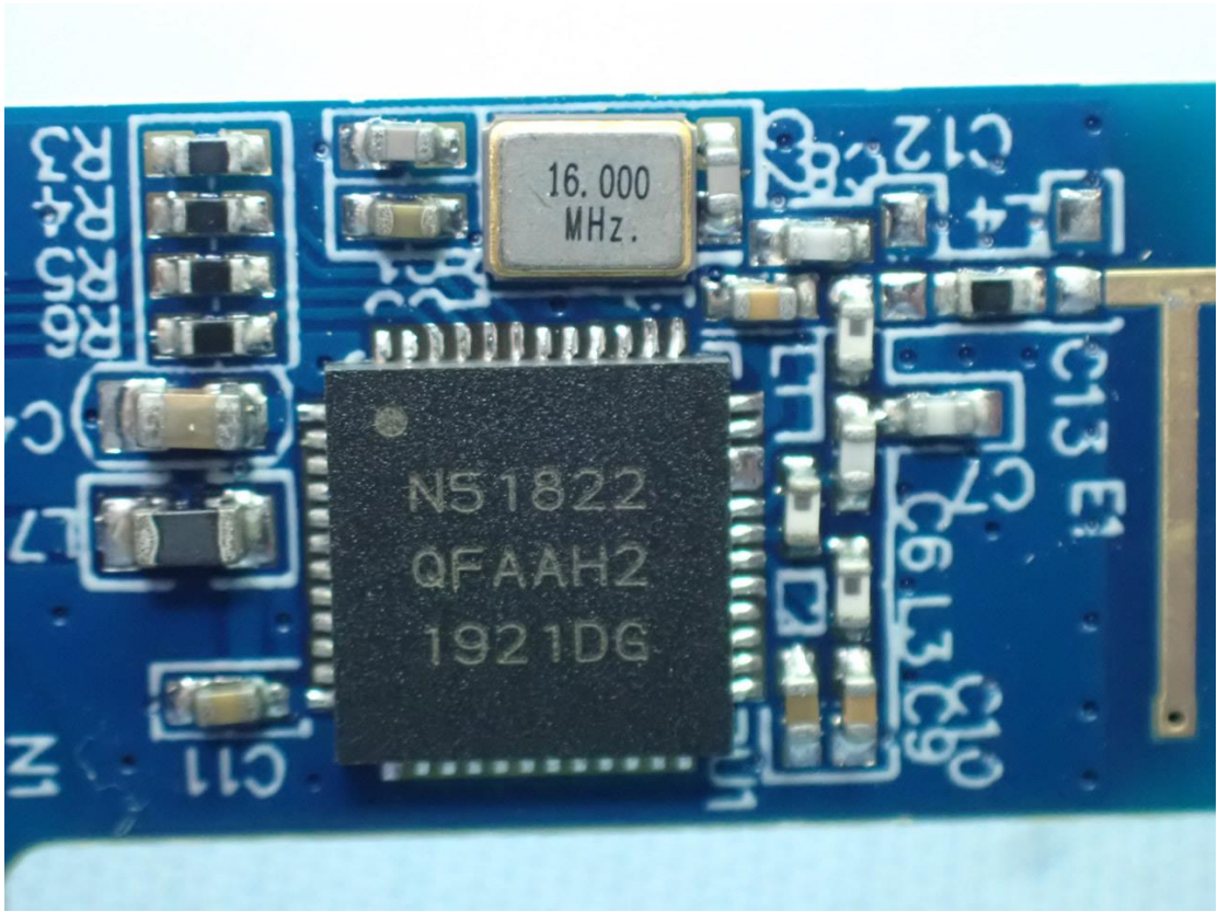
Figure 15 RF Chip View
