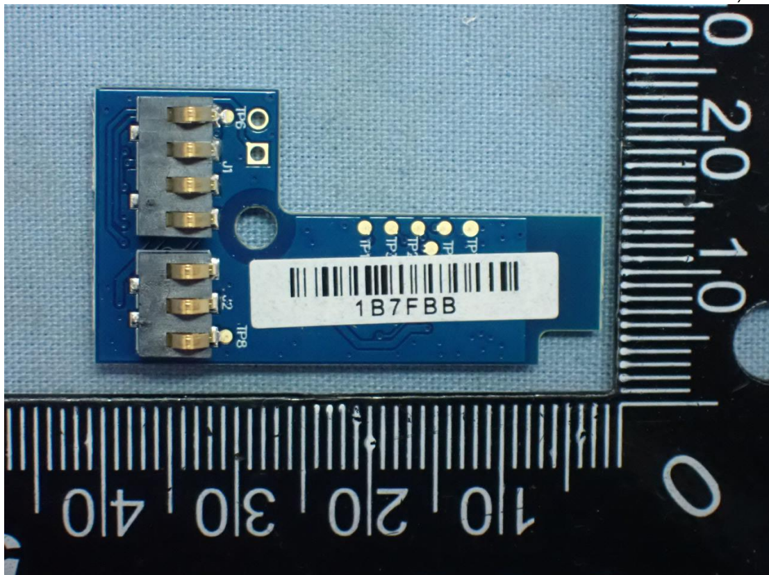
Bluetooth Module, Back View
