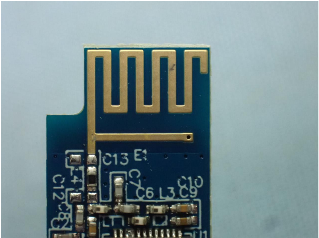
Figure 16 PCB Antenna View
