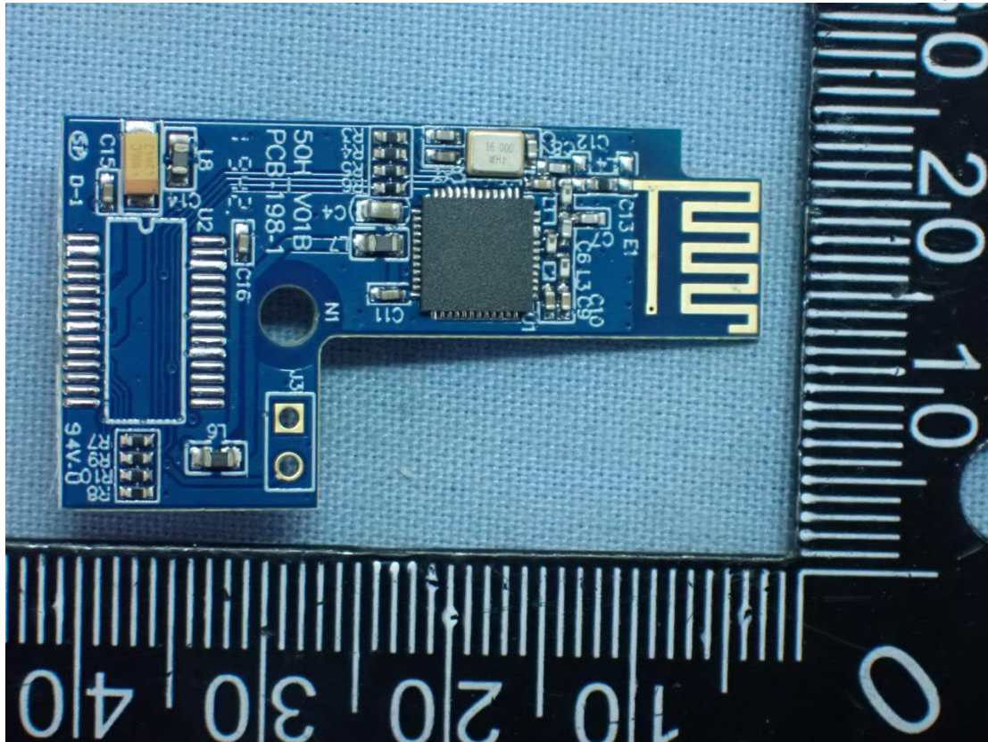
Bluetooth Module, Front View
