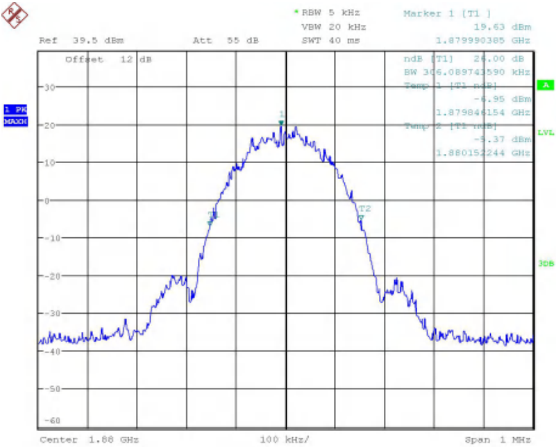
99% OBW-8PSK-Channel 661
