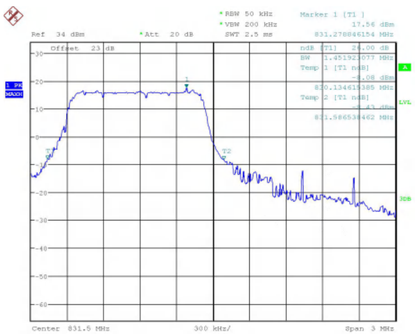
Band26-26dB OBW-3MHz Bandwidth-16QAM
