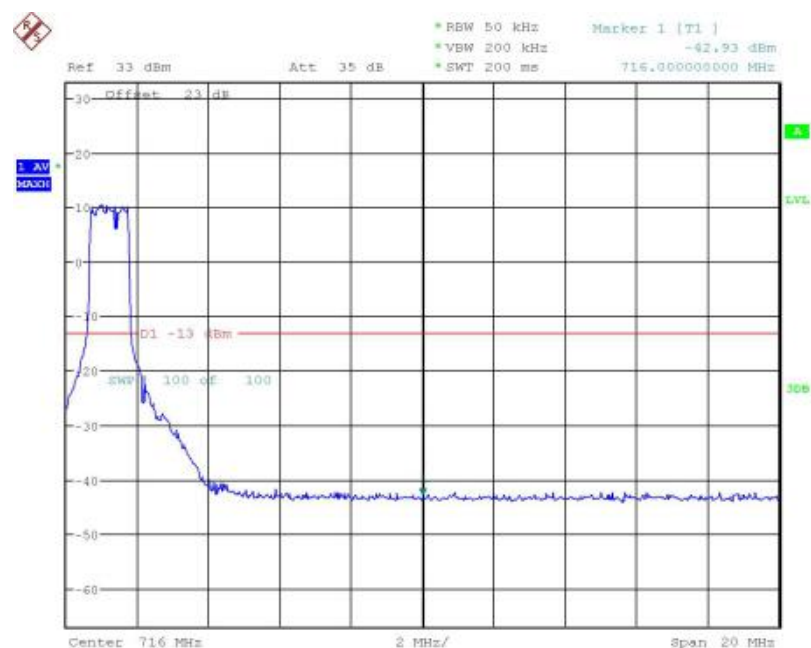
Band12-High Channel-10MHz Bandwidth-6RB-16QAM
