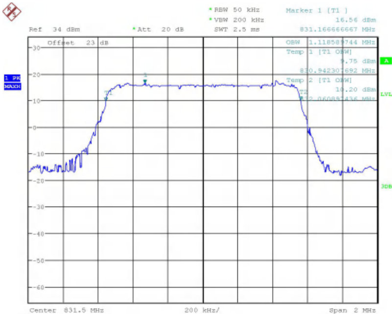
Band26-99% OBW-1.4MHz Bandwidth-16QAM
