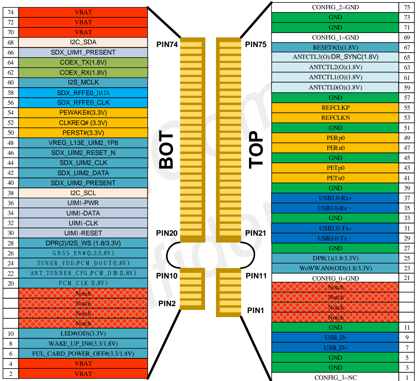
Figure 3: Pin assignment
