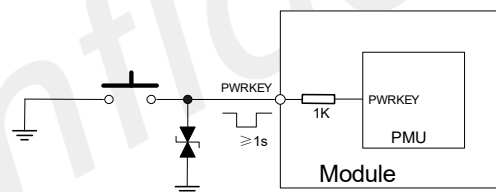
Figure 8: Power on the module use button
