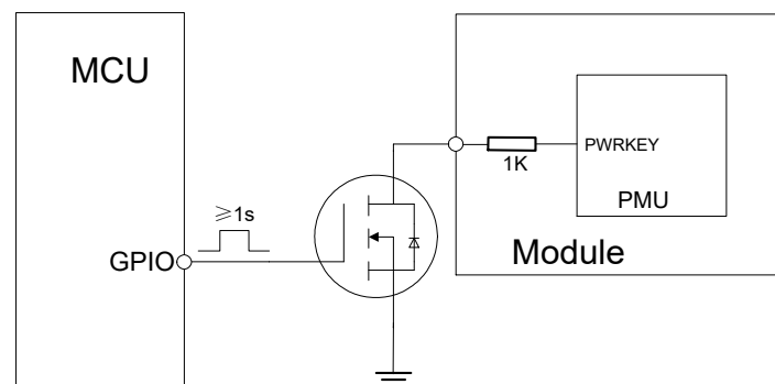
Figure 9: Power on the module use GPIO drive
