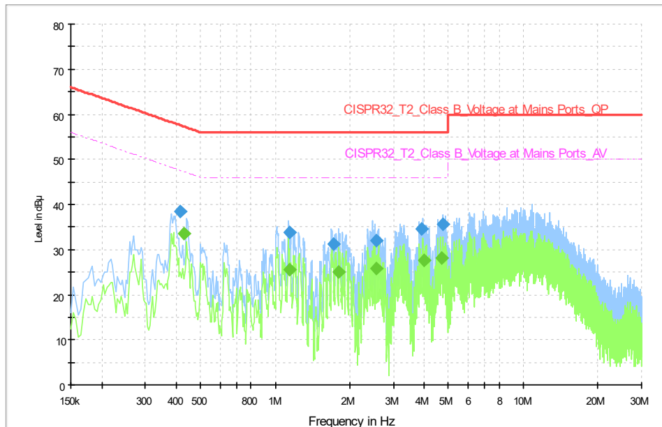
CISPR N&amp;L1 Voltage 150k to 30MHz-Class B
