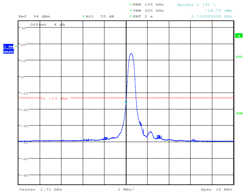
Band4-Low Channel-1.4MHz Bandwidth-1RB-16QAM
