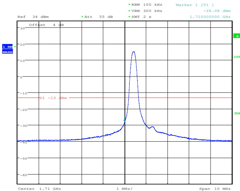
Band4-Low Channel-3MHz Bandwidth-1RB-16QAM
