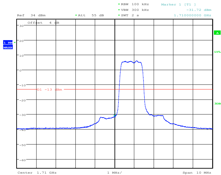
Band4-Low Channel-3MHz Bandwidth-5RB-16QAM
