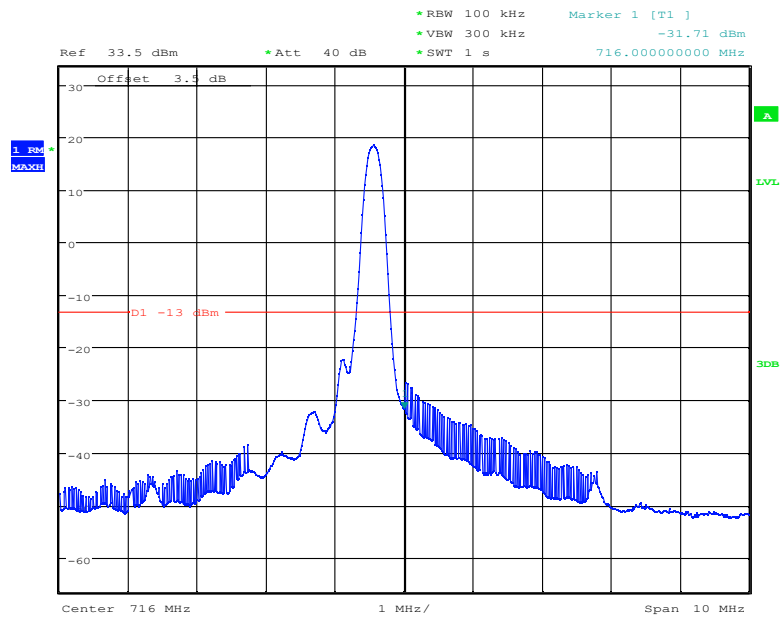
High Channel-5MHz Bandwidth-1RB-16QAM
