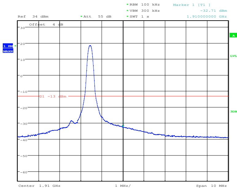
Band2-High Channel-20MHz Bandwidth-1RB-16QAM
