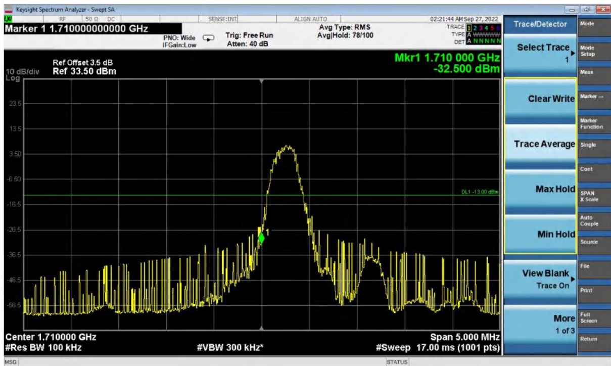
Band4-Low Channel-1.4MHz Bandwidth-1RB-QPSK
