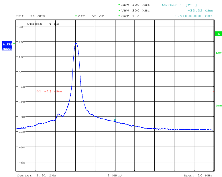
Band2-High Channel-10MHz Bandwidth-1RB-16QAM
