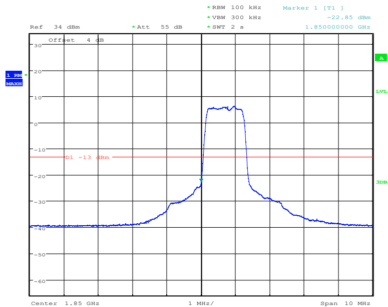
Band2-Low Channel-1.4MHz Bandwidth-5RB-16QAM
