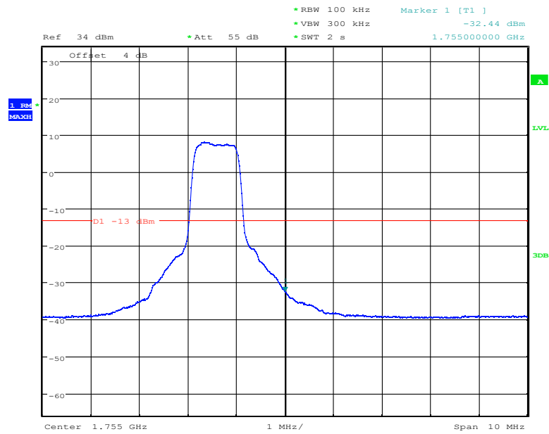
Band4-High Channel-10MHz Bandwidth-5RB-16QAM
