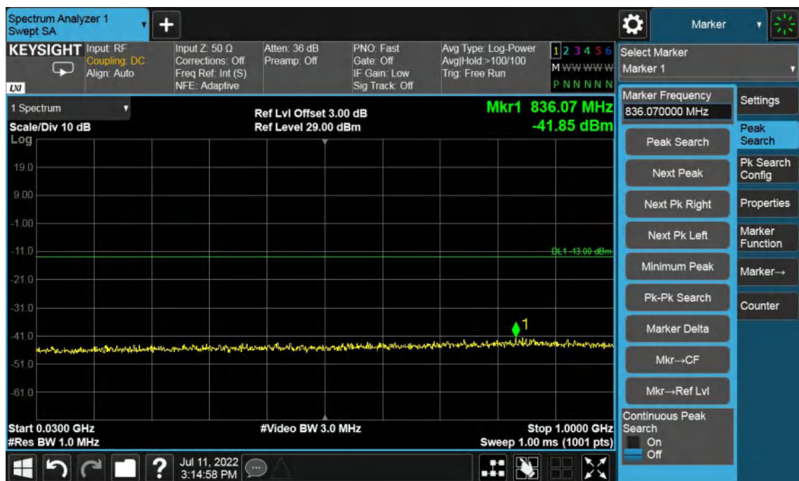
Band2-Low Channel-20MHz Bandwidth-30MHz to 1GHz
