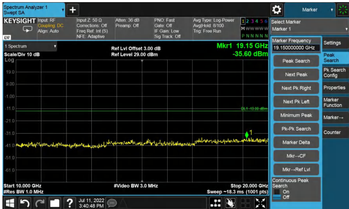
Band2-High Channel-15MHz Bandwidth-10GHz to 20GHz
