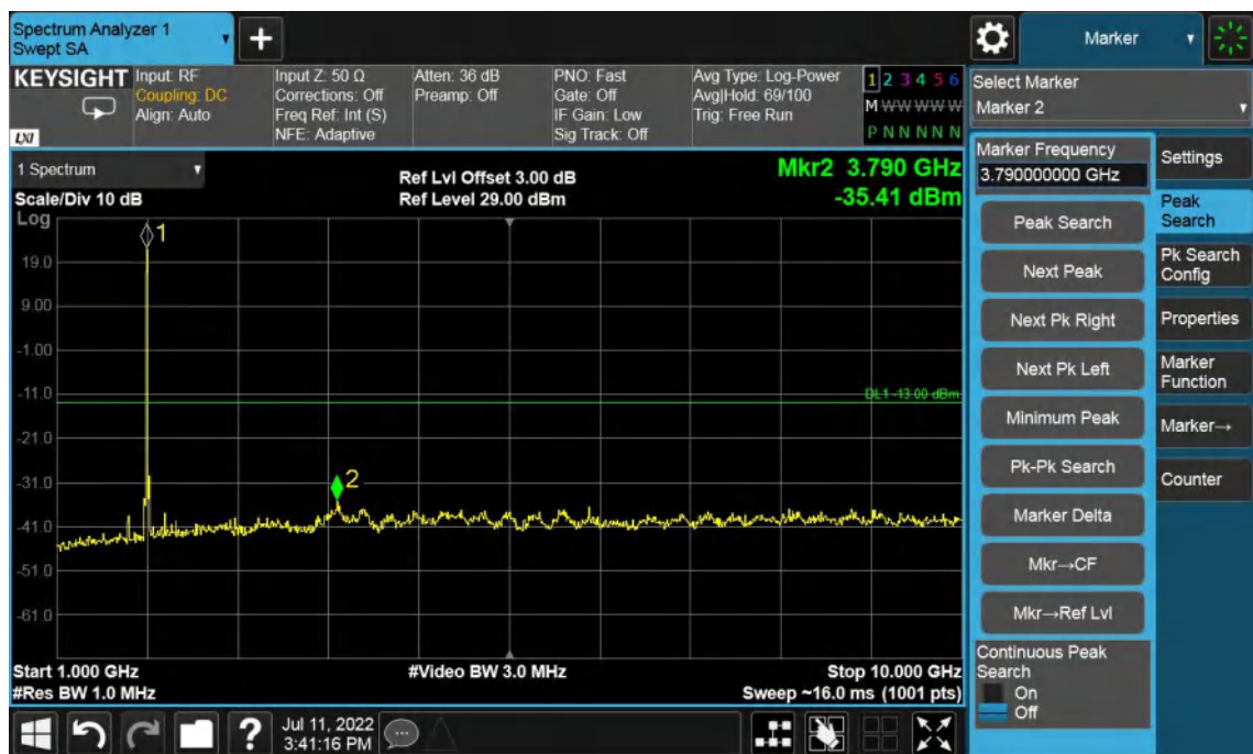
Band2-High Channel-15MHz Bandwidth-1GHz to 10GHz
