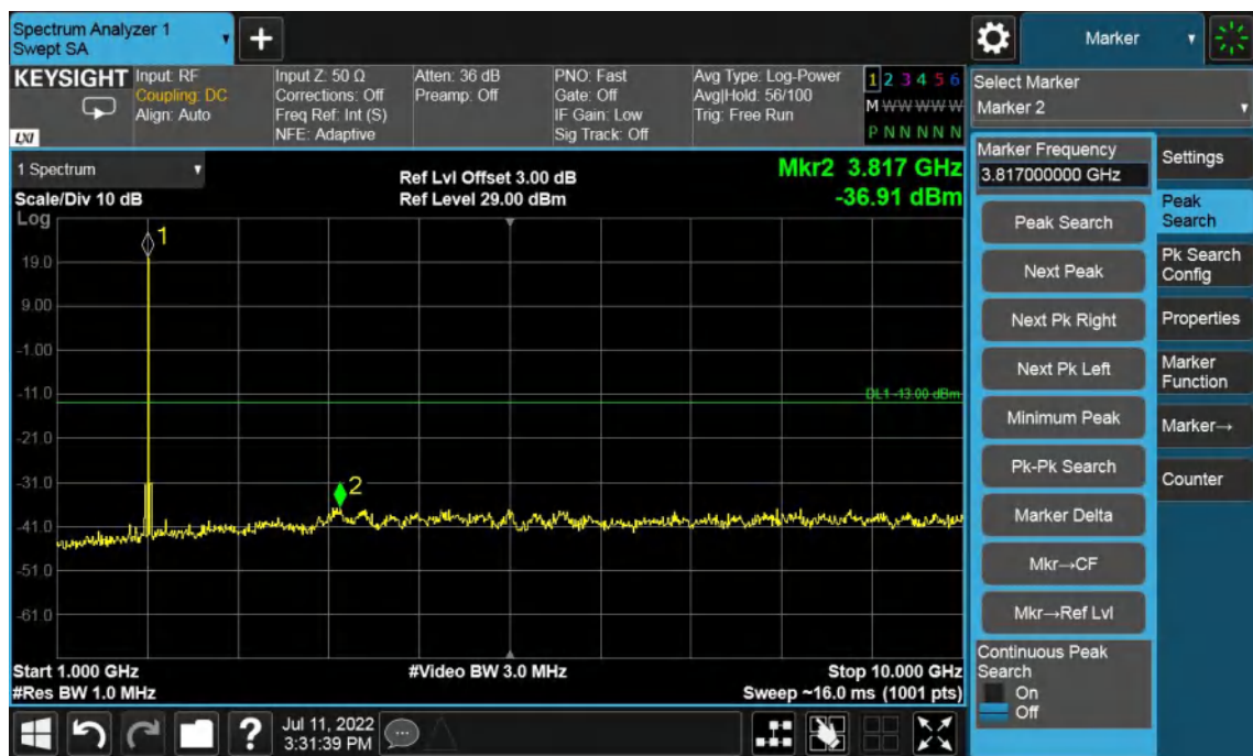
Band2-High Channel-1.4MHz Bandwidth-1GHz to 10GHz
