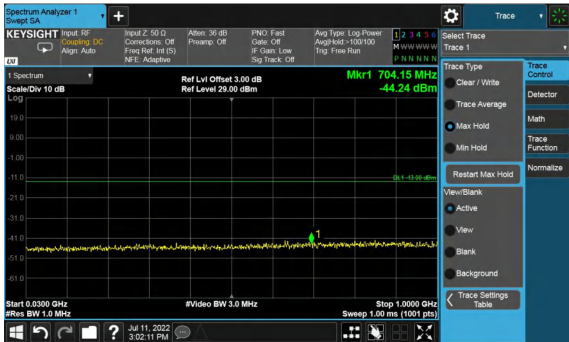
Band2-Low Channel-5MHz Bandwidth-30MHz to 1GHz
