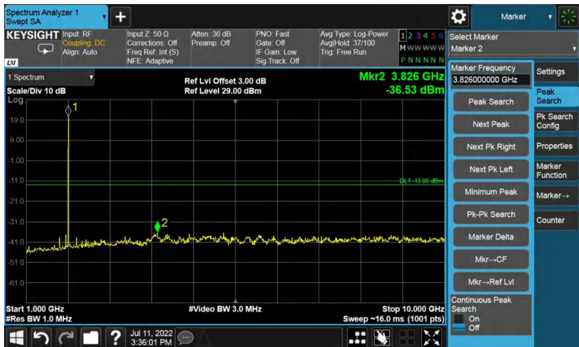
Band2-High Channel-5MHz Bandwidth-1GHz to 10GHz
