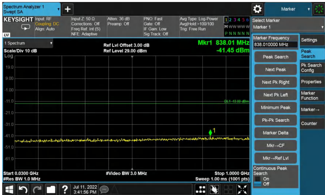
Band2-High Channel-15MHz Bandwidth-30MHz to 1GHz
