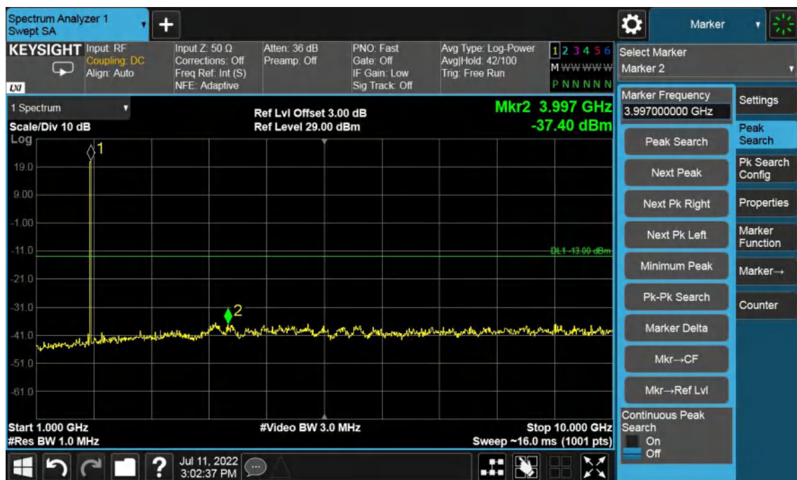
Band2-Low Channel-5MHz Bandwidth-1GHz to 10GHz
