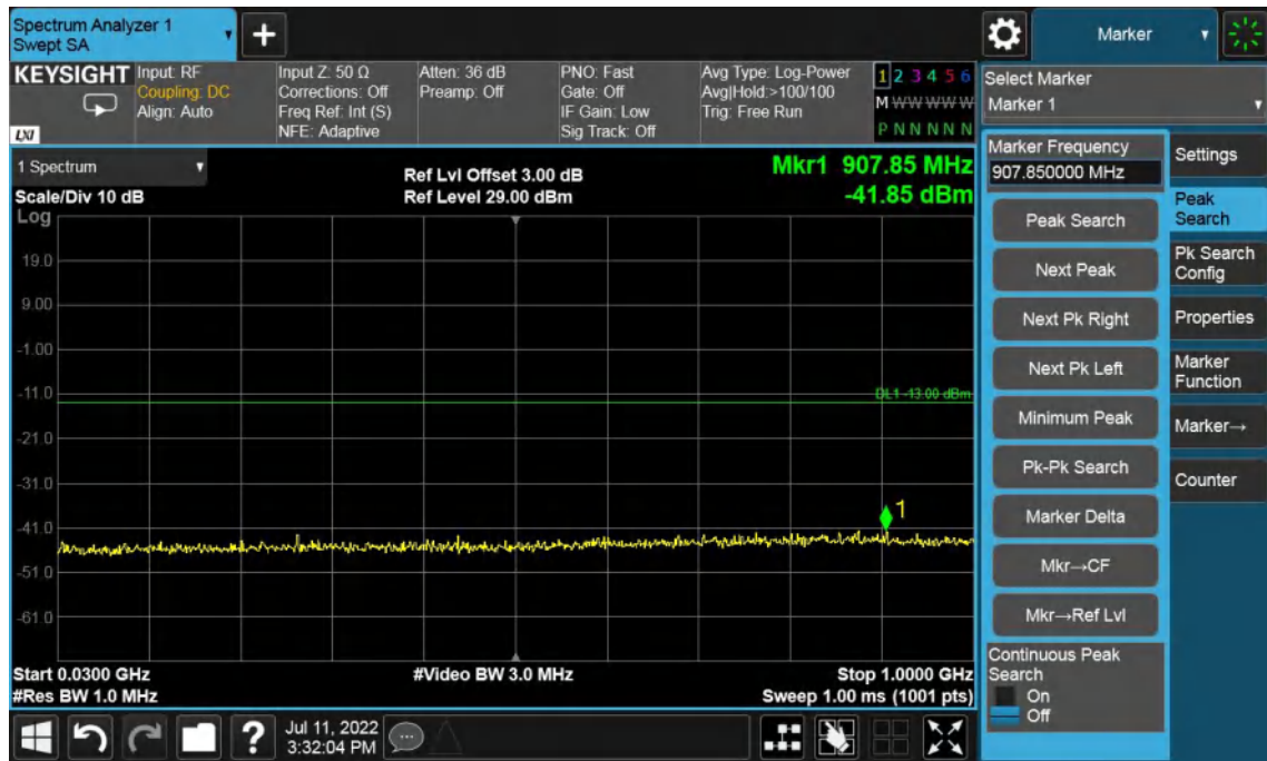
Band2-High Channel-1.4MHz Bandwidth-30MHz to 1GHz
