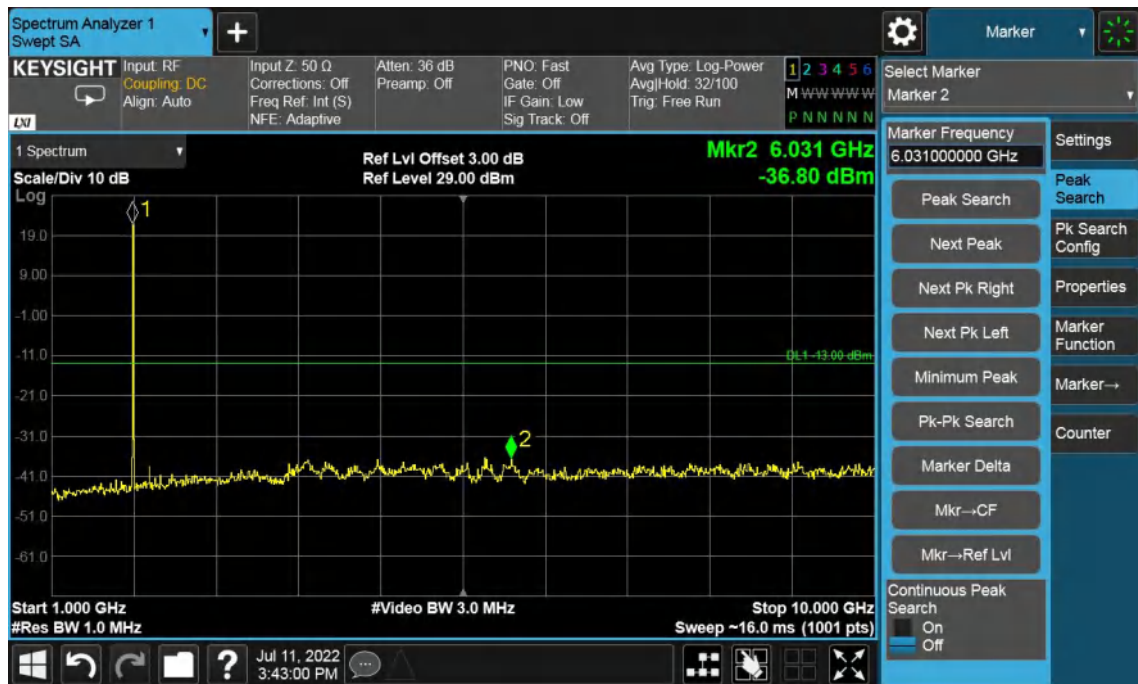
Band2-High Channel-20MHz Bandwidth-1GHz to 10GHz
