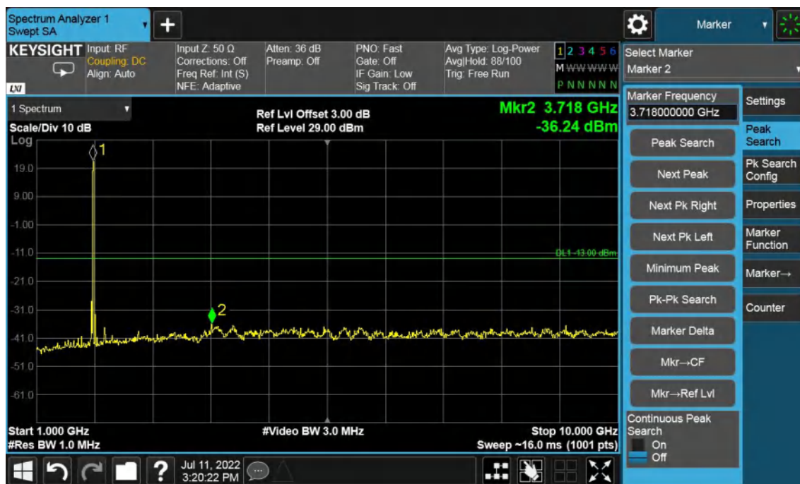
Band2-Middle Channel-5MHz Bandwidth-1GHz to 10GHz
