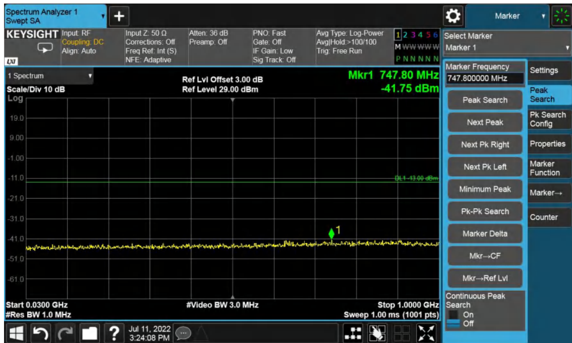
Band2-Middle Channel-15MHz Bandwidth-30MHz to 1GHz
