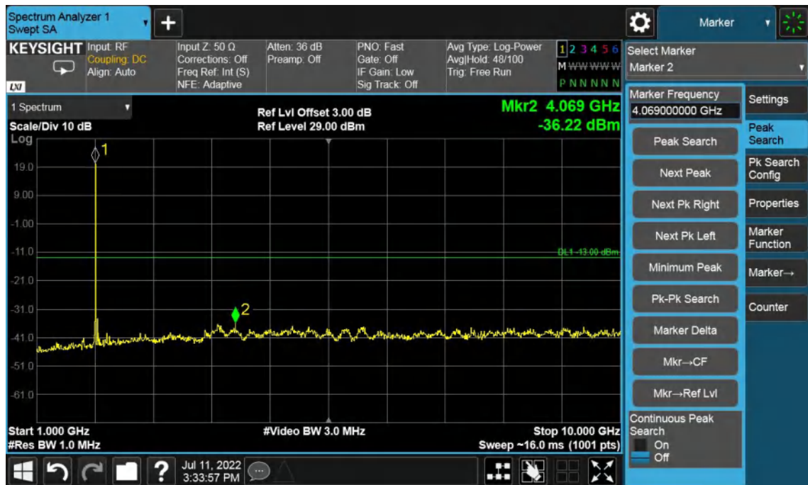
Band2-High Channel-3MHz Bandwidth-1GHz to 10GHz
