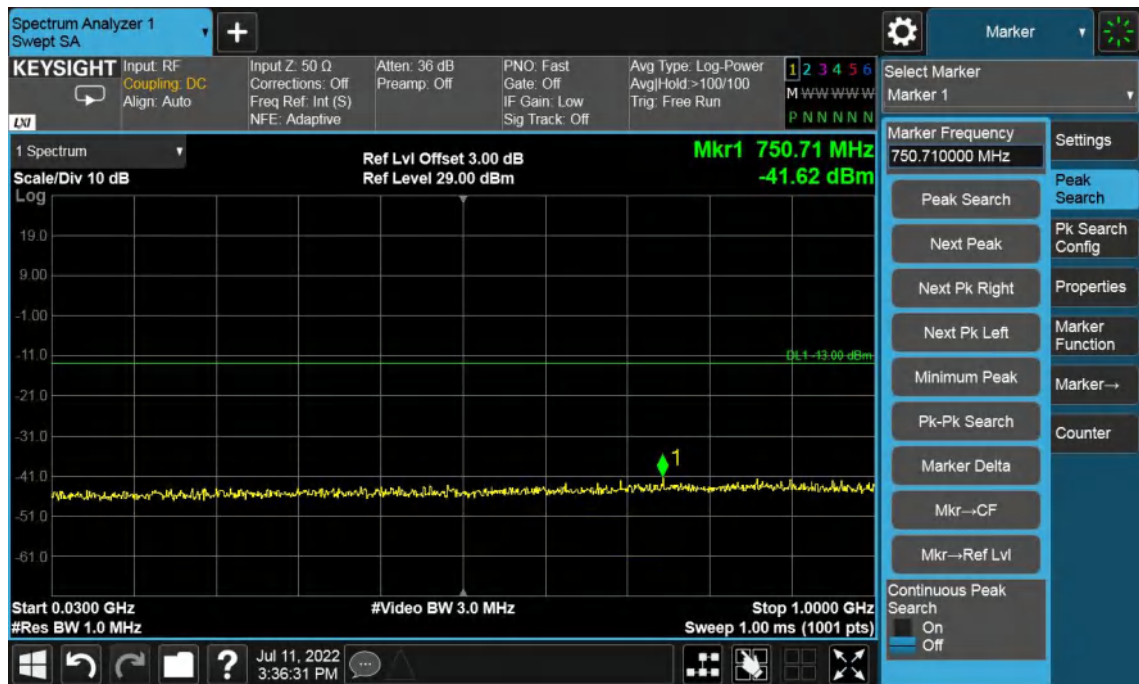
Band2-High Channel-5MHz Bandwidth-30MHz to 1GHz
