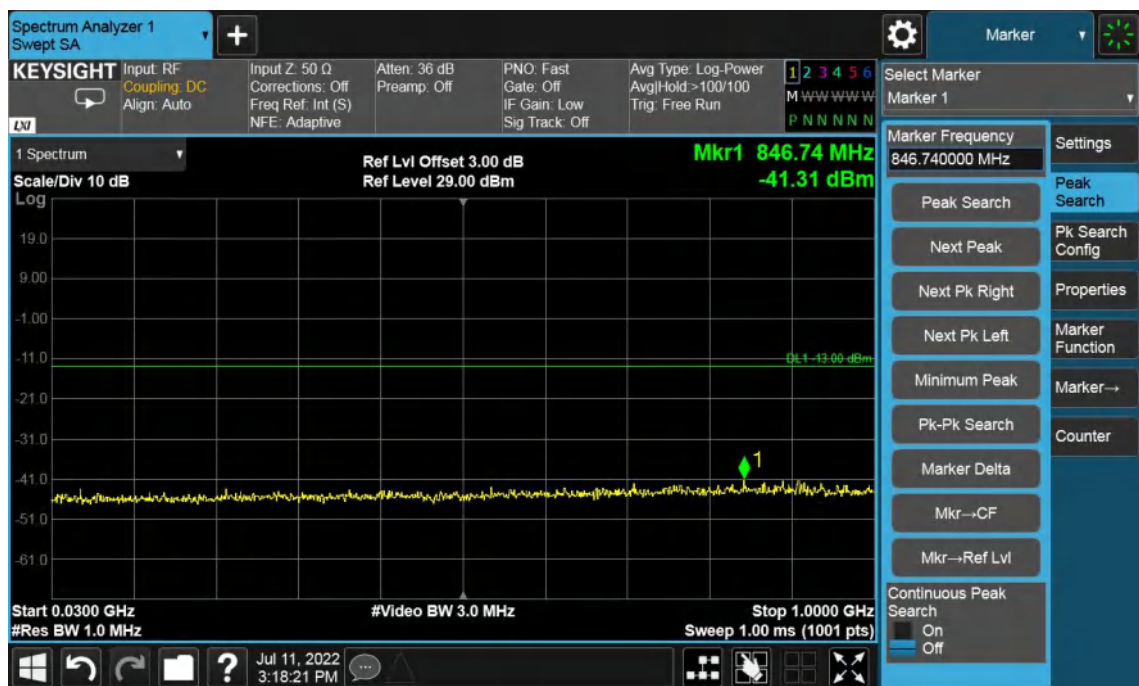
Band2-Middle Channel-3MHz Bandwidth-30MHz to 1GHz
