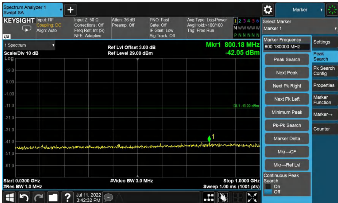
Band2-High Channel-20MHz Bandwidth-30MHz to 1GHz
