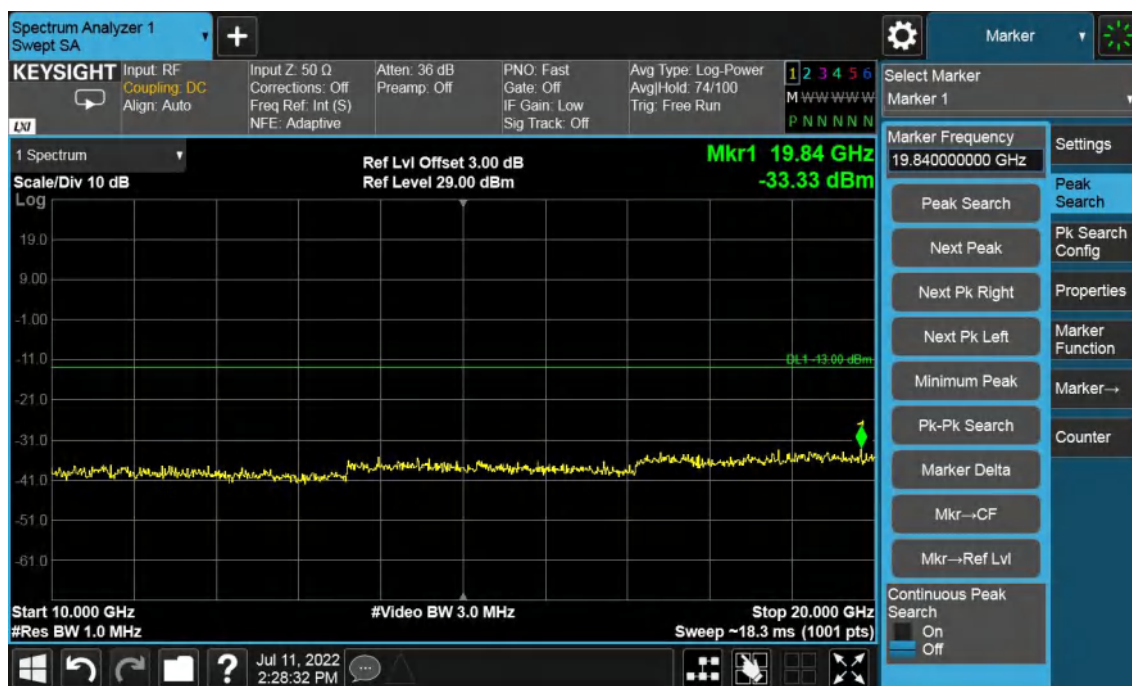
Band2-Low Channel-1.4MHz Bandwidth-10GHz to 20GHz
