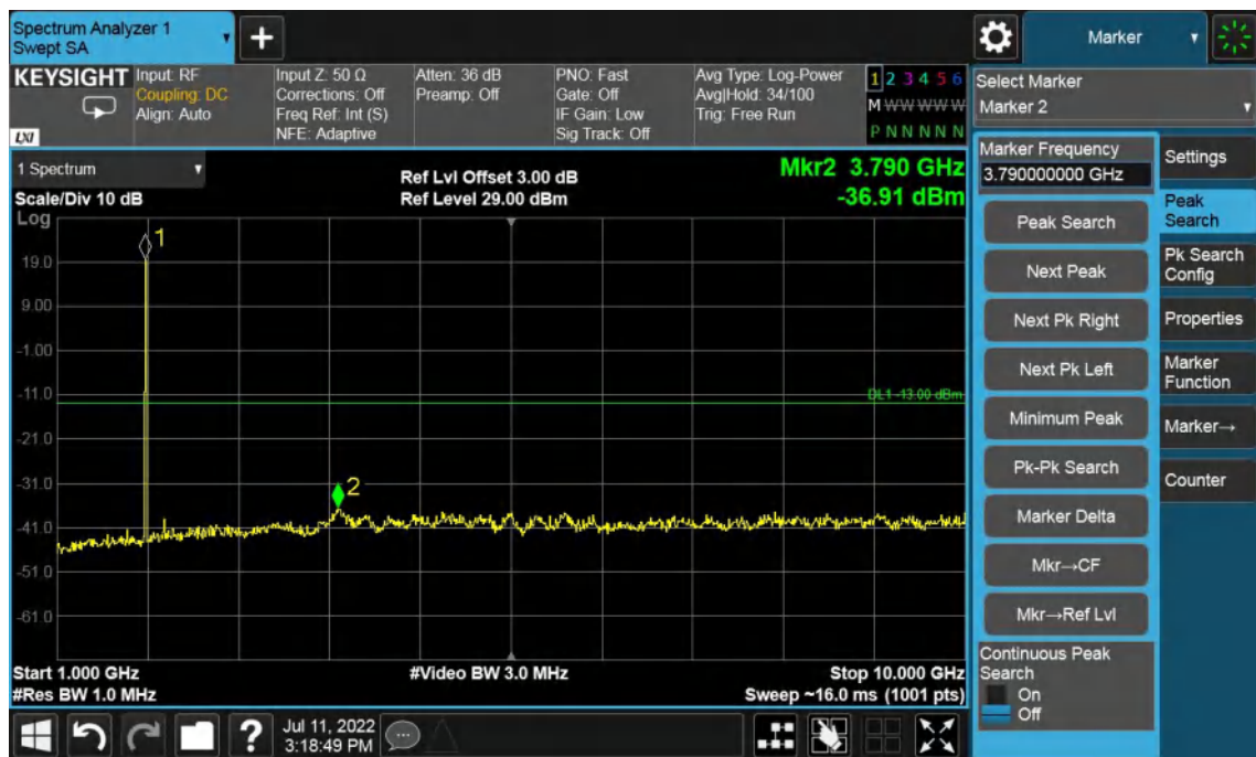
Band2-Middle Channel-3MHz Bandwidth-1GHz to 10GHz
