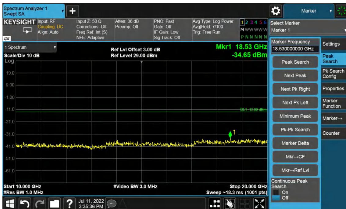
Band2-High Channel-5MHz Bandwidth-10GHz to 20GHz
