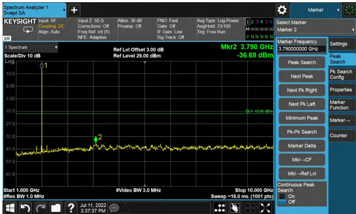
Band2-High Channel-10MHz Bandwidth-1GHz to 10GHz
