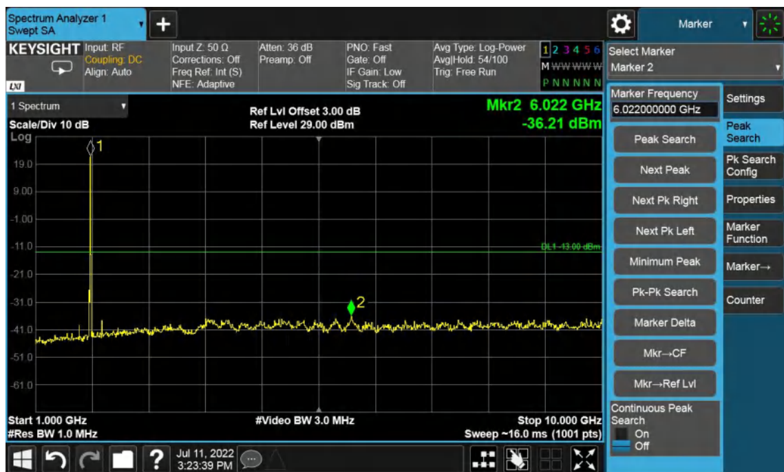
Band2-Middle Channel-15MHz Bandwidth-1GHz to 10GHz
