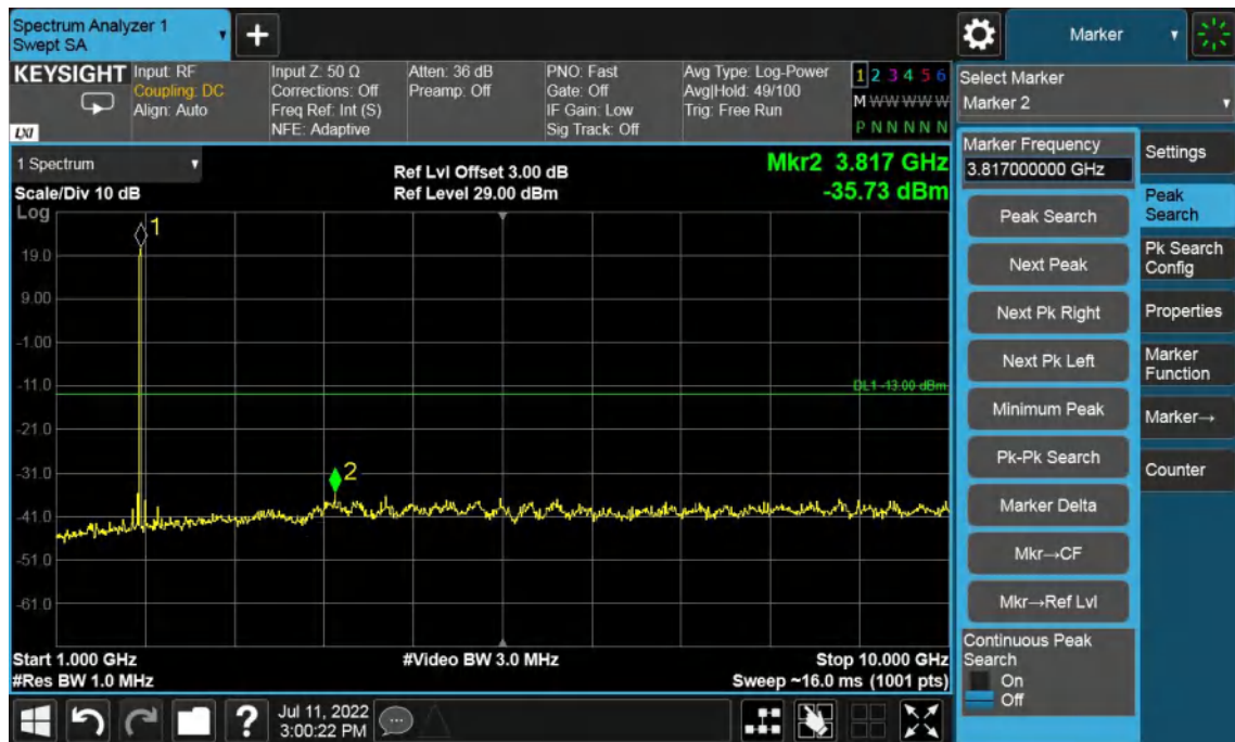
Band2-Low Channel-3MHz Bandwidth-1GHz to 10GHz
