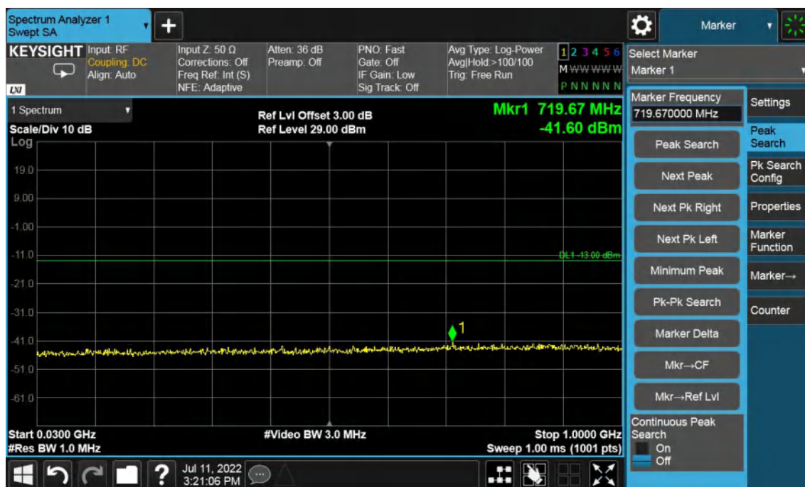
Band2-Middle Channel-5MHz Bandwidth-30MHz to 1GHz
