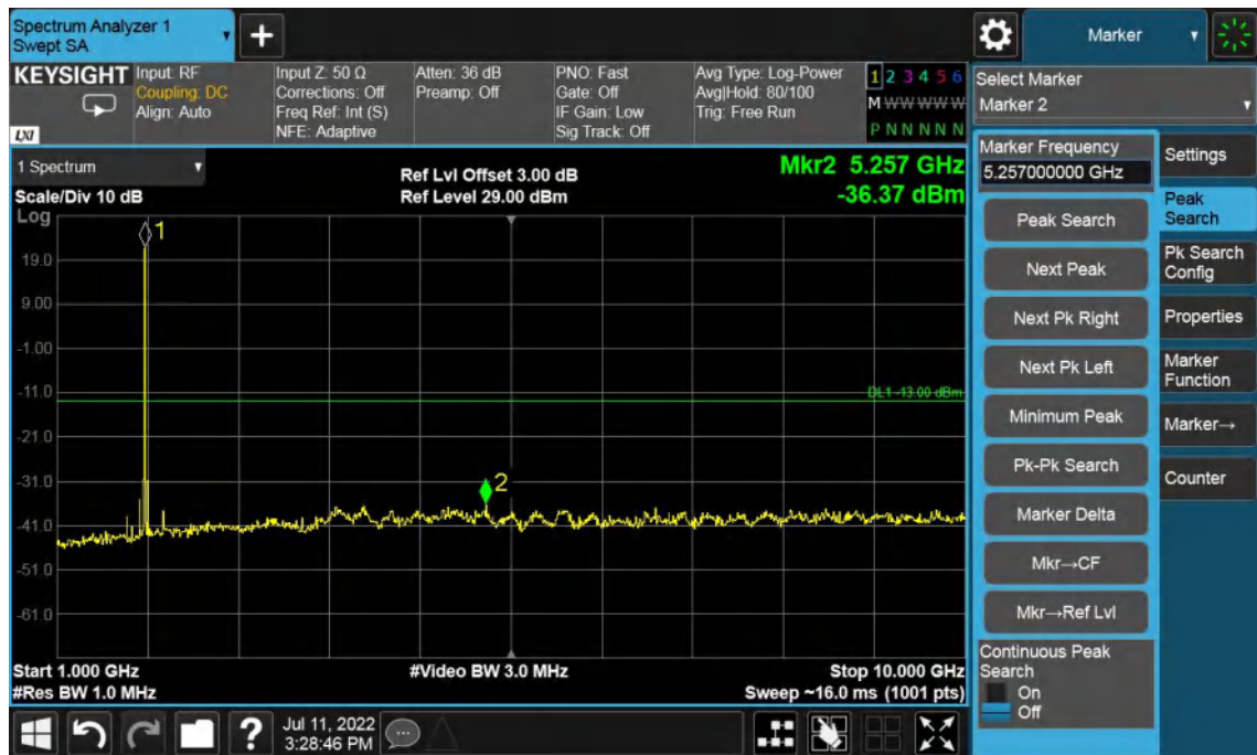
Band2-Middle Channel-20MHz Bandwidth-1GHz to 10GHz
