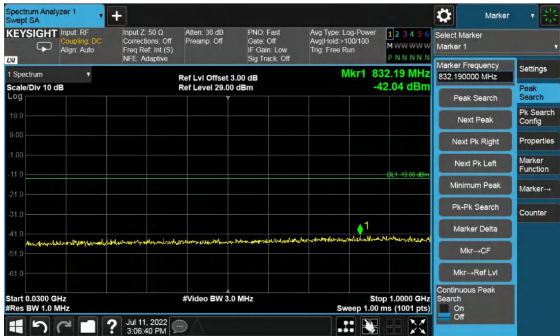
Band2-Low Channel-15MHz Bandwidth-30MHz to 1GHz
