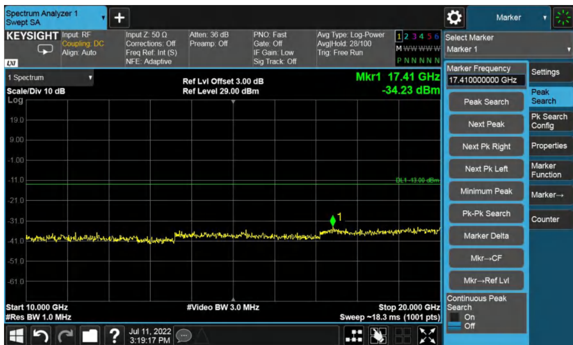
Band2-Middle Channel-3MHz Bandwidth-10GHz to 20GHz
