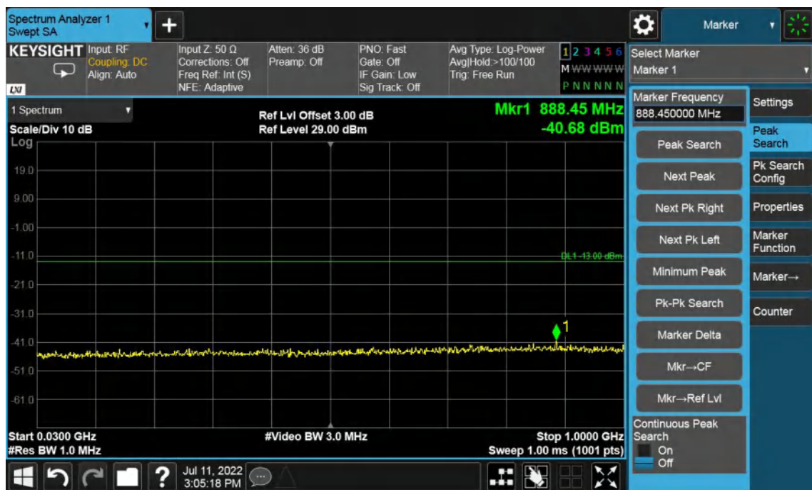
Band2-Low Channel-10MHz Bandwidth-30MHz to 1GHz
