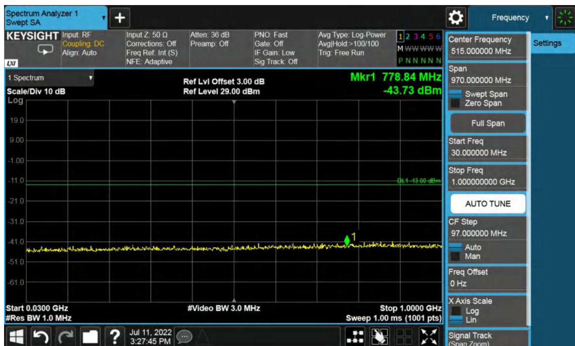
Band2-Middle Channel-20MHz Bandwidth-30MHz to 1GHz
