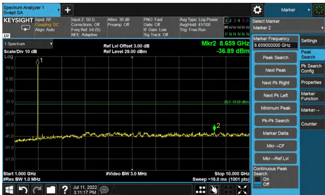
Band2-Middle Channel-1.4MHz Bandwidth-1GHz to 10GHz
