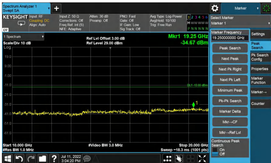
Band2-Low Channel-10MHz Bandwidth-10GHz to 20GHz
