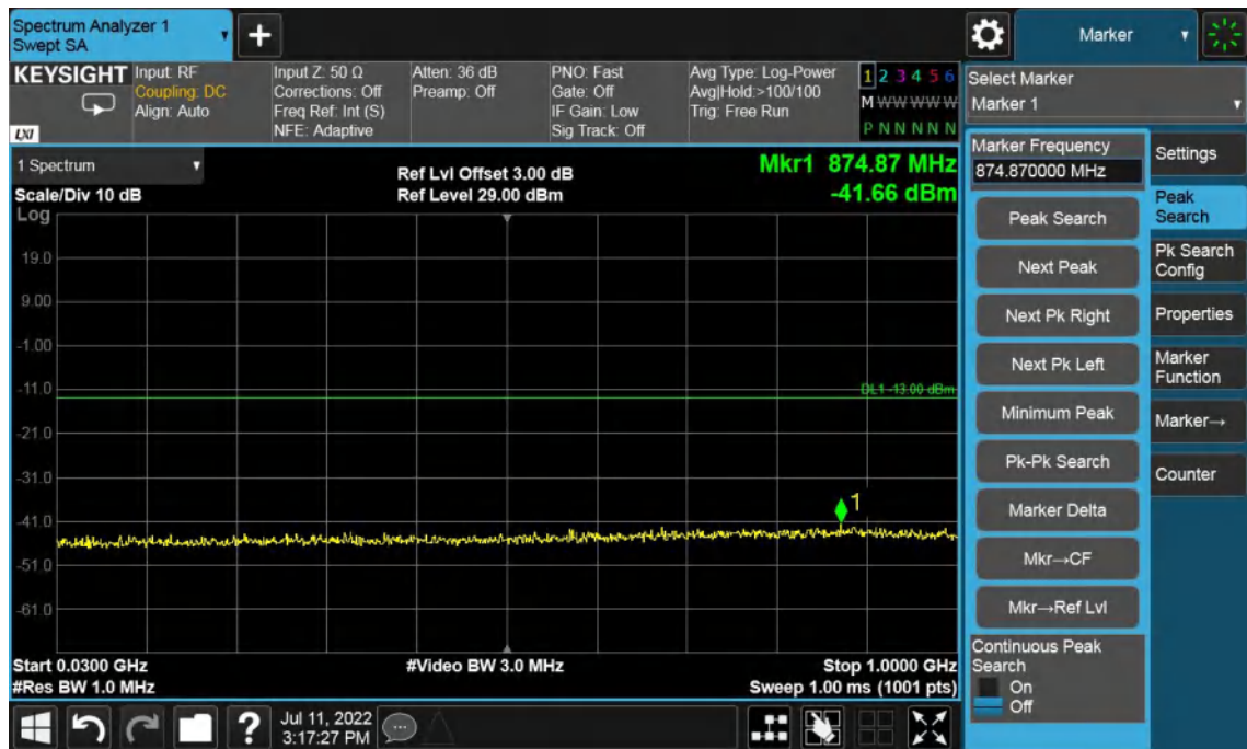
Band2-Middle Channel-1.4MHz Bandwidth-30MHz to 1GHz
