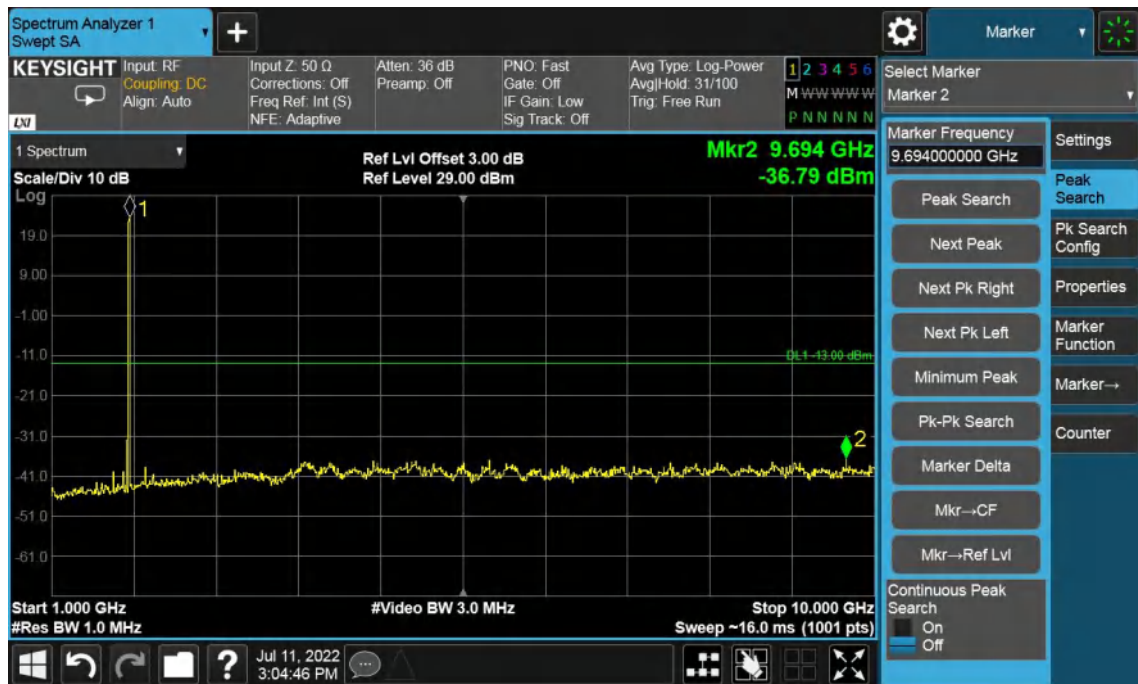
Band2-Low Channel-10MHz Bandwidth-1GHz to 10GHz
