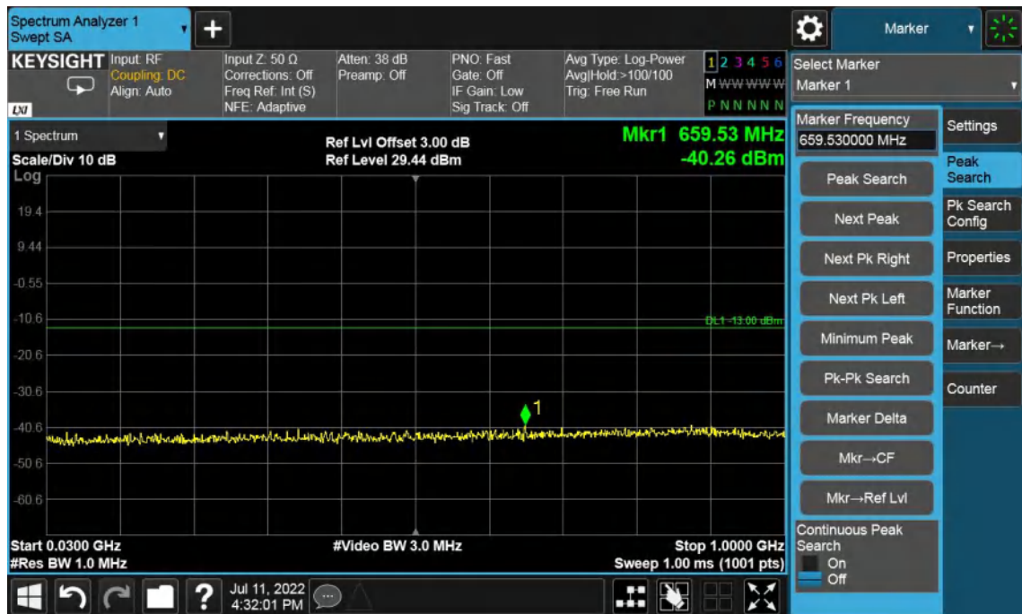
Band4-High Channel-15MHz Bandwidth-30MHz to 1GHz
