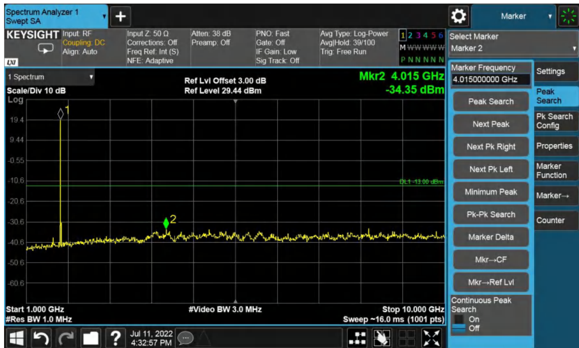
Band4-High Channel-20MHz Bandwidth-1GHz to 10GHz
