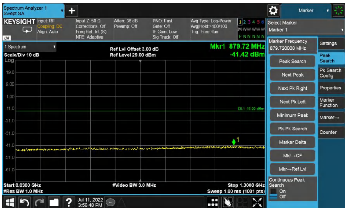
Band4-Low Channel-20MHz Bandwidth-30MHz to 1GHz
