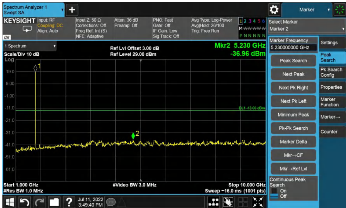
Band4-Low Channel-3MHz Bandwidth-1GHz to 10GHz
