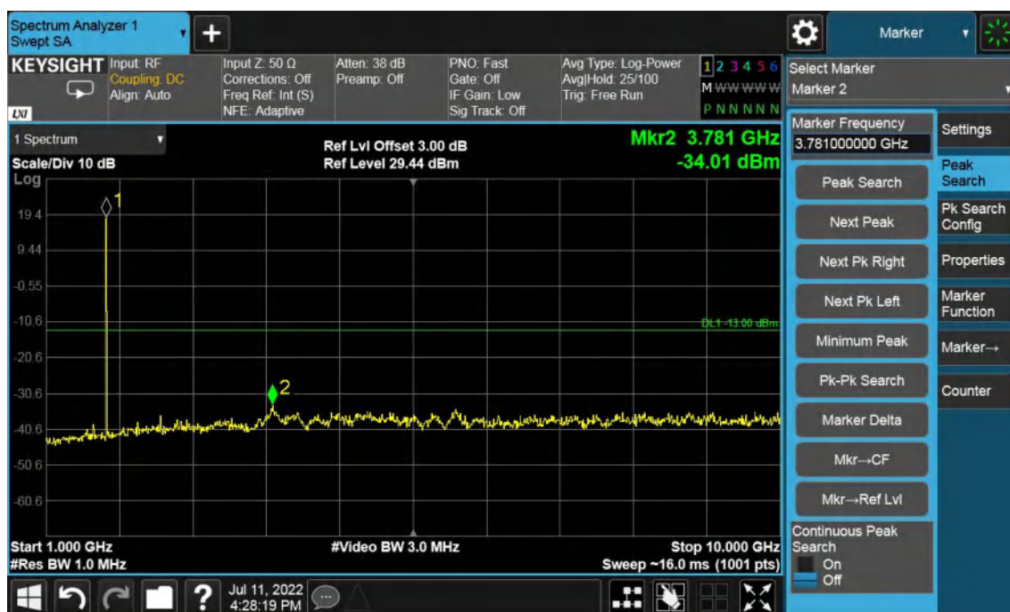
Band4-High Channel-5MHz Bandwidth-1GHz to 10GHz
