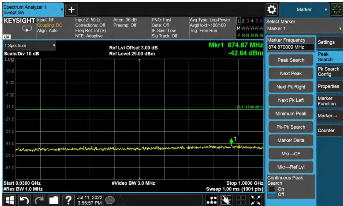
Band4-Low Channel-15MHz Bandwidth-30MHz to 1GHz
