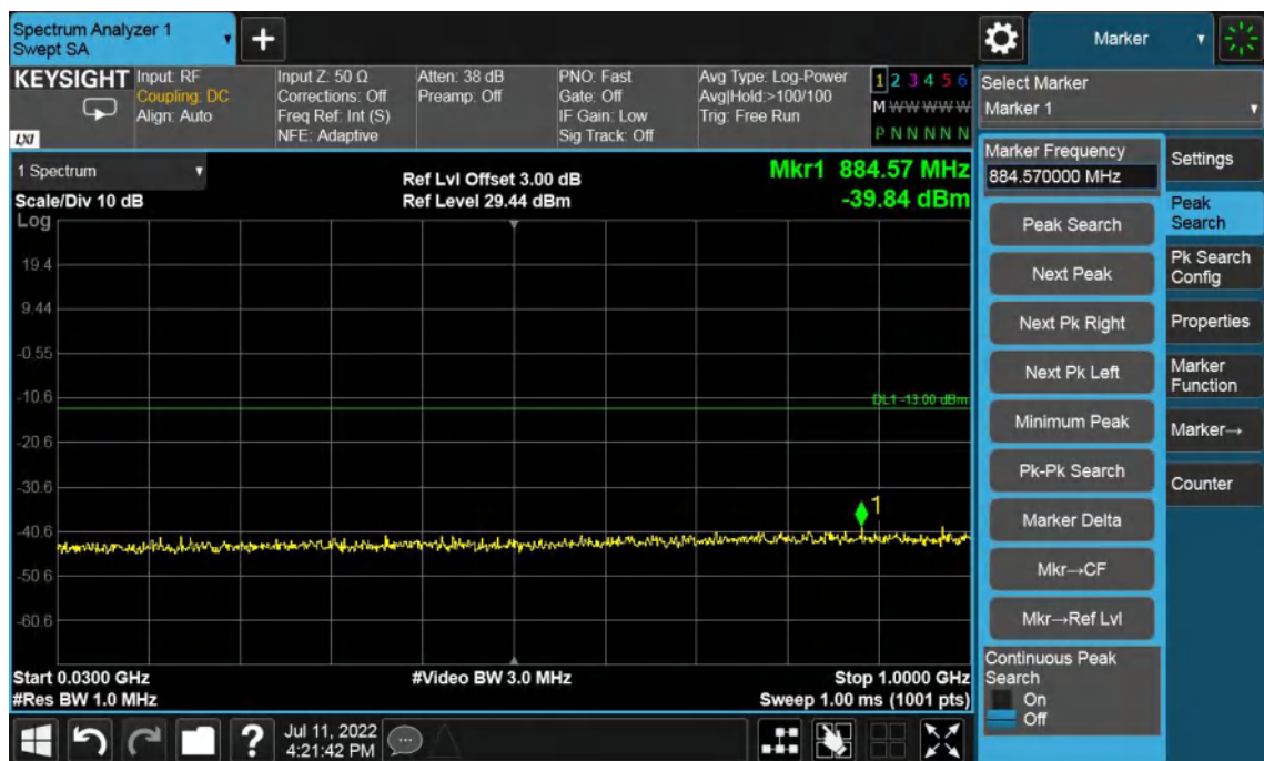
Band4-High Channel-3MHz Bandwidth-30MHz to 1GHz
