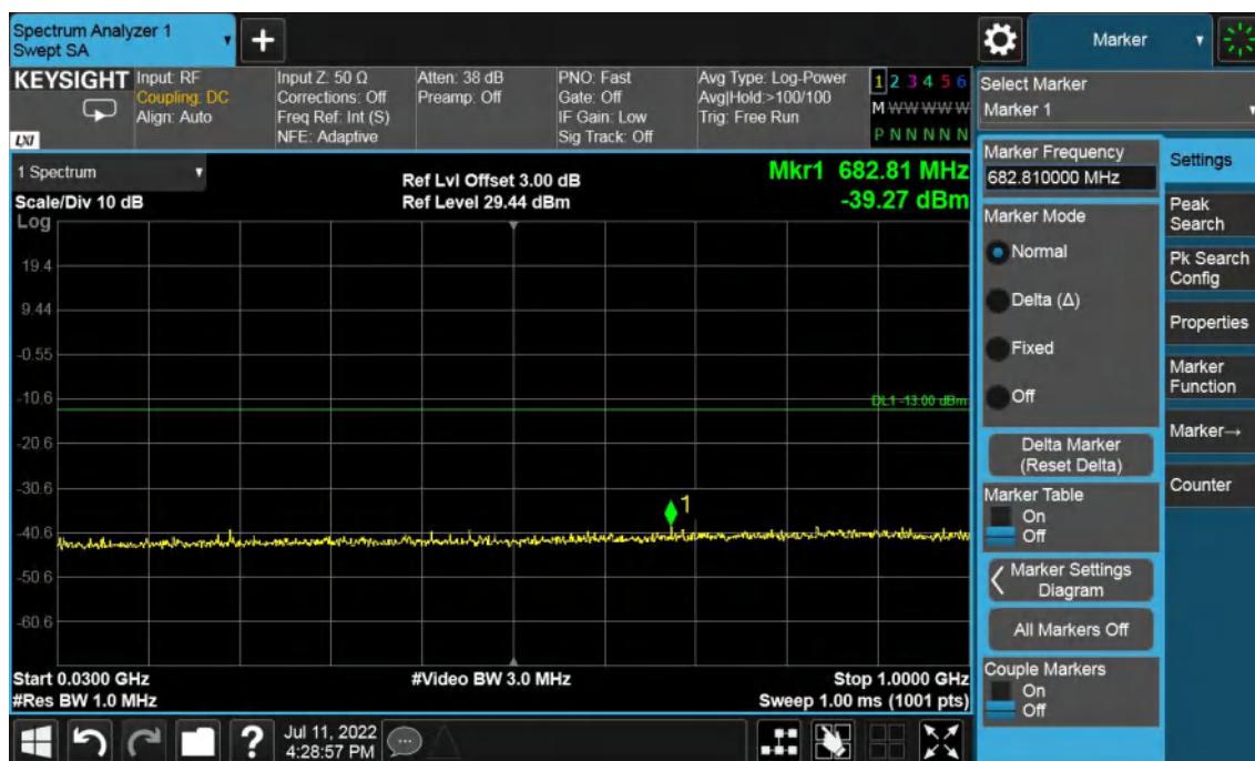
Band4-High Channel-5MHz Bandwidth-30MHz to 1GHz
