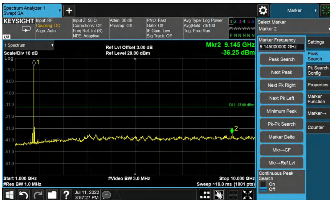
Band4-Low Channel-20MHz Bandwidth-1GHz to 10GHz
