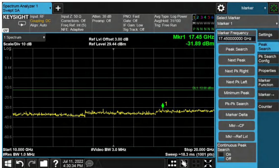
Band4-High Channel-10MHz Bandwidth-10GHz to 20GHz
