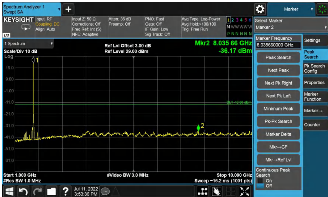
Band4-Low Channel-10MHz Bandwidth-1GHz to 10GHz
