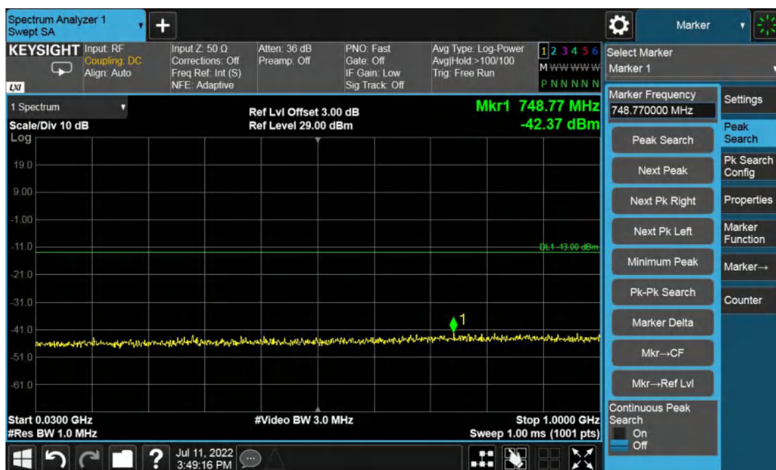
Band4-Low Channel-3MHz Bandwidth-30MHz to 1GHz
