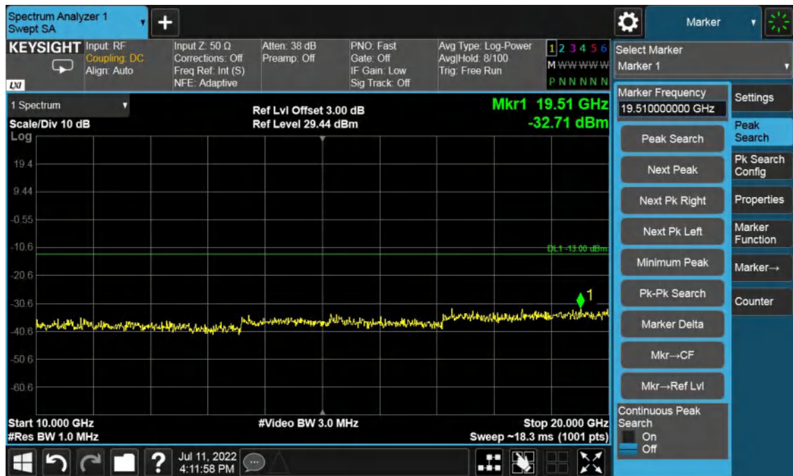
Band4-Middle Channel-5MHz Bandwidth-10GHz to 20GHz
