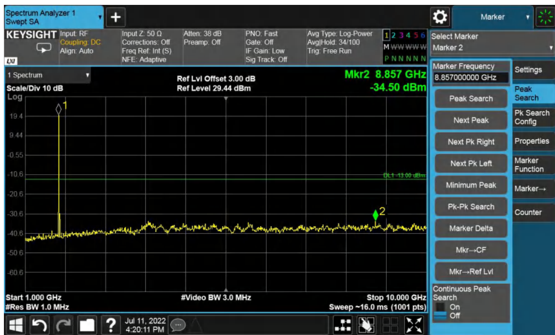
Band4-High Channel-1.4MHz Bandwidth-1GHz to 10GHz
