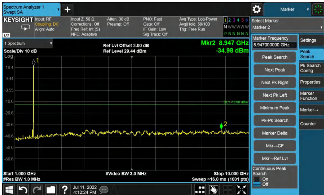
Band4-Middle Channel-5MHz Bandwidth-1GHz to 10GHz
