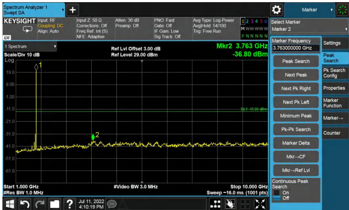
Band4-Middle Channel-3MHz Bandwidth-1GHz to 10GHz
