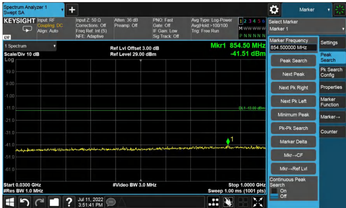
Band4-Low Channel-5MHz Bandwidth-30MHz to 1GHz
