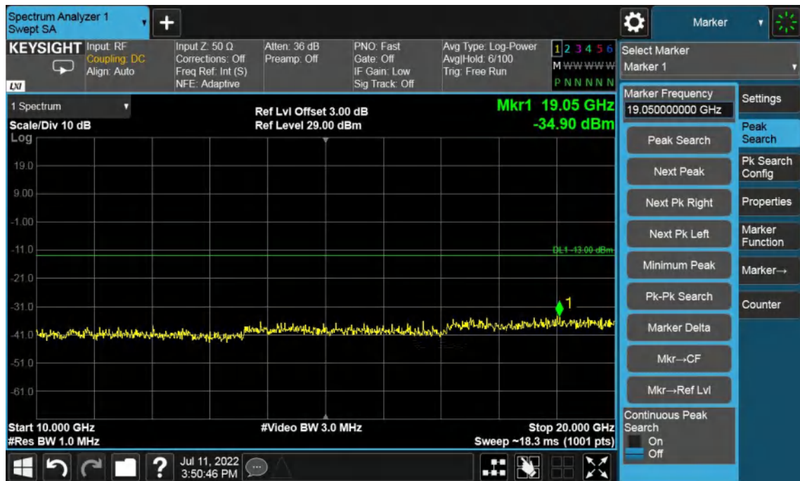
Band4-Low Channel-5MHz Bandwidth-10GHz to 20GHz
