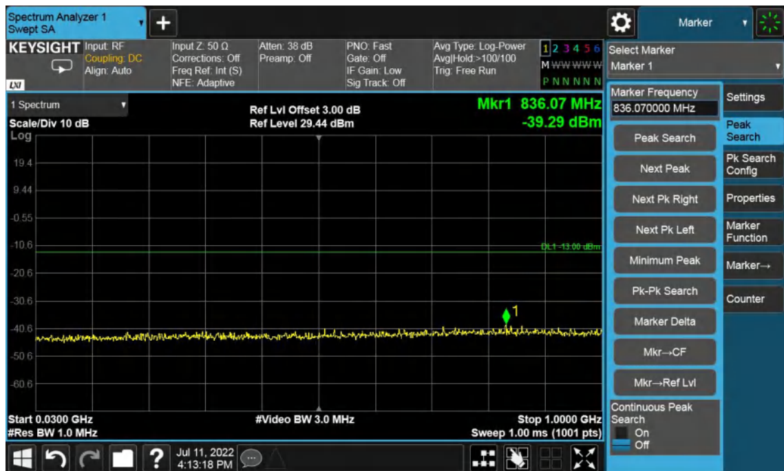
Band4-Middle Channel-10MHz Bandwidth-30MHz to 1GHz
