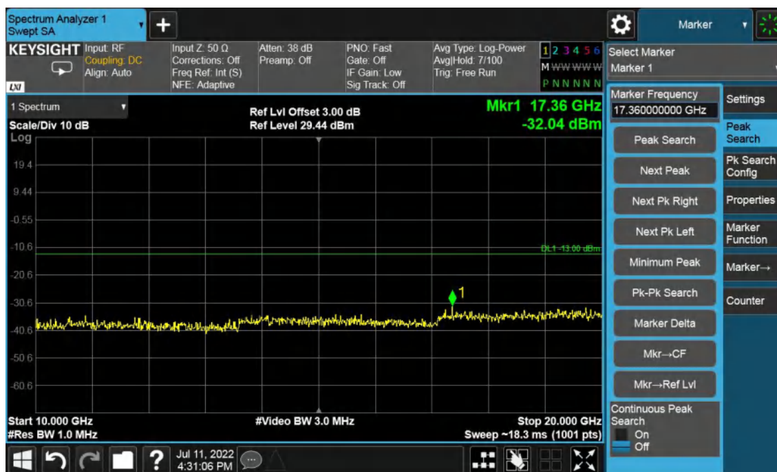
Band4-High Channel-15MHz Bandwidth-10GHz to 20GHz
