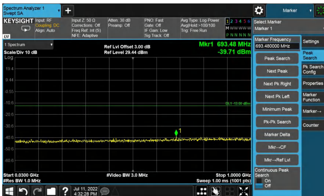
Band4-High Channel-20MHz Bandwidth-30MHz to 1GHz
