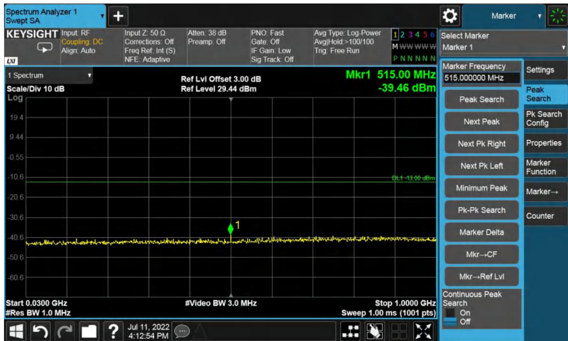
Band4-Middle Channel-5MHz Bandwidth-30MHz to 1GHz
