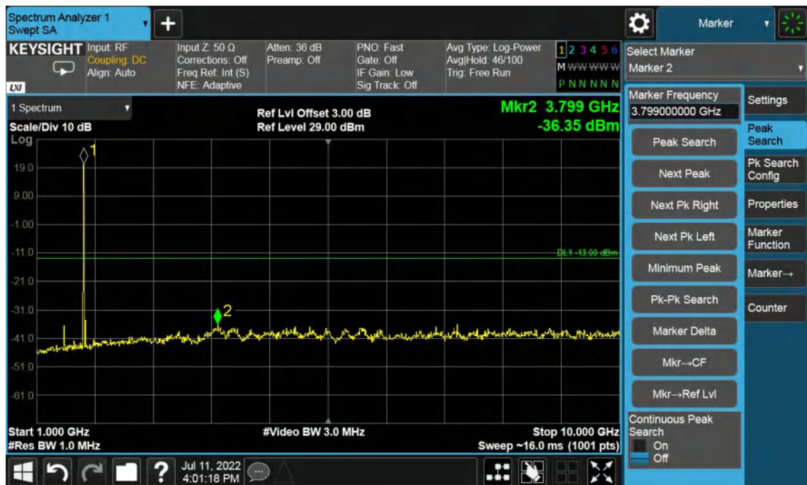
Band4-Middle Channel-1.4MHz Bandwidth-1GHz to 10GHz
