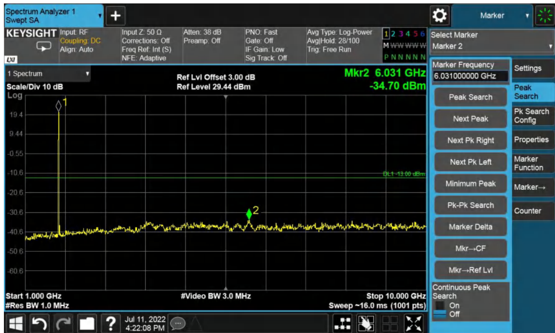
Band4-High Channel-3MHz Bandwidth-1GHz to 10GHz
