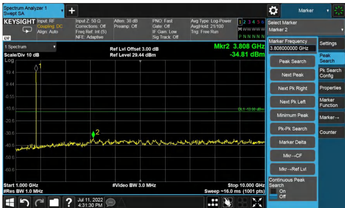
Band4-High Channel-15MHz Bandwidth-1GHz to 10GHz
