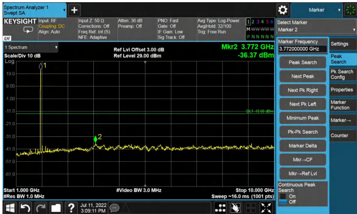
Band2-Low Channel-20MHz Bandwidth-1GHz to 10GHz
