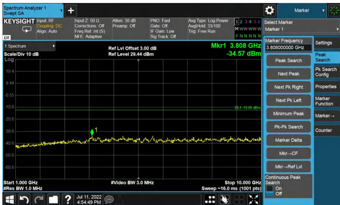
Middle Channel-1.4MHz Bandwidth-1GHz to 10GHz
