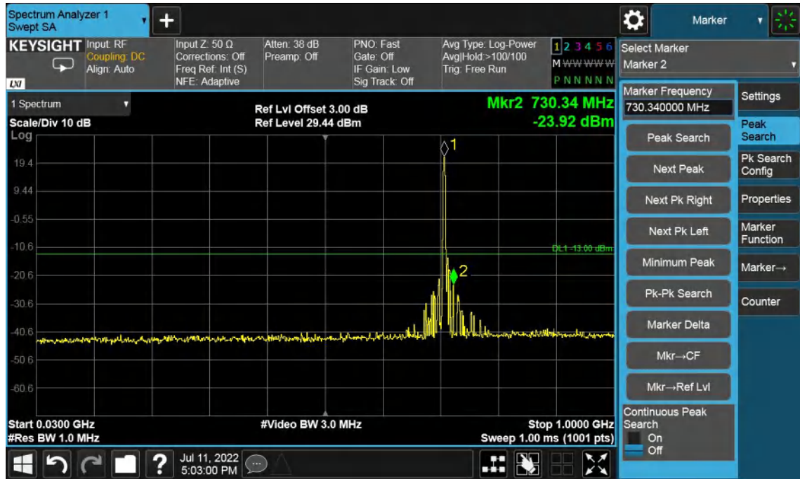
High Channel-1.4MHz Bandwidth-30MHz to 1GHz
