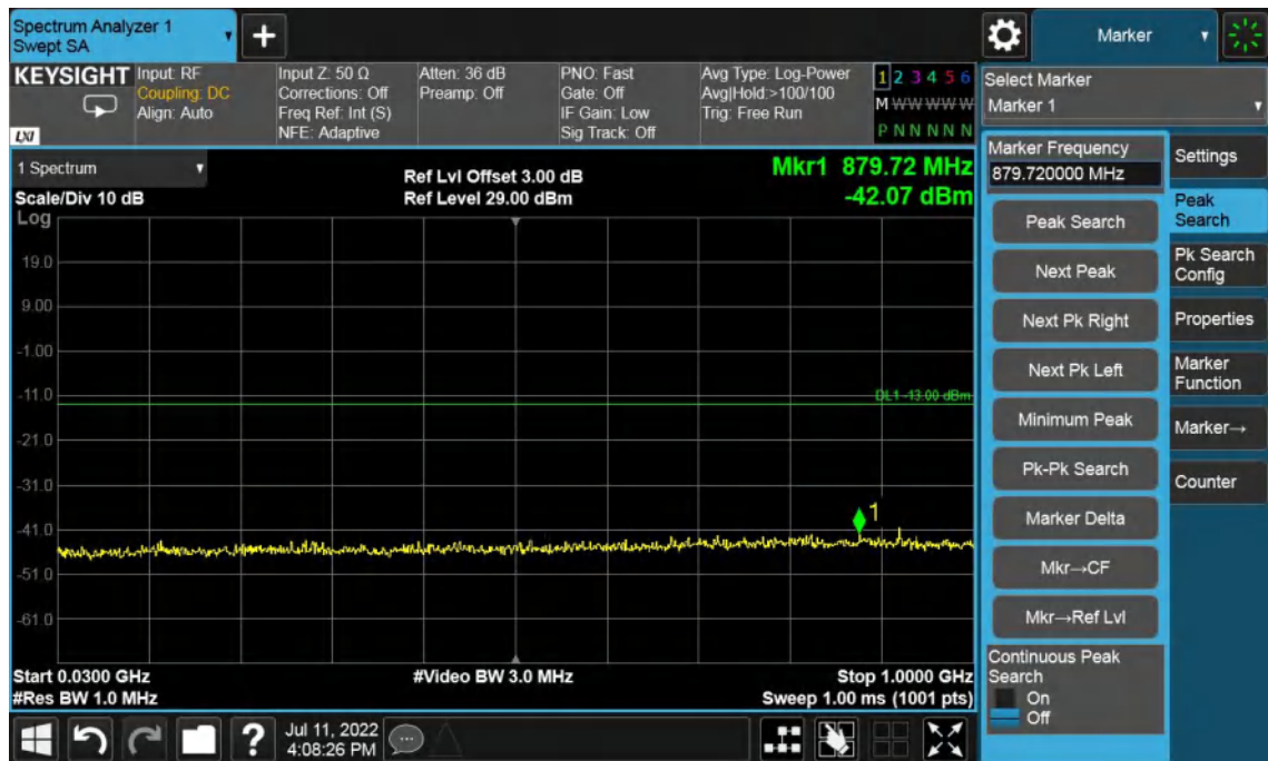
Band4-Middle Channel-1.4MHz Bandwidth-30MHz to 1GHz
