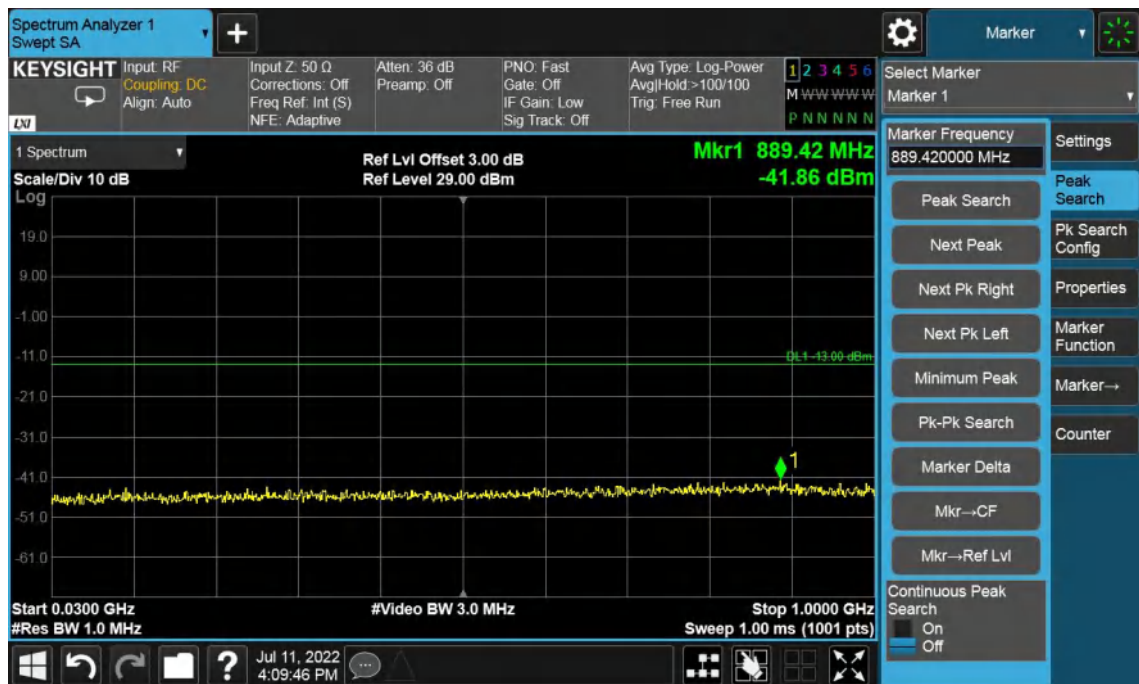
Band4-Middle Channel-3MHz Bandwidth-30MHz to 1GHz
