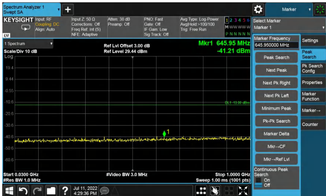
Band4-High Channel-10MHz Bandwidth-30MHz to 1GHz
