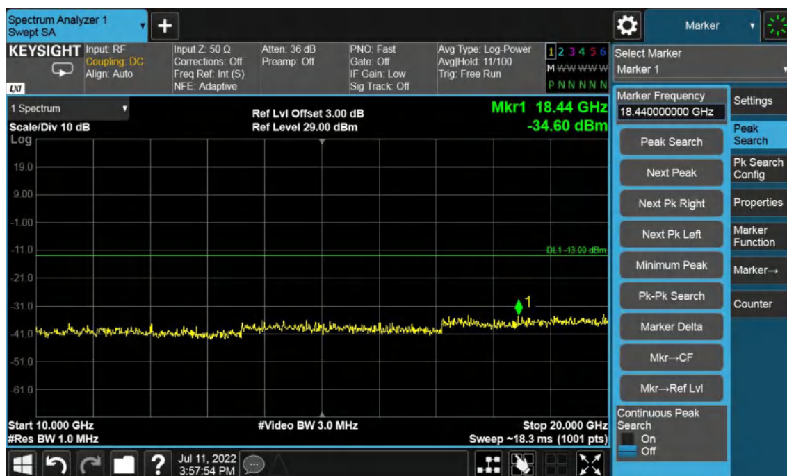
Band4-Low Channel-20MHz Bandwidth-10GHz to 20GHz
