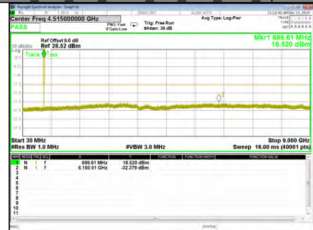
B12_15K_1#0_BPSK_BW_Mid_CDT_Spurious
