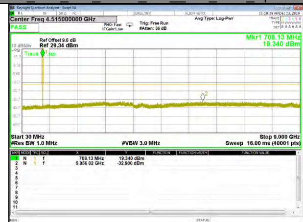
B12_15K_1#0_BPSK_BW_High_CDT_Spurious
