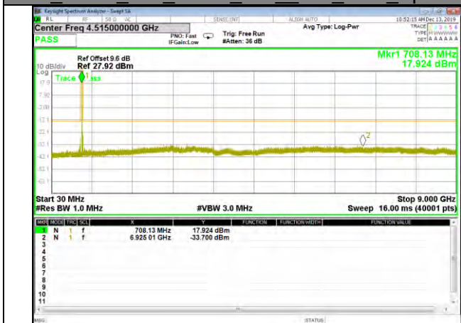
B12_3.75K_1#0_BPSK_BW_High_CDT_Spurious
