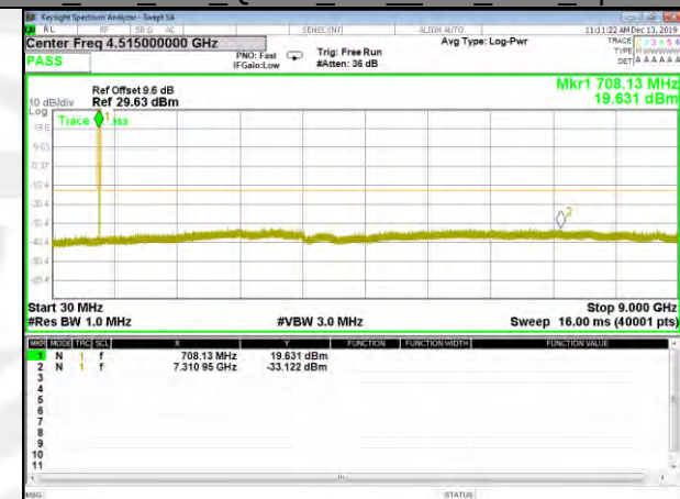
B12_15K_1#0_QPSK_BW_High_CDT_Spurious
