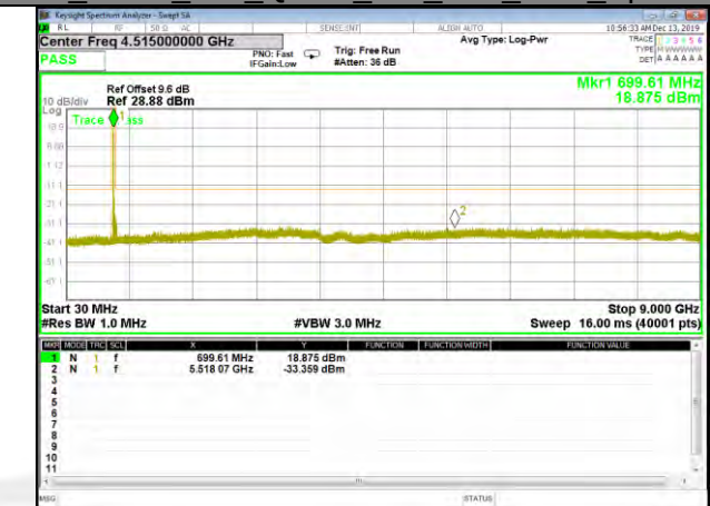
B12_3.75K_1#0_QPSK_BW_Mid_CDT_Spurious
