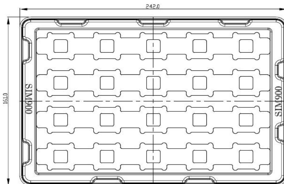
Figure 37: Tray drawing
