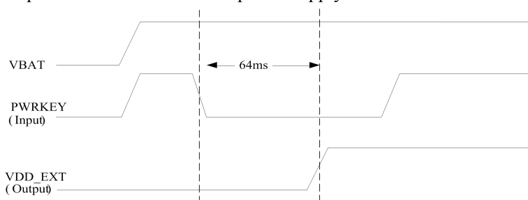
Figure 25: Power on sequence of the VDD_EXT
