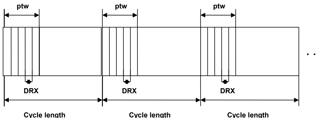
Figure 31: e-DRX diagrammatic sketch
