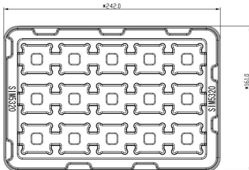
Figure 44: Tray drawing
