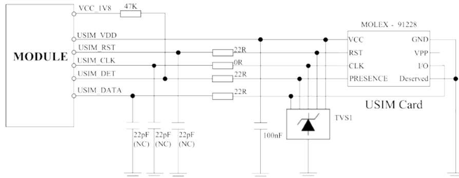
Figure 23: USIM interface reference circuit with USIM_DET
