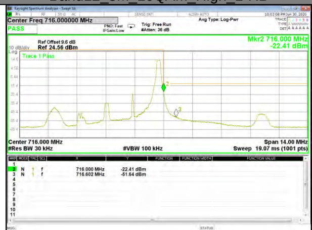
Band12_3M_16QAM_High_1-RB
