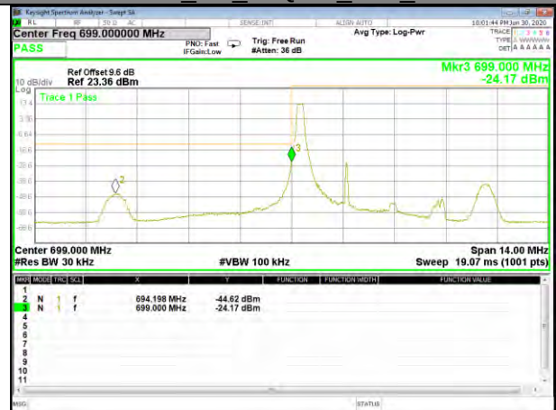
Band12_3M_16QAM_Low_Full-RB
