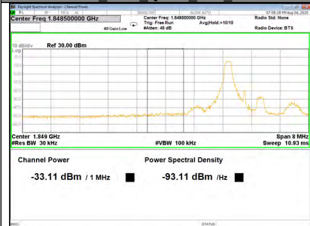
Band2_1.4M_QPSK_Low_Full-RB
