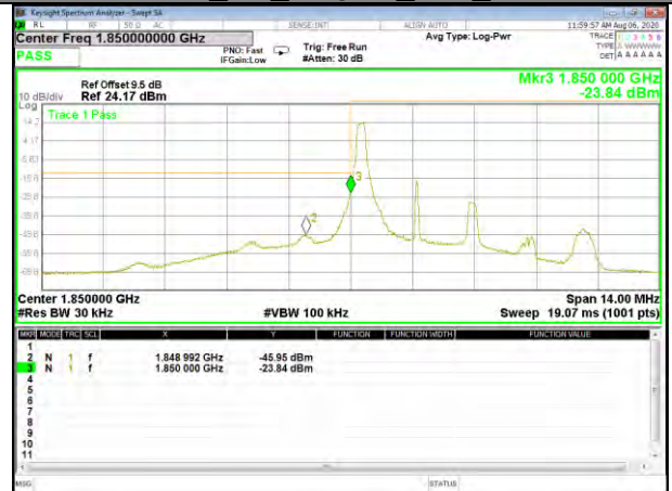
Band2_3M_16QAM_Low_Full-RB
