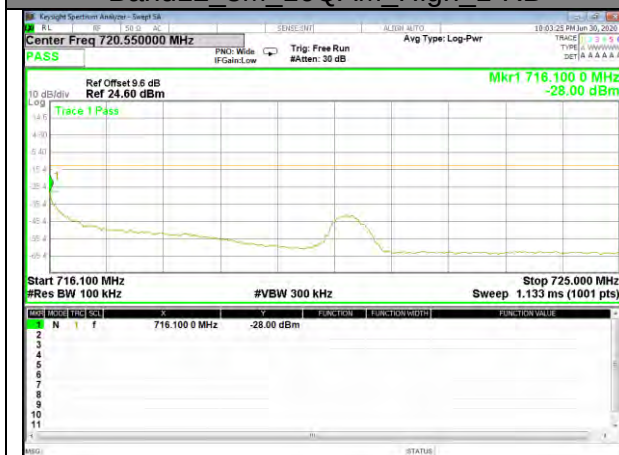
Band12_3M_16QAM_High_1-RB
