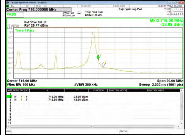
Band12_10M_QPSK_High_1-RB
