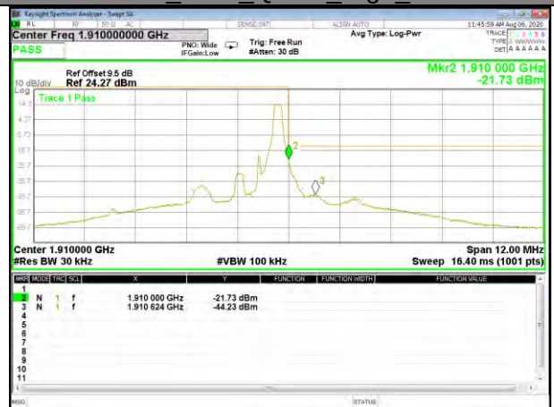
Band2_1.4M_QPSK_High_1-RB
