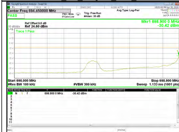
Band12_3M_16QAM_Low_Full-RB
