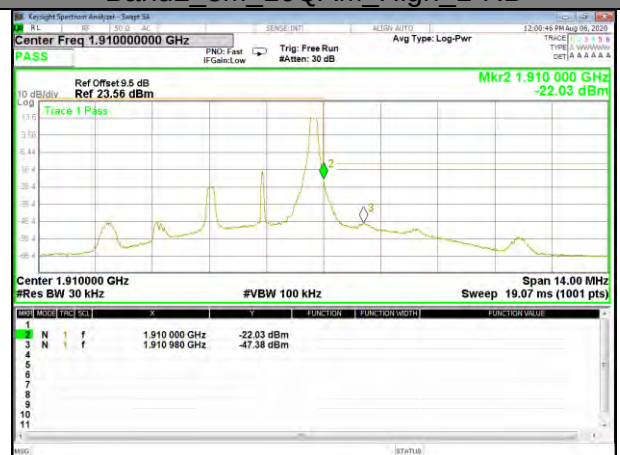
Band2_3M_16QAM_High_1-RB
