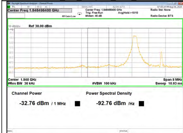
Band2_3M_16QAM_Low_Full-RB
