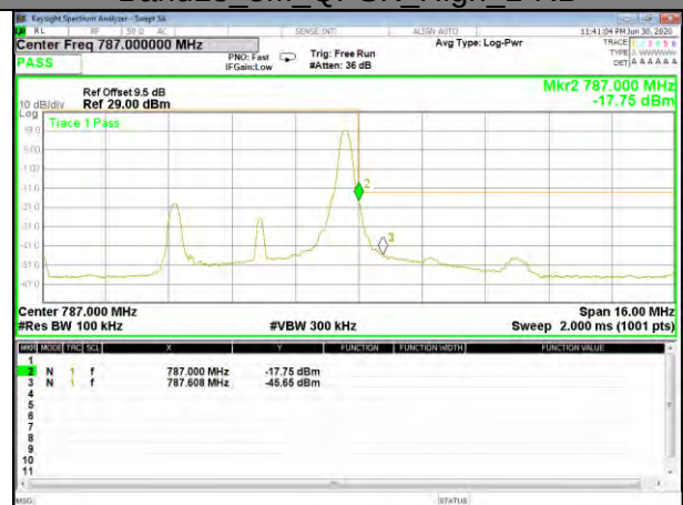
Band13_5M_QPSK_High_1-RB
