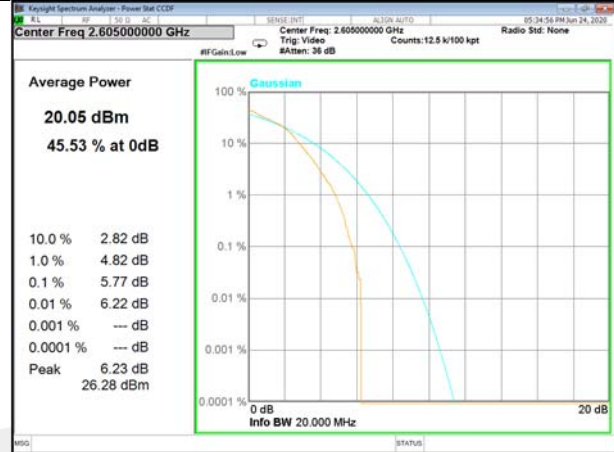
Band41_100_QPSK_High
