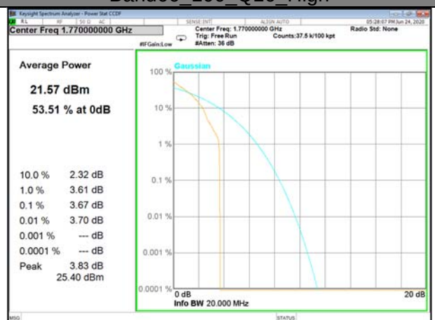
Band66_100_Q16_High
