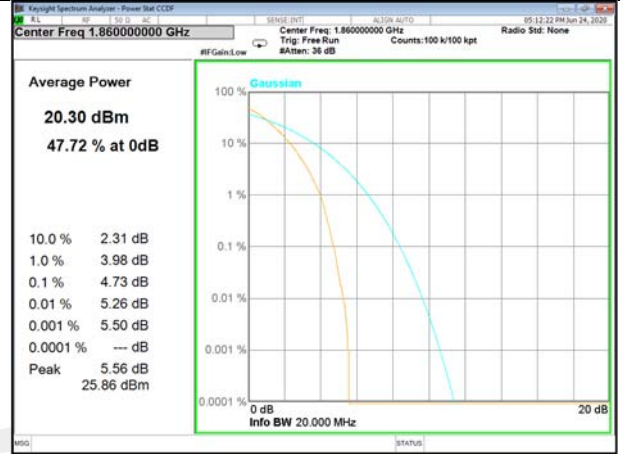
Band25_100_Q16_Low
