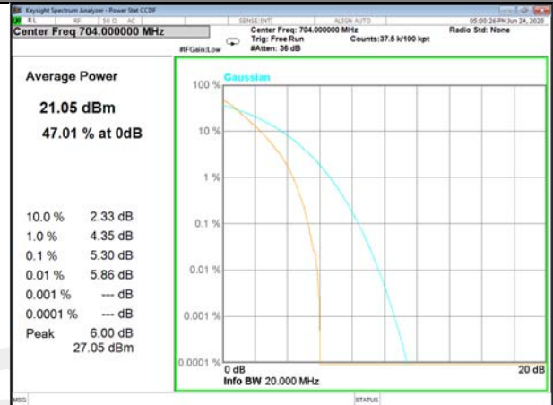
Band12_50_Q16_Low
