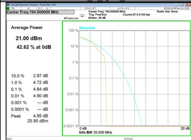
Band12_1_QPSK_Middle
