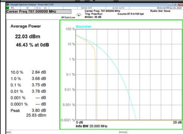
Band12_1_QPSK_Middle
