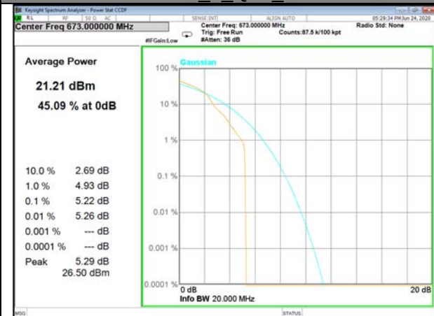
Band71_1_QPSK_Middle
