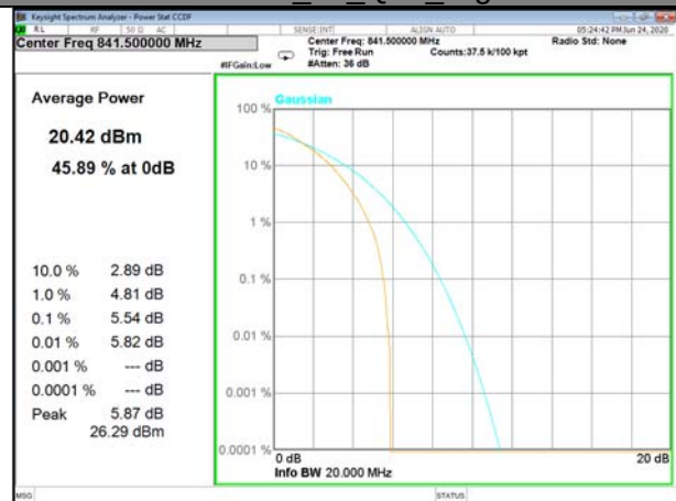
Band26_50_Q16_High
