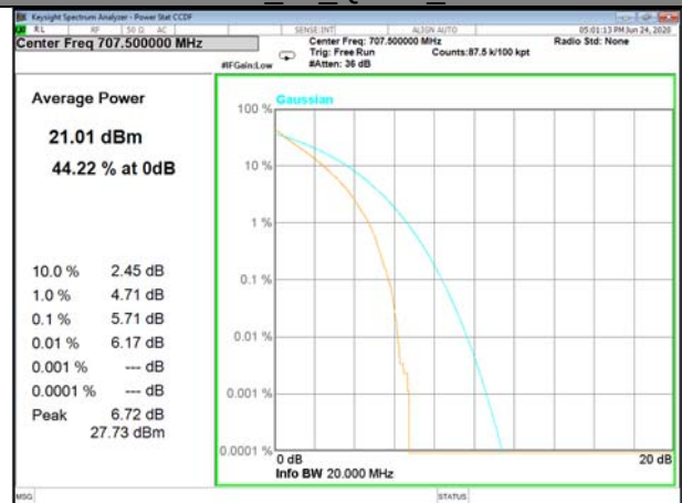
Band12_50_QPSK_Middle
