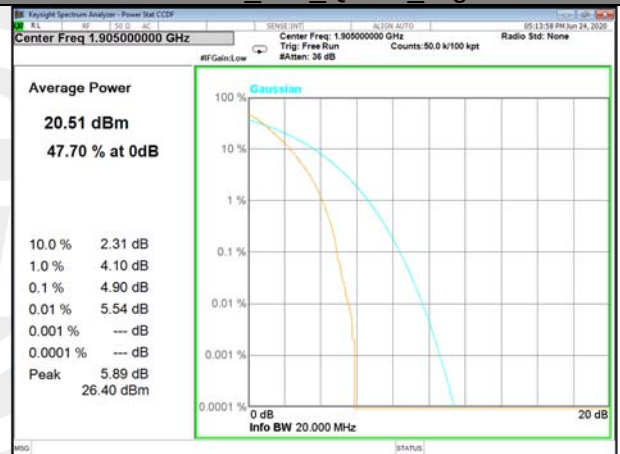
Band25_100_Q16_High
