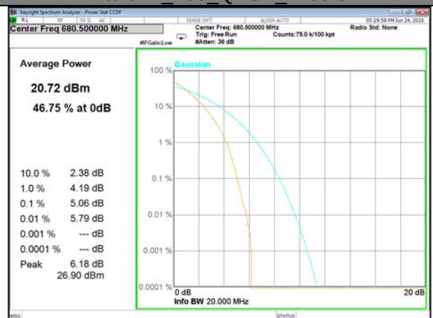
Band71_100_QPSK_Middle
