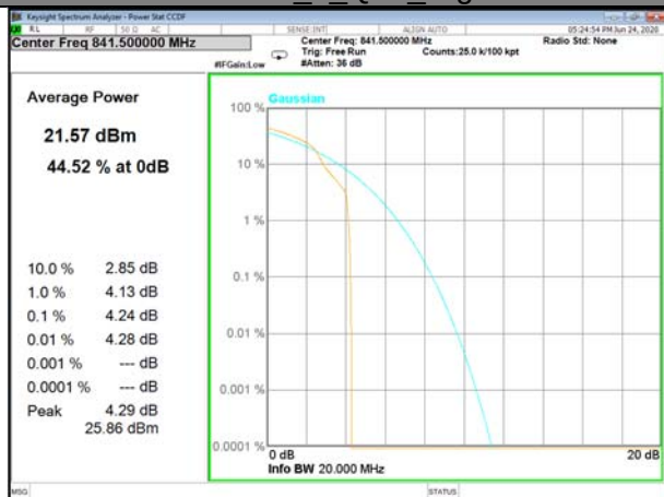
Band26_1_Q16_High
