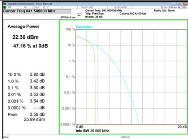
Band26_1_Q16_High
