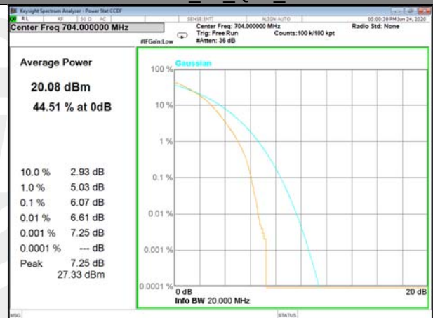
Band12_50_QPSK_Middle
