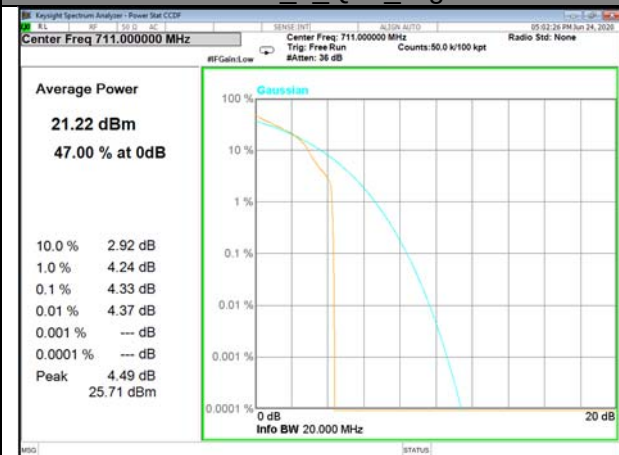
Band12_1_Q16_High
