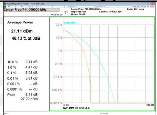
Band12_50_Q16_High
