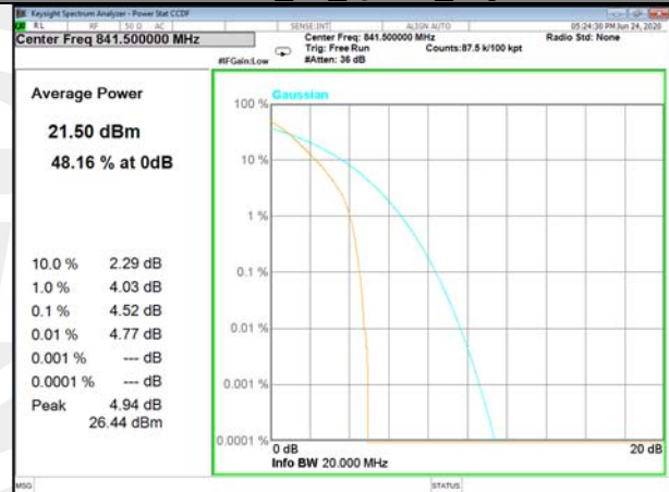
Band26_50_Q16_High
