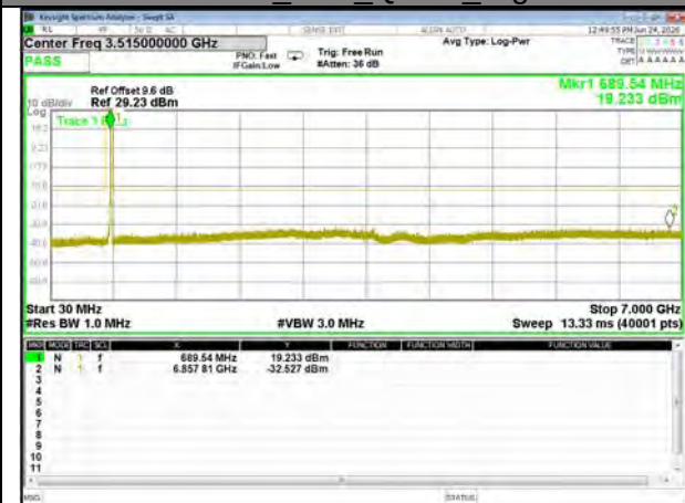
Band71_10M_QPSK_High
