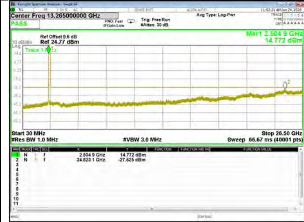
Band41_20M_QPSK_Middle
