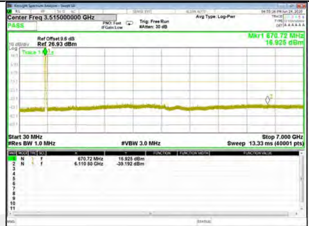
Band71_20M_16QAM_Middle
