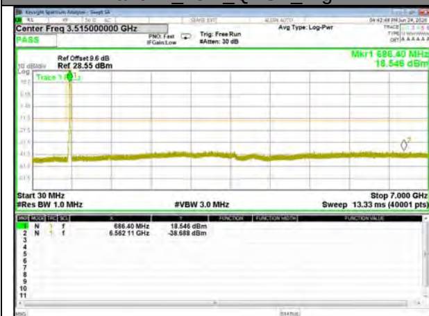
Band71_15M_QPSK_High
