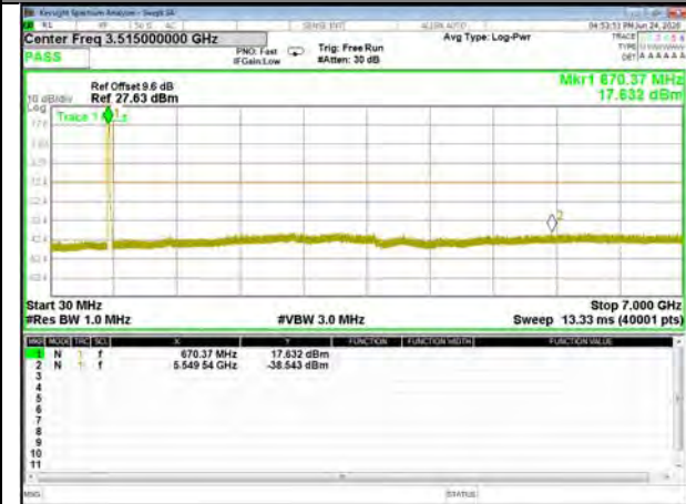
Band71_20M_QPSK_Middle
