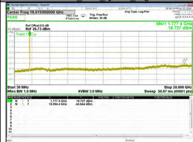
Band66_15M_QPSK_High
