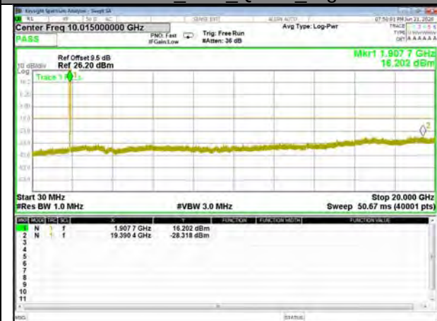
Band25_15M_QPSK_High
