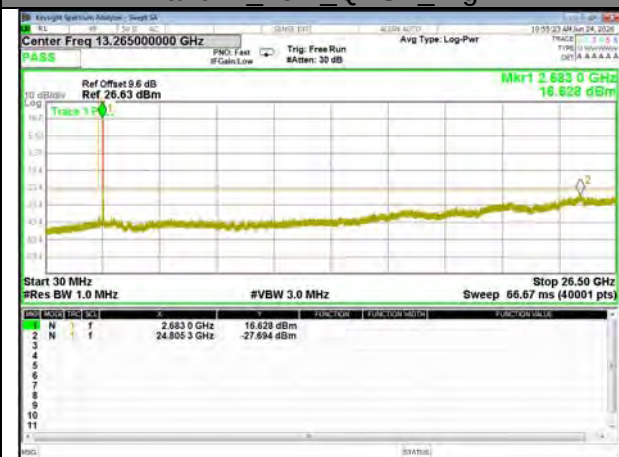
Band41_15M_QPSK_High
