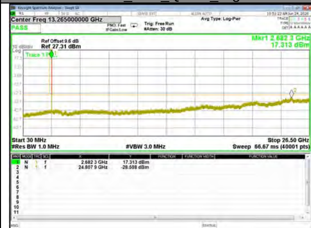
Band41_10M_QPSK_High
