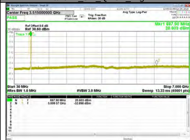
Band71_5M_QPSK_High
