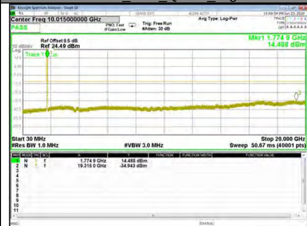
Band66_20M_QPSK_High
