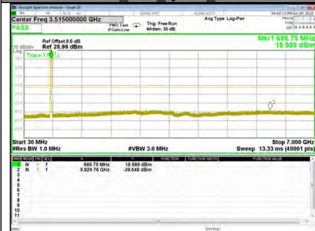
Band71_15M_QPSK_High
