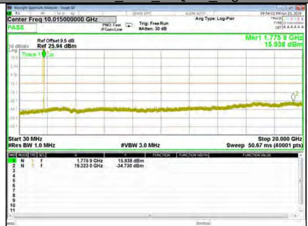
Band66_10M_16QAM_High
