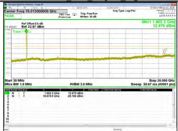
Band25_15M_16QAM_High
