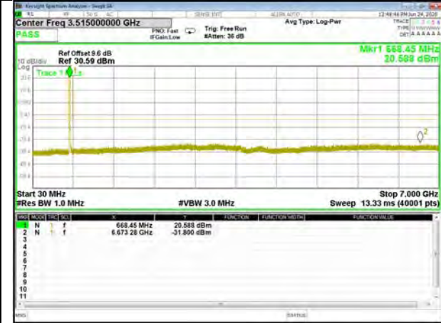
Band71_10M_QPSK_Middle
