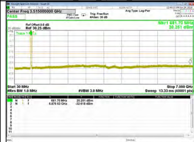
Band71_10M_QPSK_High
