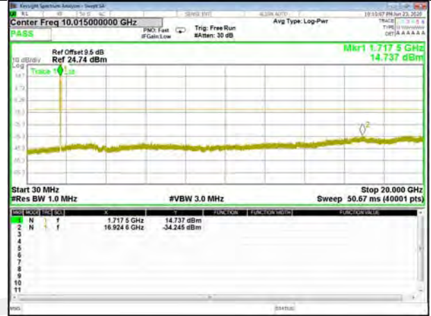
Band66_20M_16QAM_Middle
