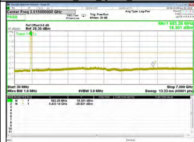
Band71_20M_QPSK_High
