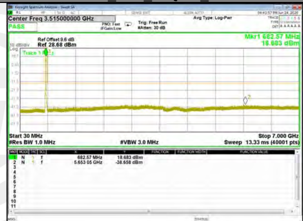
Band71_15M_16QAM_High
