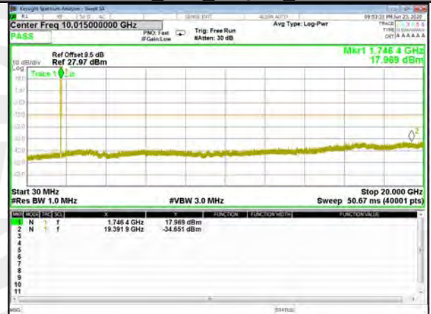
Band66_10M_16QAM_High
