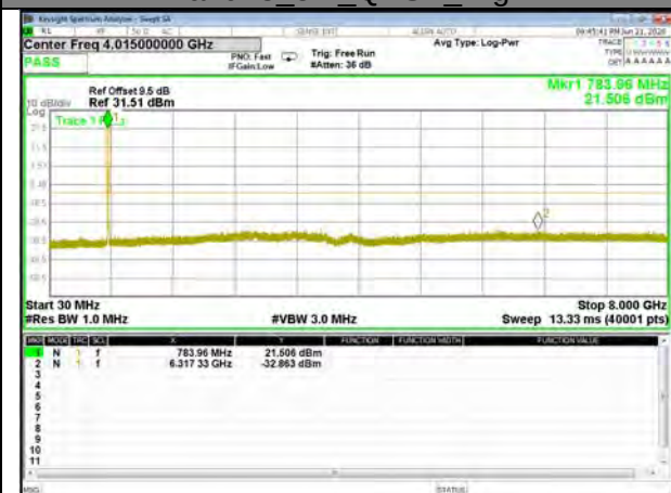
Band13_5M_QPSK_High
