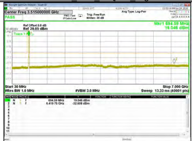
Band71_10M_16QAM_High
