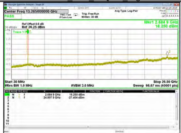
Band41_10M_16QAM_High
