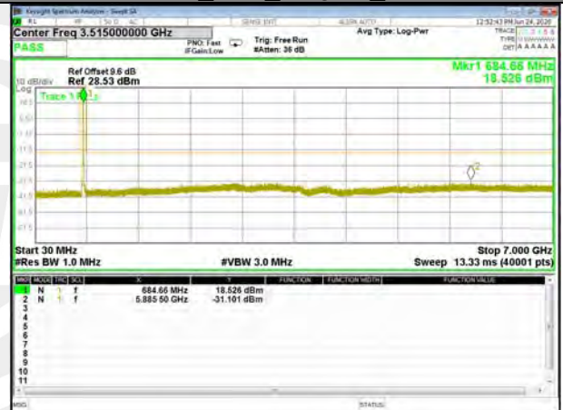
Band71_10M_16QAM_High
