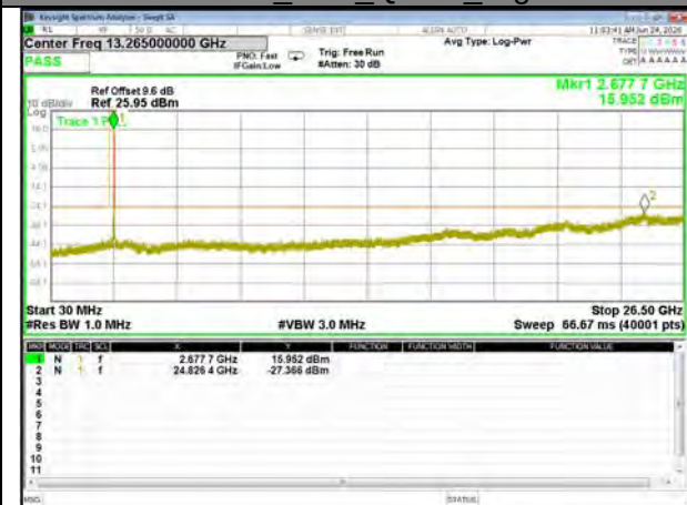
Band41_20M_QPSK_High
