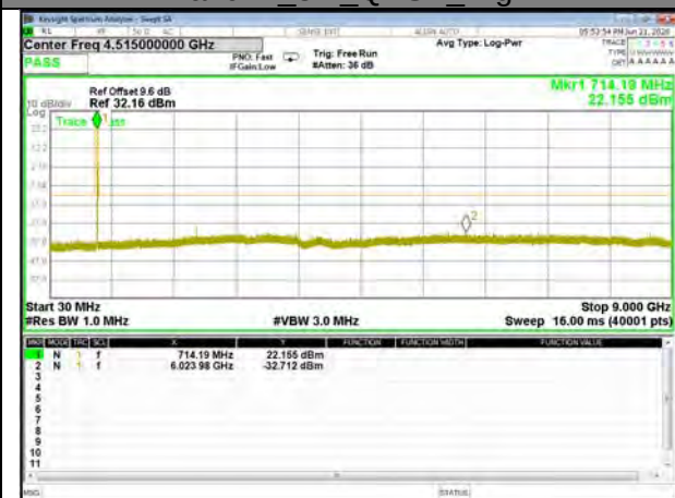
Band12_3M_QPSK_High
