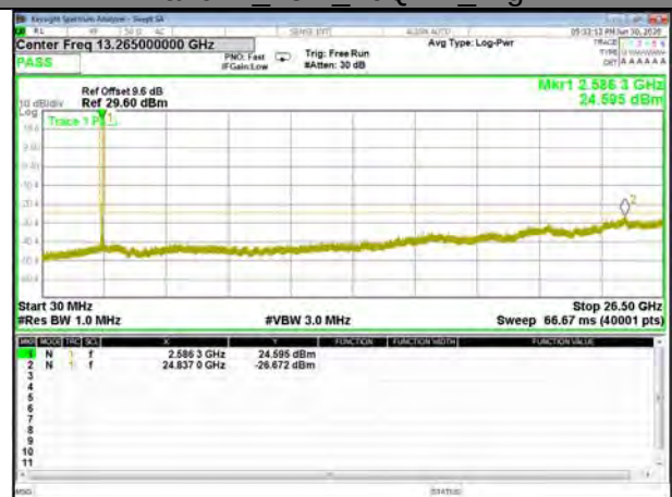
Band41_15M_16QAM_High
