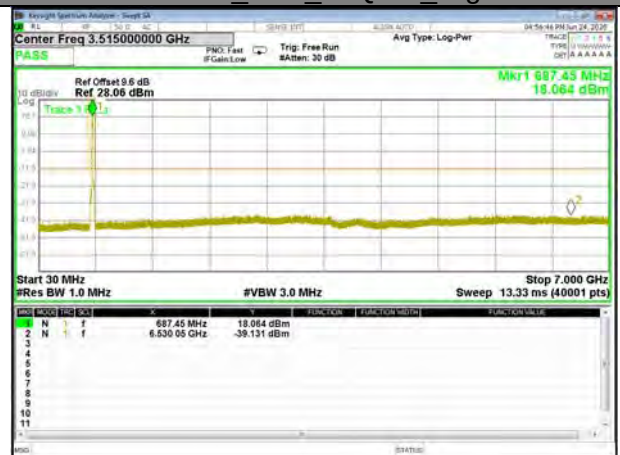
Band71_20M_16QAM_High
