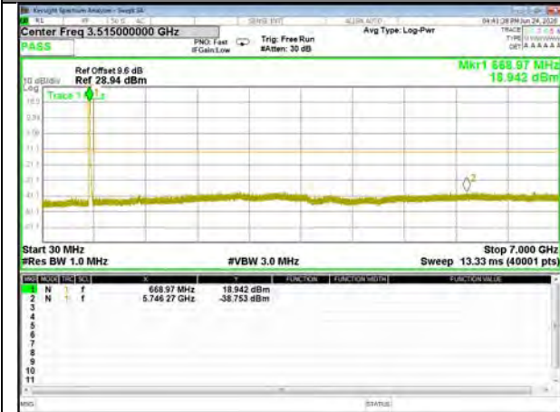
Band71_15M_QPSK_Middle
