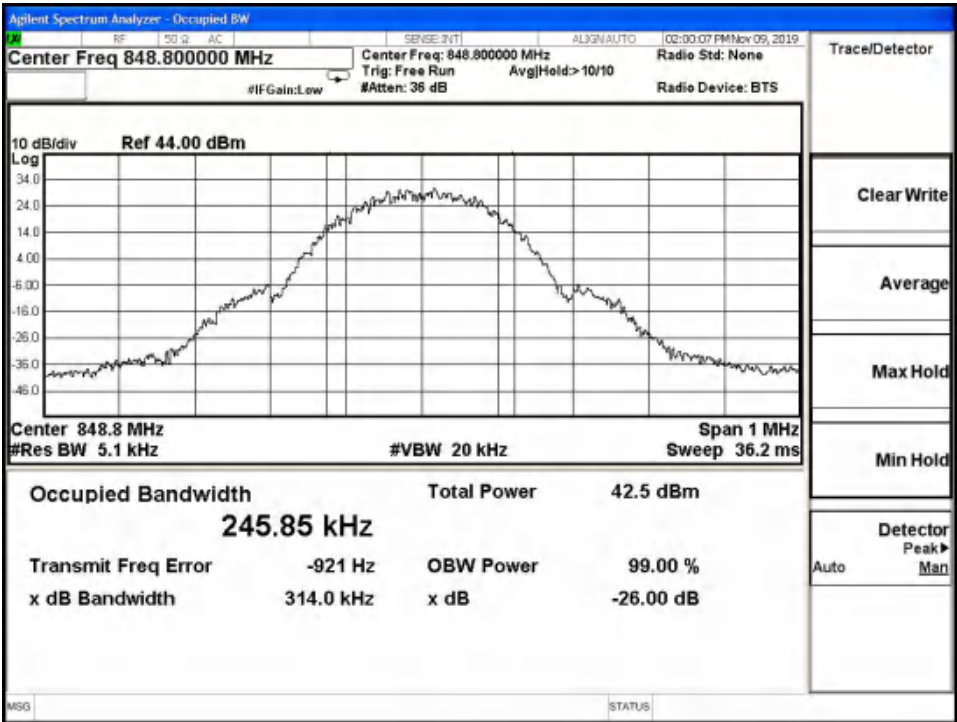
GMSK 99% Channel 251
