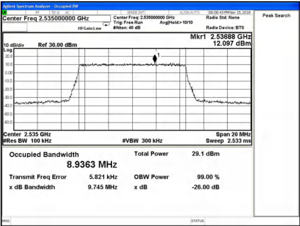
LTE Band7 QPSK 99% Channel 21100 BW=10MHz RB=50 RB Offset=0
