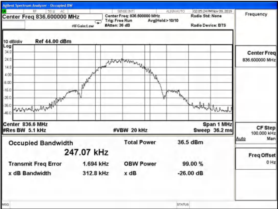
8PSK 99% Channel 190
