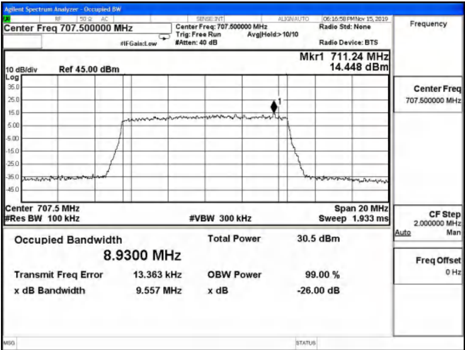
LTE Band12 QPSK -26dBc Channel 21625 BW=10MHz RB=50 RB Offset=0
