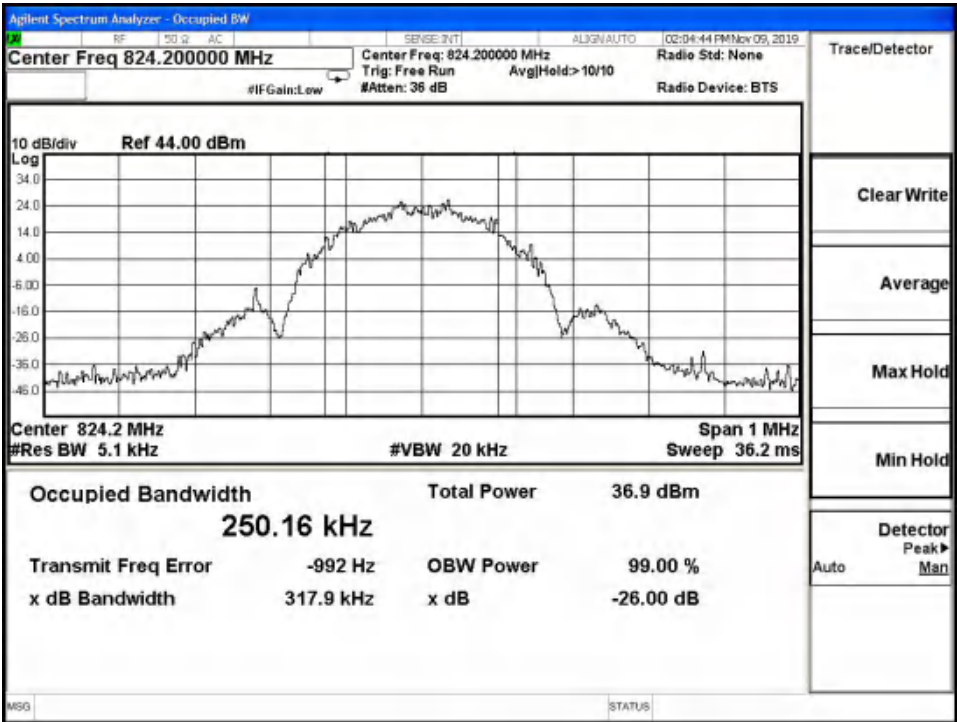
8PSK 99% Channel 128
