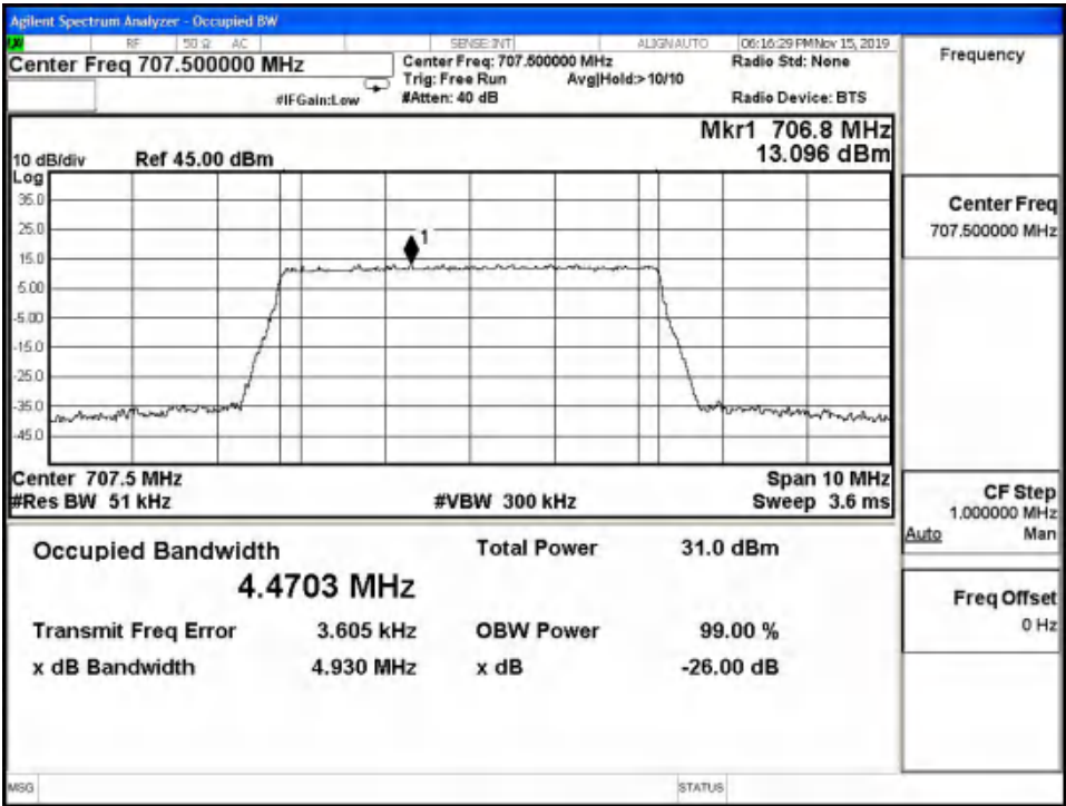
LTE Band12 QPSK -26dBc Channel 21625 BW=5MHz RB=25 RB Offset=0
