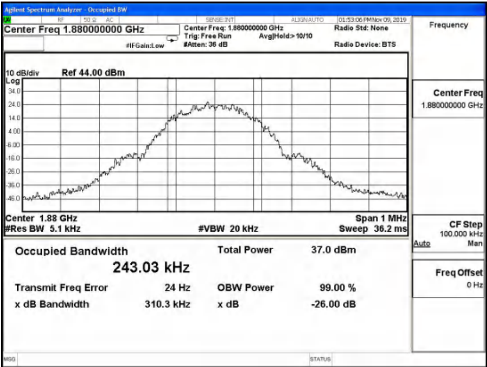
GMSK 99% Channel 661
