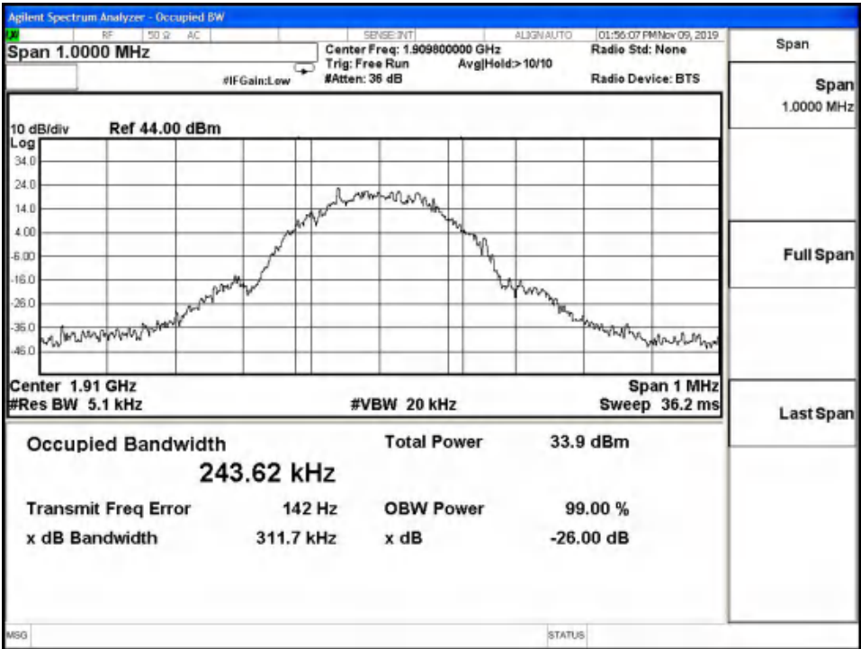
8PSK 99% Channel 810
