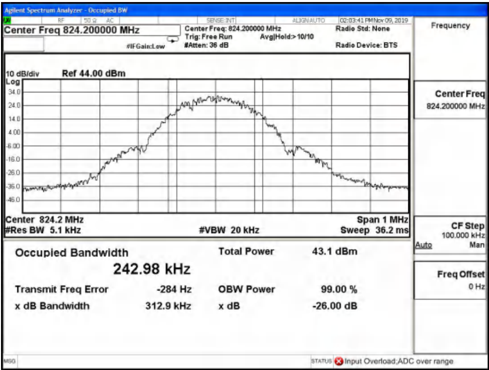
GMSK 99% Channel 128
