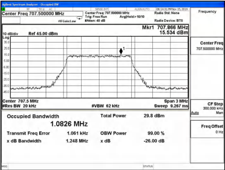
LTE Band12 16QAM 99% Channel 21625 BW=1.4MHz RB=6 RB Offset=0
