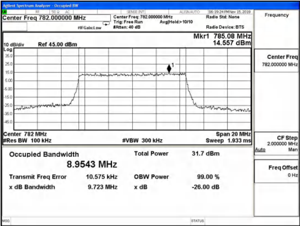
LTE Band13 16QAM -99% Channel 23230 BW=10MHz RB=50 RB Offset=0
