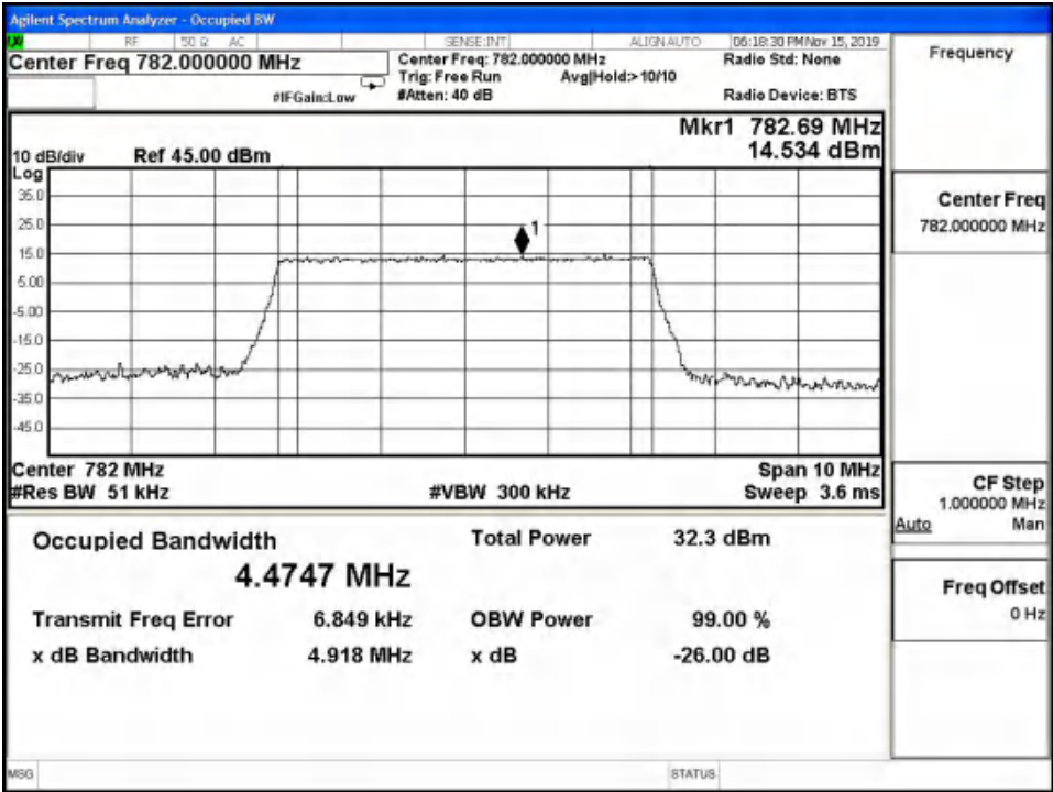
LTE Band13 16QAM 99% Channel 23230 BW=5MHz RB=25 RB Offset=0
