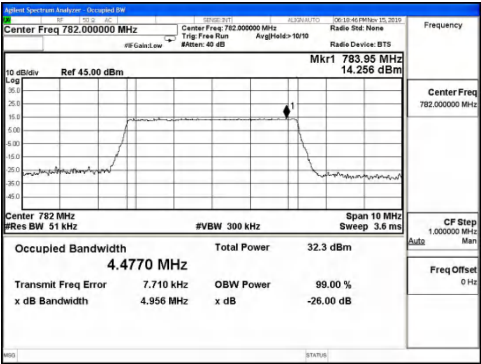
LTE Band13 QPSK -26dBc Channel 23230 BW=5MHz RB=25 RB Offset=0
