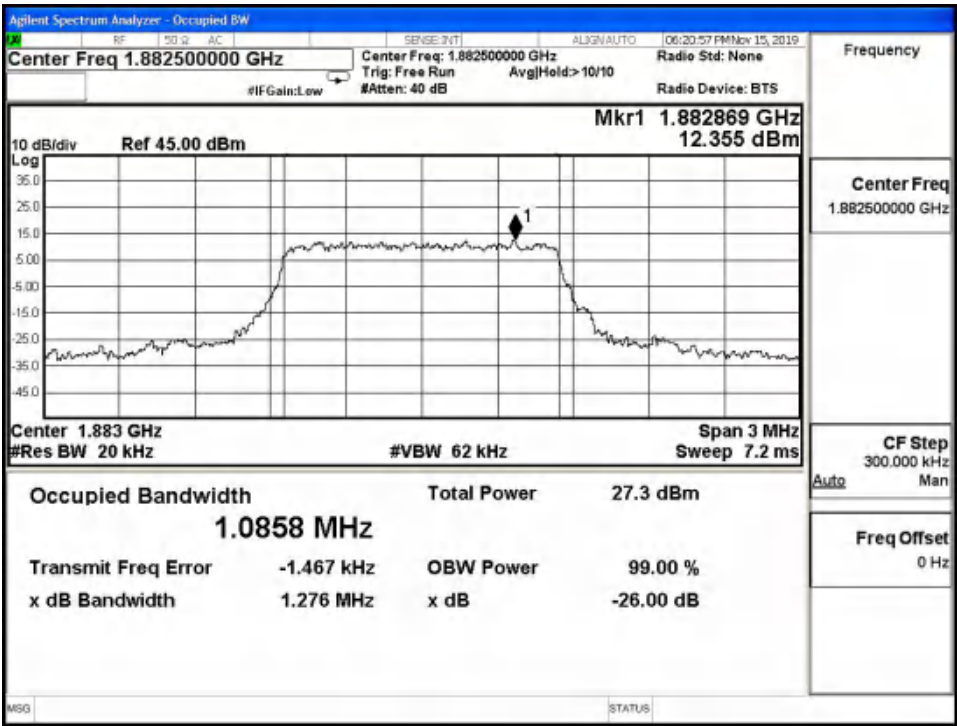
LTE Band25 QPSK 99% Channel 26365 BW=1.4MHz RB=6 RB Offset=0
