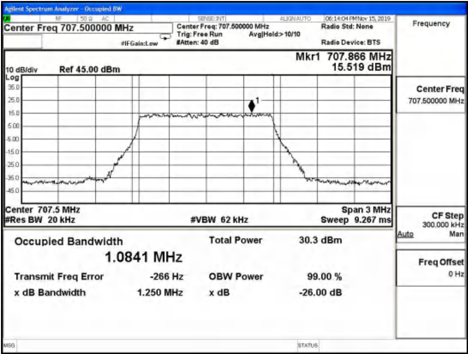
LTE Band12 QPSK 99% Channel 21625 BW=1.4MHz RB=6 RB Offset=0
