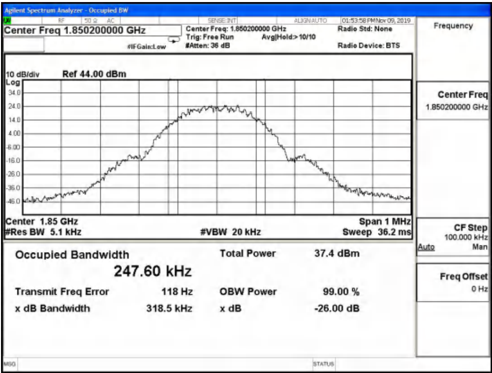
GMSK 99% Channel 512
