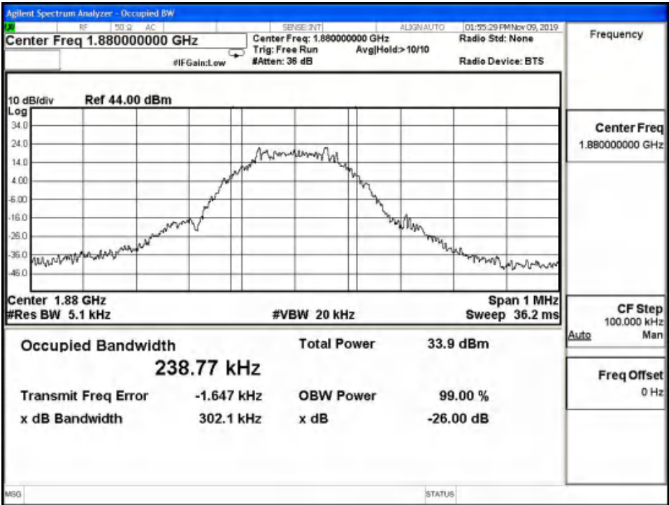
8PSK 99% Channel 661
