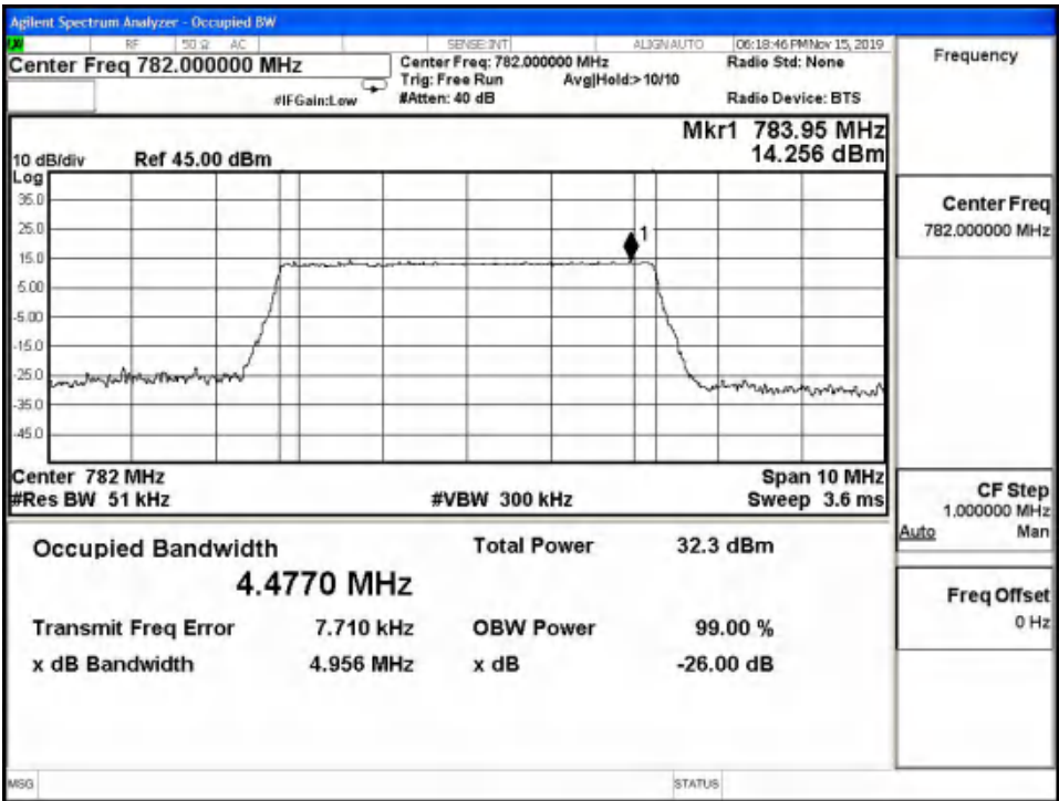
LTE Band13 QPSK 99% Channel 23230 BW=5MHz RB=25 RB Offset=0
