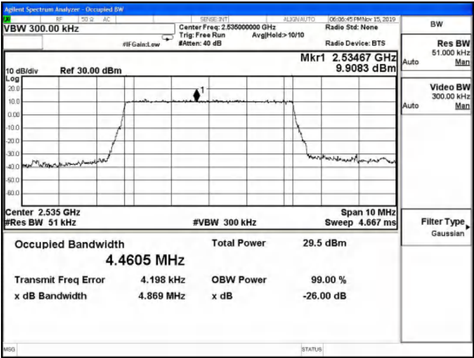
LTE Band7 QPSK -26dBc Channel 21100 BW=5MHz RB=25 RB Offset=0
