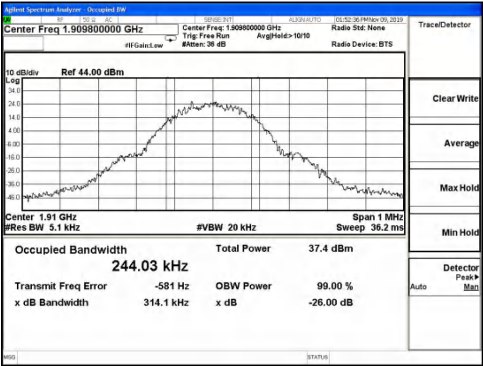
GMSK 99% Channel 810
