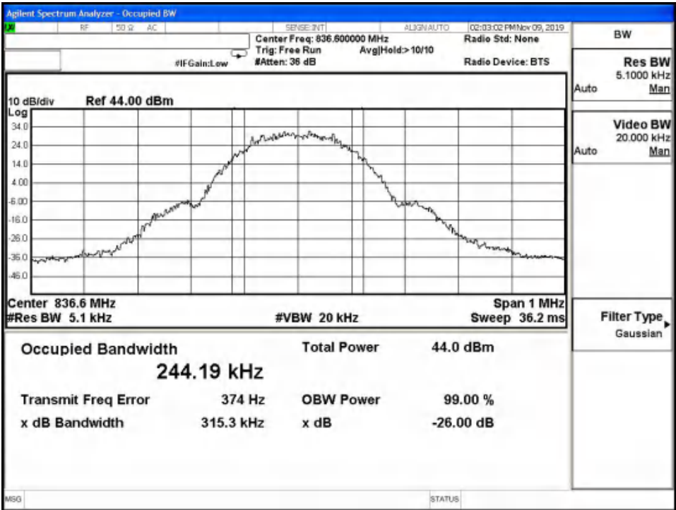
GMSK 99% Channel 190
