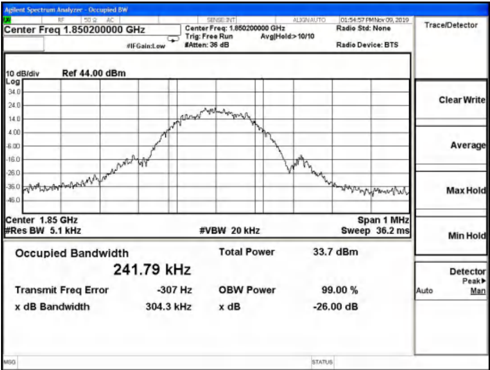
8PSK 99% Channel 512
