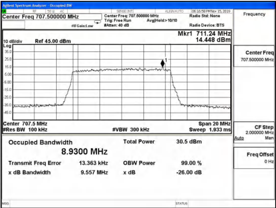
LTE Band12 QPSK 99% Channel 21625 BW=10MHz RB=50 RB Offset=0
