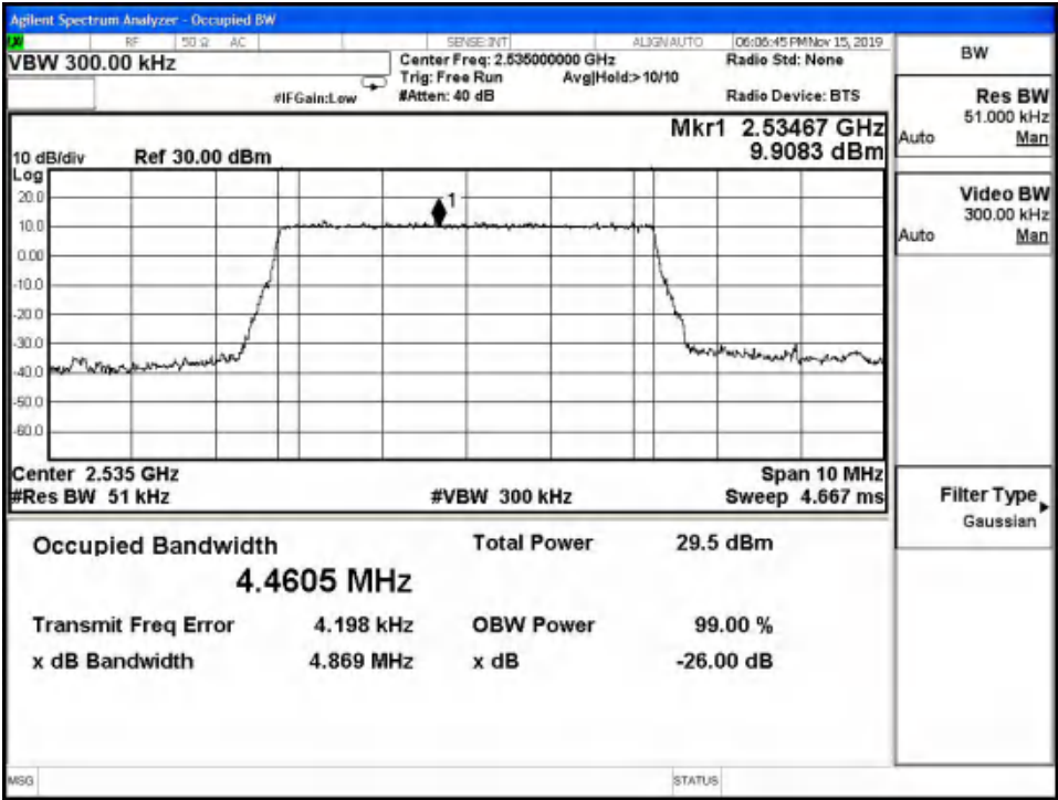
LTE Band7 QPSK 99% Channel 21100 BW=5MHz RB=25 RB Offset=0
