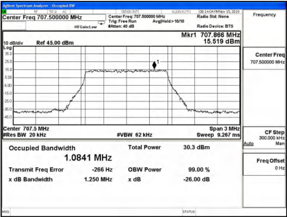
LTE Band12 QPSK -26dBc Channel 21625 BW=1.4MHz RB=6 RB Offset=0
