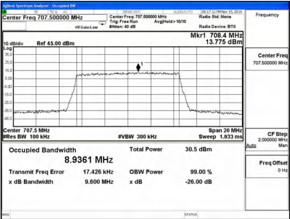
LTE Band12 16QAM -26dBc Channel 21625 BW=10MHz RB=50 RB Offset=0
